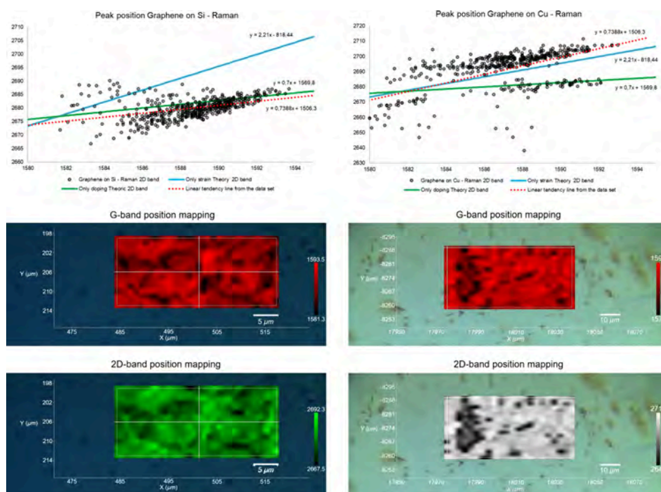
Figure 4. Correlation between G and 2D peak positions for graphene on Si (left column) and graphene on Cu (right column), together with spatial maps of the fitted peak positions. Top panels: scatter plots of the experimental data (black dots) compared with reference trends for strain-dominated (blue line) and doping-dominated (green line) regimes, along with the linear fit of the data sets (red dotted line). Middle panels: spatial distribution of the G band position extracted from peak fitting. Bottom panels: spatial distribution of the 2D band position extracted from peak fitting. The graphene on Si data set consists of 510 spectra acquired over a 34 \times 15 -point grid with 1 \mu\text{m} step size in both x and y directions. The graphene on Cu data set consists of 440 spectra acquired over a 22 \times 20 -point grid with 1 \mu\text{m} step size in both x and y directions.
