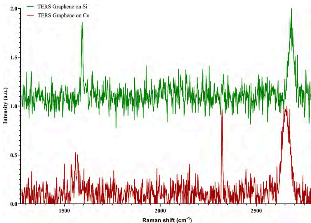
Figure 5. TERS spectra acquired on graphene on Si (green) and graphene on Cu (red), highlighting differences in near-field Raman response between the two substrates. The enhanced spectral features reflect local signal amplification at the tip–sample junction. A peak around \sim 2320 \text{cm}^{-1} is attributed to molecular \text{N}_2 from the ambient environment. Tip-in and tip-out comparisons are reported in Figures S2 and S3 (Supporting Information) together with the far-field in Figures S4 and S5 (Supporting Information).
