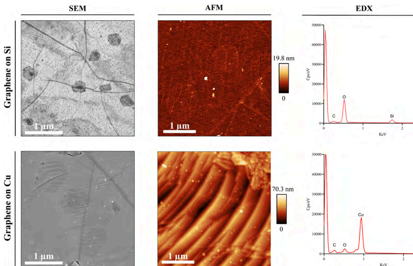
Figure 2. Graphene on Si (top row) and graphene on Cu (bottom row). For each sample, the first column shows representative SEM micrographs. The second column reports AFM topography maps (orange scale). The third column presents EDX spectra acquired from the investigated regions.
