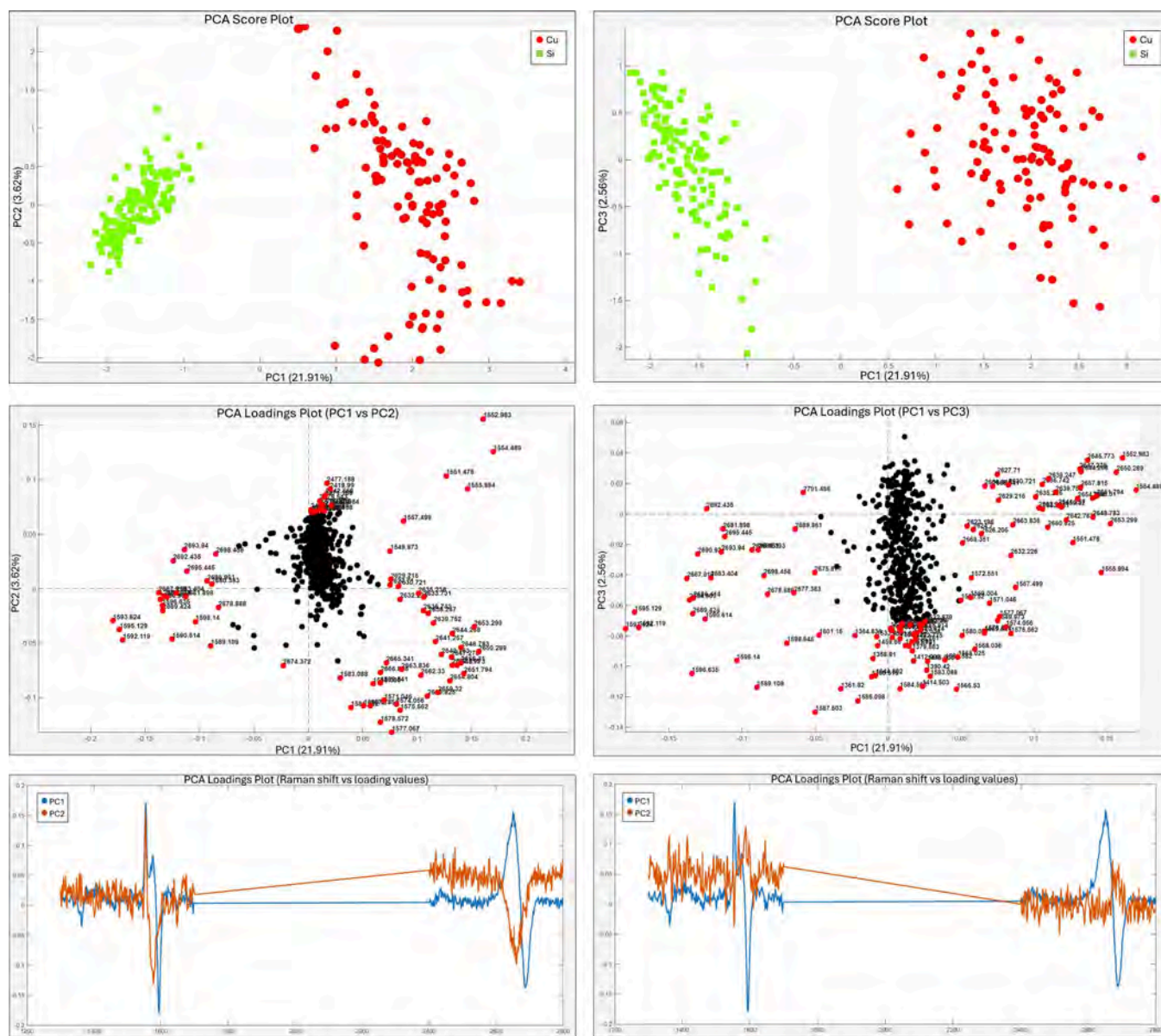
Figure 9. Principal component analysis (PCA) of the combined TERS data set acquired on graphene on Si and Cu. Score plots (PC1 vs PC2 and PC1 vs PC3, uppermost panels). The corresponding loadings plots are reported in the central panels. Each point in the loading plot corresponds to a Raman shift variable; points farther from the origin have a larger contribution to the corresponding principal components. Red points are used only as a visual guide to highlight the Raman-shift variables that appear farther from the origin in the loading space, while black points indicate the remaining variables. No quantitative threshold or independent color scale was applied for this graphical highlighting. The bottommost panels show the PC loading values as a function of the Raman shift ( \text{cm}^{-1} ). Compared to Raman, the distribution is significantly broader, particularly for graphene on Cu, indicating increased variability.
