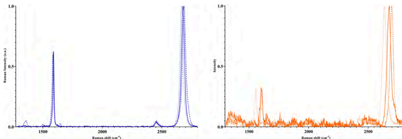
Figure 3. Raman spectra of graphene on Si (blue, left) and graphene on Cu (orange, right). For each sample, three spectra (solid, dashed, and dotted) are reported with visible shifts in the G-band and 2D band positions across different measurement points.
