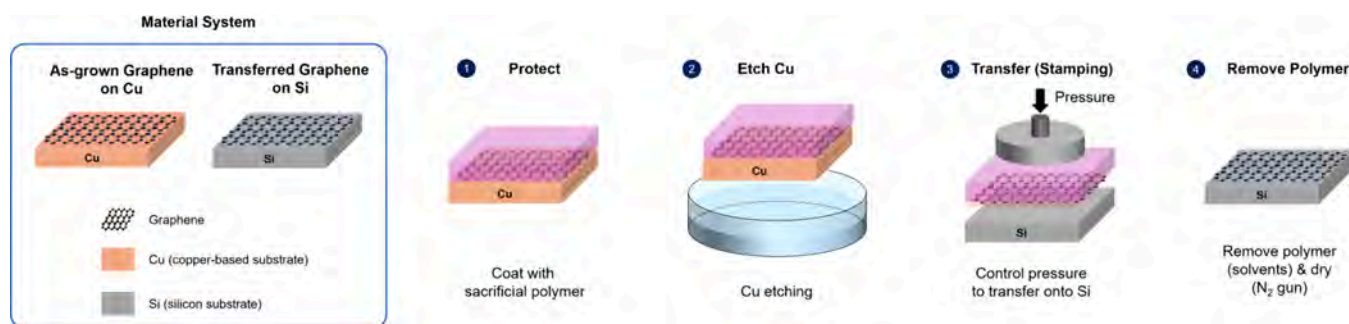
Figure 1. Schematic illustration of the monolayer graphene systems investigated in this work and of the semidry transfer process from Cu-based growth substrates to Si substrates. The scheme summarizes sacrificial polymer protection, Cu etching, pressure-assisted transfer onto Si, and final polymer removal.
