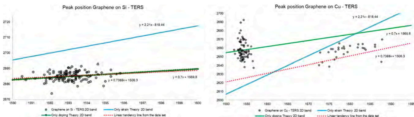
Figure 6. Correlation between G and 2D peak positions from TERS measurements for graphene on Si (left) and graphene on Cu (right). Experimental data (black dots) are compared with reference trends for strain-dominated (blue line) and doping-dominated (green line) regimes, together with the linear fit of the data sets (red dotted line).
