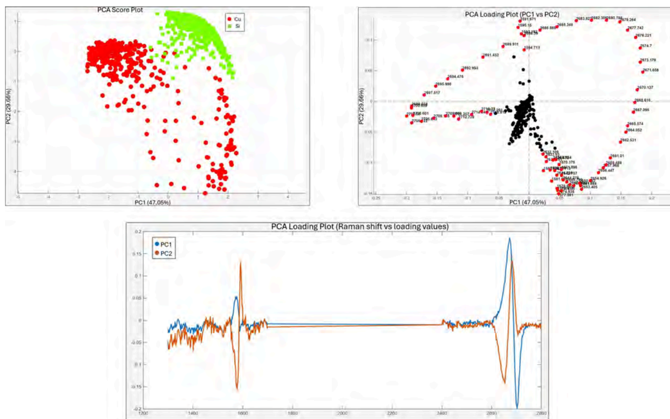
Figure 7. Principal component analysis (PCA) of the combined Raman data set acquired on graphene on Si and Cu. The score plot (PC1 vs PC2; upper-left panel). The corresponding loadings plots (reported in the upper-right and bottom panels) show the contribution of the different wavenumbers in the definition of the components. Each point in the loading plot corresponds to a Raman shift variable; points farther from the origin have a larger contribution to the corresponding principal components. Red points are used only as a visual guide to highlight the Raman-shift variables that appear farther from the origin in the loading space, while black points indicate the remaining variables. No quantitative threshold or independent color scale was applied for this graphical highlighting. In particular, the bottom panel reports the PC1 (blue) and PC2 (orange) loading values as a function of the Raman shift ( \text{cm}^{-1} ). PCA performed separately on each data set does not show distinct clustering for graphene on Si (see Supplementary Figures S6–S7 ).
