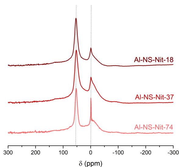
Fig. 5 ^{27}\text{Al} ssNMR spectra of aluminosilicate samples with various Si/Al ratios. The dotted lines are indicative of the position of the major contributions.
