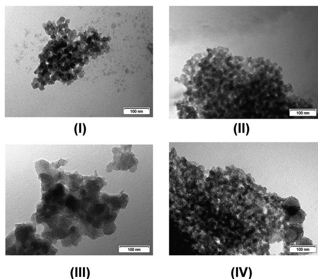
Fig. 2 TEM images of aluminosilicate nanospheres synthesized with different precursors. (I) Al-NS-Nit, (II) Al-NS-Cl, (III) Al-NS-Iso and (IV) Al-NS-Nit-a.
