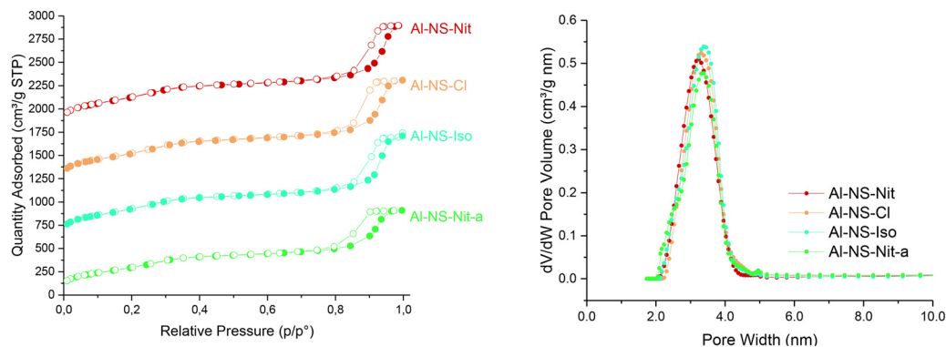
Fig. 3 N_2 physisorption adsorption-desorption isotherm (left) and DFT pore size distribution (right) of four aluminosilicate nanospheres synthesized with various Al sources. The isotherms of Al-NS-Iso, Al-NS-Cl, and Al-NS-Nit were incremented by 600, 1200 and 1800 \text{cm}^3 \text{g}^{-1} , respectively, for clarity.
