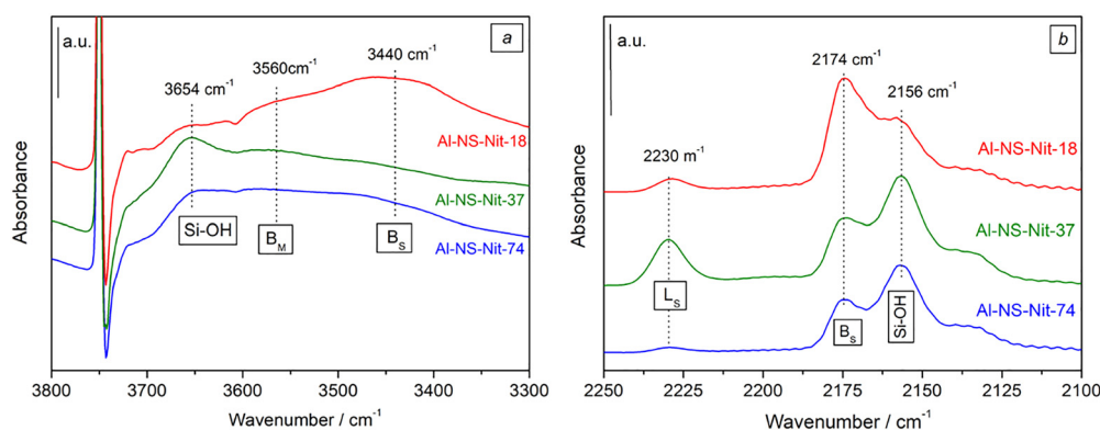
Fig. 7 Normalized IR difference spectra at equal equilibrium pressure (0.1 mbar) of CO at 77 K on Al-NS-Nit-74, Al-NS-Nit-37, and Al-NS-Nit-18 in the high (a) and low frequency region (b). Labels: L_s : strong Lewis, B_S : strong Brønsted, B_M : medium Brønsted.
