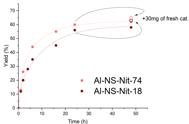
Fig. 8 Kinetic investigations conducted on Al-NS-Nit-74 and Al-NS-Nit-18 for the catalytic conversion of glycerol to solketal. Reaction conditions: glycerol:acetone = 1:4, 30 mg of catalyst, 50 °C, 800 rpm, solvent-free. Each point corresponds to one separate catalytic test performed with the same batch of materials. Dotted curves are for eye guidance only.
