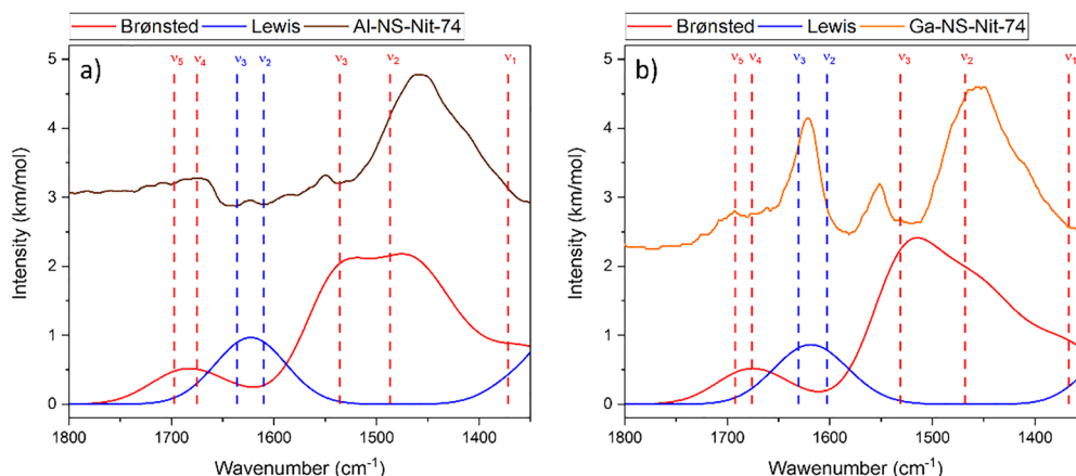
Fig. 10 Comparison between simulated IR spectra of ammonia interacting with Brønsted (red) and Lewis (blue) acid sites in (a) aluminosilicates and (b) gallosilicates, and experimental spectra (brown for aluminosilicates, yellow for gallosilicates). The mean frequency values for each vibrational mode are represented by vertical dashed lines.
