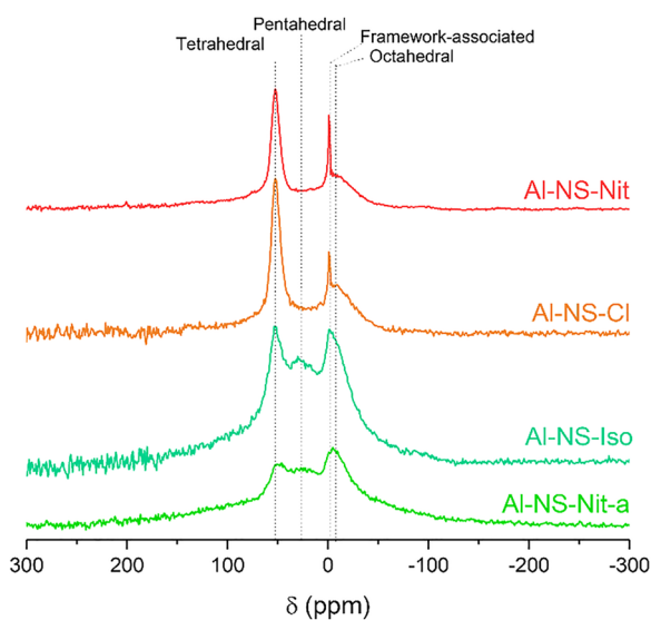
Fig. 4 ^{27}\text{Al} solid-state NMR spectra of aluminosilicate nanospheres using different Al sources.
