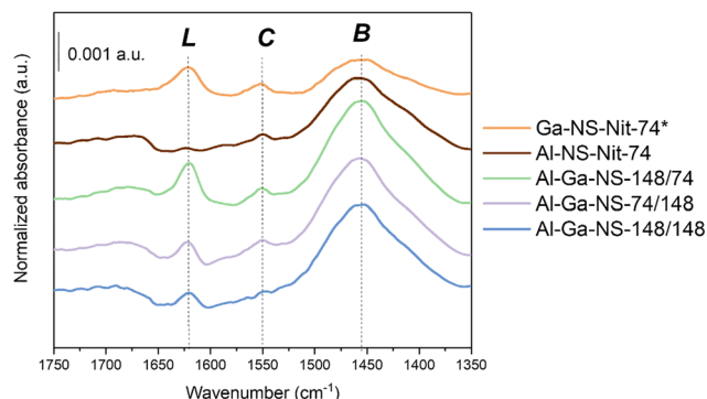
Fig. 9 Difference and normalized FT-IR spectra of ammonia dosages on bi-functional aluminosilicate and gallosilicate nanospheres after ammonia dosages and prolonged outgassing at RT. (L: Lewis, B: Brønsted, H: H-bonded, C: Chemisorbed ammonia). *The spectrum of Ga-NS-Nit-74 was previously reported by our group. 22
