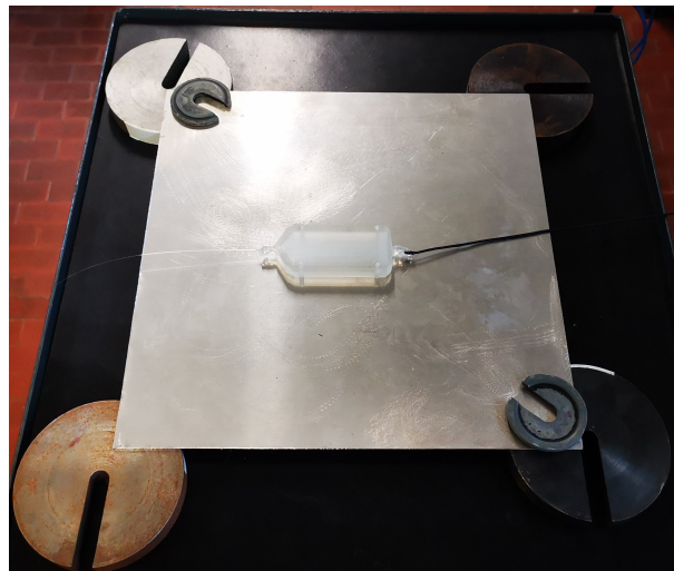
Figure 3: Experimental setup for impulse-based testing of the blade
