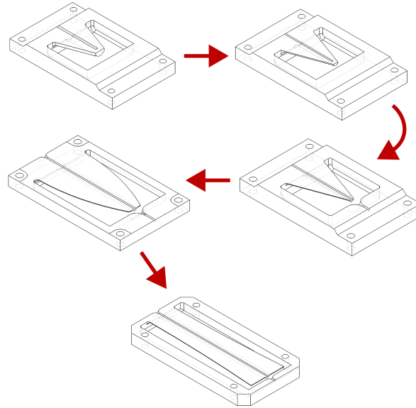
Figure 1: Evolution of the internal cross-section of the sensing element.
