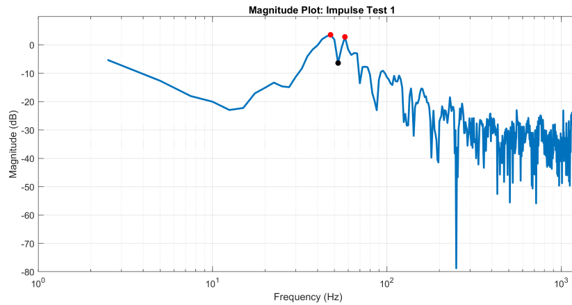
Figure 4: Power spectrum for the impulse test response
