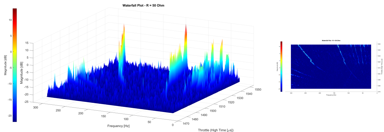
Figure 5: Power spectra for different throttle settings shown in 3D on the left and in 2D on the right
