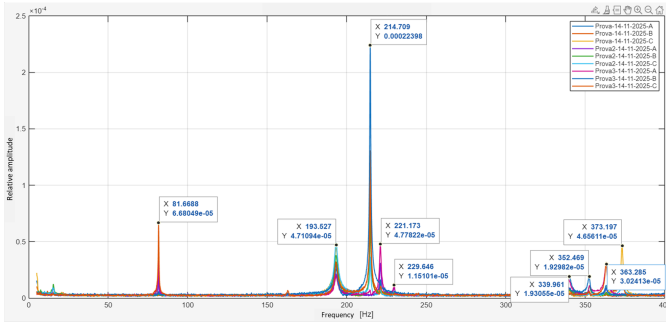
Fig. 6. Spectrum obtained from the FBG .
