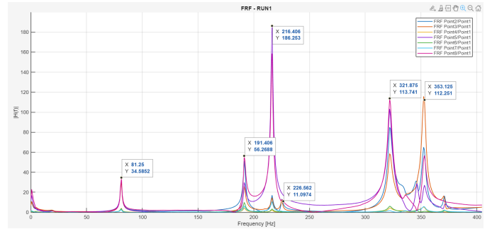
Fig. 4. Spectrum obtained from the piezoelectric instrumentation.
