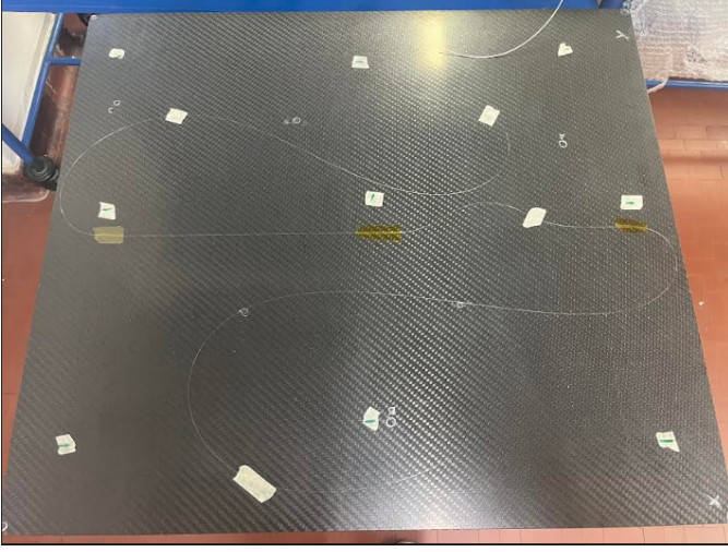
Fig. 2. Plate instrumented with the optical sensor network
