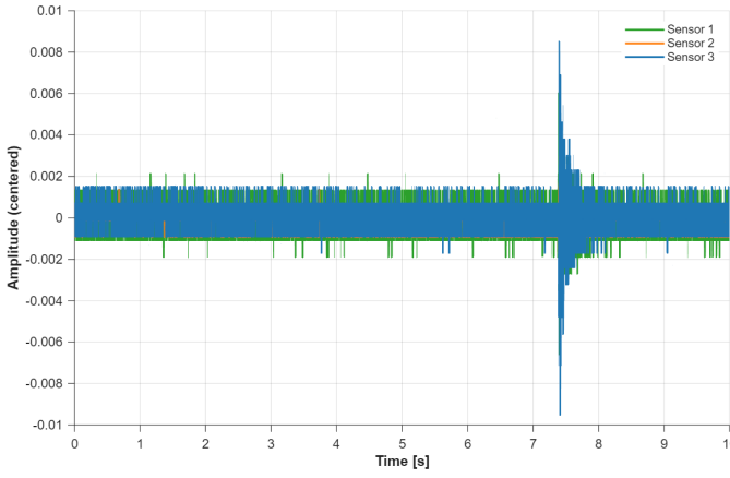
Fig. 5. Example of FBG raw data during an Hammer test.
