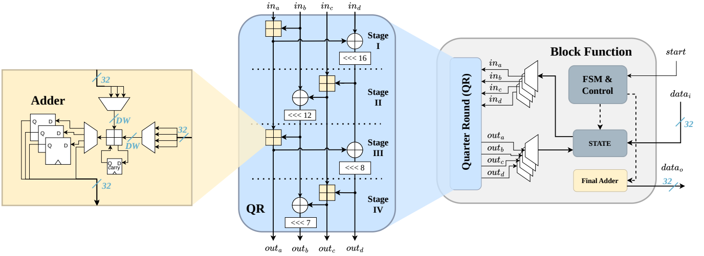
Fig. 2. Hierarchical hardware architecture of the ChaCha core, illustrating a top-down drill-down from the system level to individual arithmetic components.
