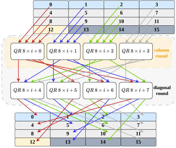
Fig. 1. Composition of column and diagonal rounds in ChaCha.
