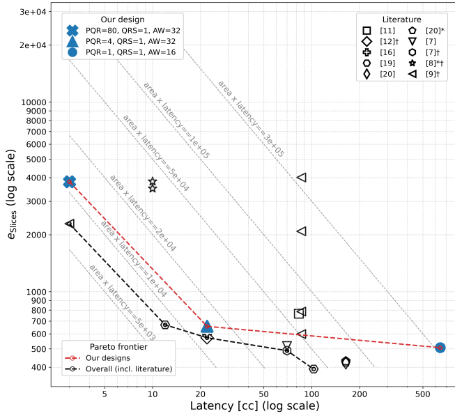
Fig. 4. Latency (x) vs eSlices (y) SoA comparison.
