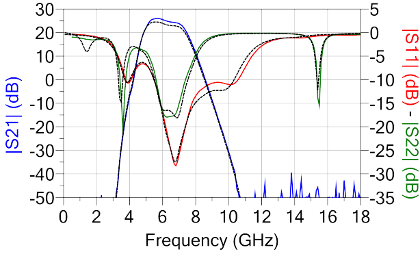
Fig. 8. Measured S-parameters (solid, colored) compared to simulations (dashed, black) of the proposed DPA based on improved power cell.
