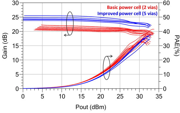
Fig. 7. Measured CW performance: comparison between the two DPA versions with basic (red) and 5-VIA (blue) power cell .
