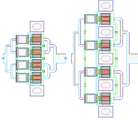
Fig. 1. Layout of the basic (left) and 5-VIA (right) power cells.
