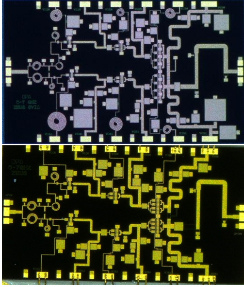
Fig. 4. Microscope picture of the two DPA versions with basic (bottom) and improved (top) power cell. Color differences are due to different set-ups adopted for taking the pictures.
