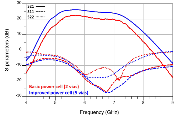
Fig. 6. Measured S-parameters: comparison between the two DPA versions with basic (red) and 5-VIA (blue) power cell.
