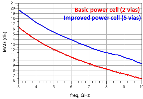
Fig. 2. Measured maximum available gain of the basic (red) and improved (blue) power cells.
