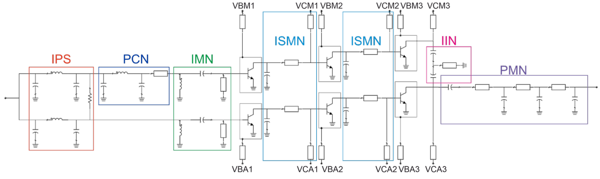
Fig. 3. Simplified schematic of the designed DPA. Device sizes for both the main (top branch) and auxiliary (bottom branch) are: 1 \times 3 \times 40 \mu\text{m}^2 (stage 1), 2 \times 3 \times 40 \mu\text{m}^2 (stage 2) and 4 \times 3 \times 40 \mu\text{m}^2 (stage 3).
