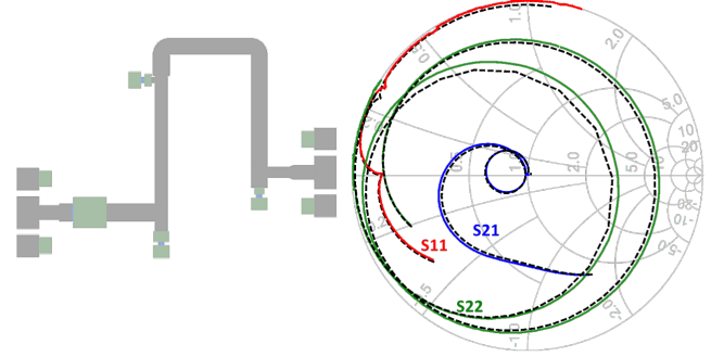
Fig. 5. Measured (solid, colored) vs simulated (dashed, black) S-parameters of the impedance inverting network cut-out shown on the left.
