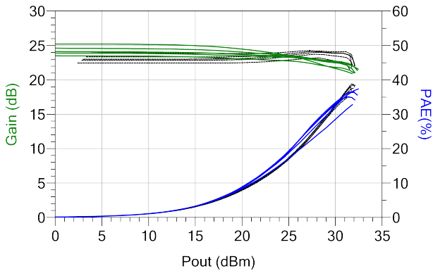
Fig. 9. Measured CW performance (solid, colored) compared to simulations (dashed, black) of the proposed DPA based on improved power cell.
