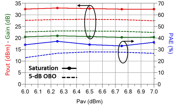
Fig. 10. Measured in-band performance at saturation (solid, symbols) and at 5 dB back-off (dashed) of the proposed DPA based on improved power cell.
