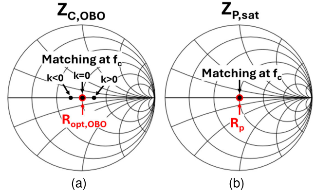
Fig. 3. Matching conditions imposed for (a) carrier and (b) peaking devices.
