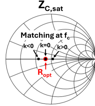
Fig. 6. Behavior of the carrier impedance at saturation at f_c based on k .
