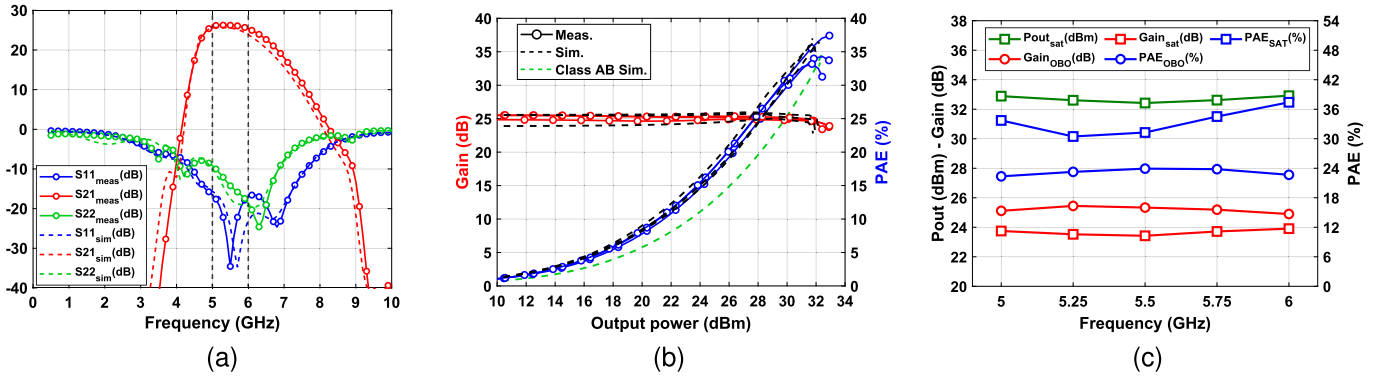
Fig. 19. (a) Comparison between measured (solid lines with circles) and simulated (dashed lines) small-signal parameters. Large-signal characterization: (b) gain and PAE versus output power and (c) performance at 6 dB OBO and saturation.
