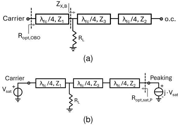
Fig. 5. Equivalent scheme of Type B combiner at (a) OBO and (b) saturation.
