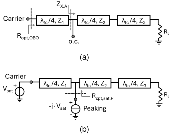
Fig. 4. Equivalent scheme of Type A combiner at (a) OBO and (b) saturation.
