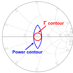
Fig. 7. Normalized 1-dB constant power contour and constant reflection coefficient contour.
