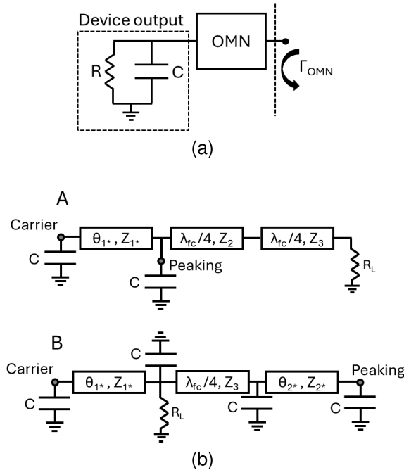
Fig. 12. Two possible approaches to compensate for device nonideal effects. (a) Using an OMN and (b) absorbing the output capacitances into the combiner.
