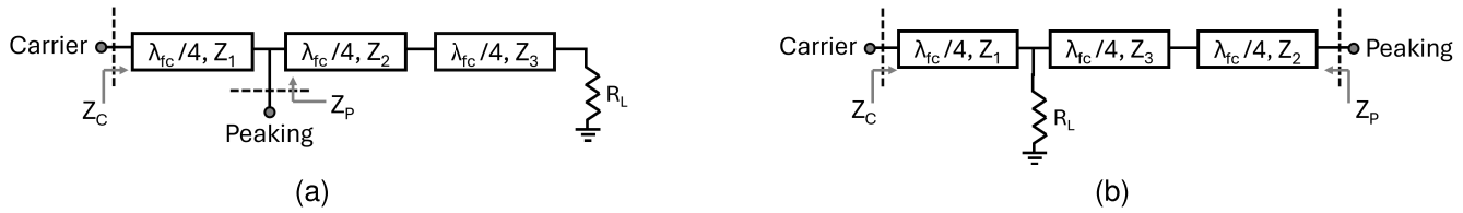
Fig. 2. Structure of the analyzed output combiners, hereafter referred as to (a) Type A and (b) Type B.
