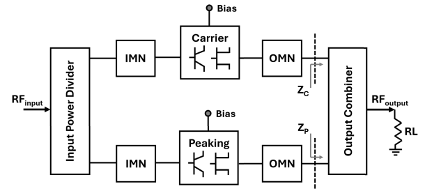
Fig. 1. Circuit diagram of a typical DPA architecture.
