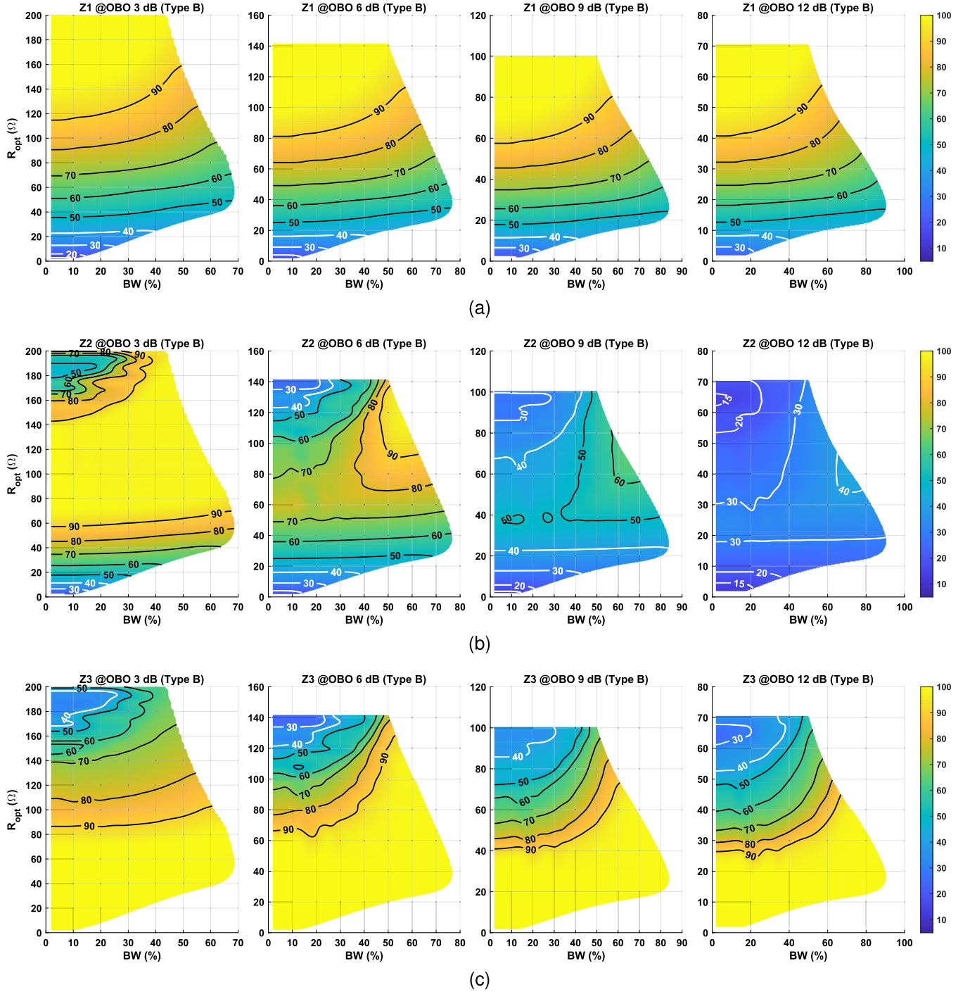
Fig. 10. Plots representing the value of (a) Z_1 , (b) Z_2 , and (c) Z_3 for Type B combiner at 3, 6, 9, 12 dB of OBO, as obtained from the optimization procedure.
