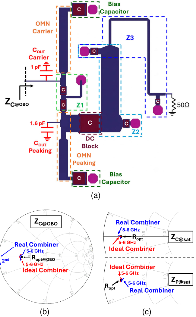
Fig. 15. (a) First version of the layout of the realized combiner, (b) comparison between the OBO carrier impedance of the ideal and real combiners, and (c) carrier and peaking loads at full power condition. The 2nd harmonic load is evaluated at the combiner plane.
