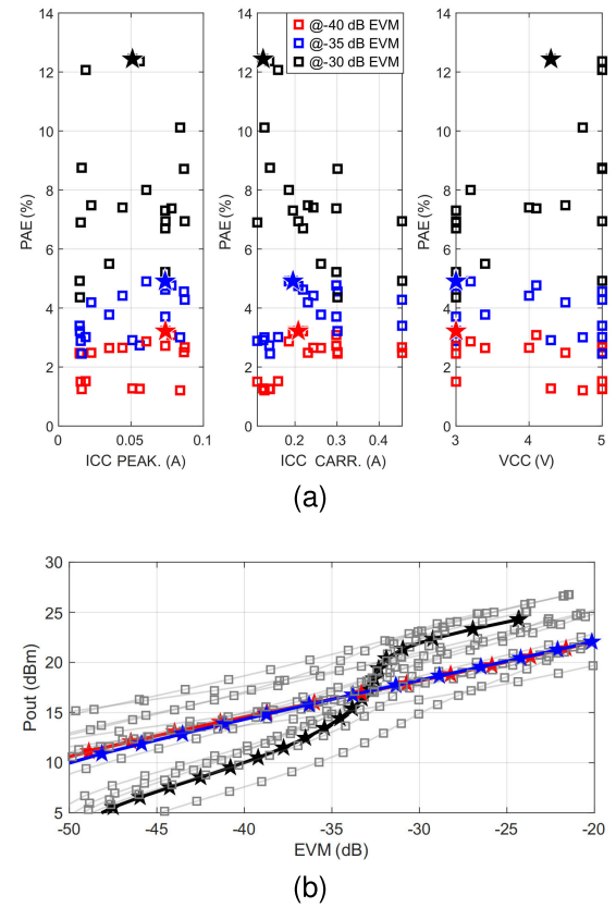
Fig. 20. (a) Results of the bias optimization process targeting the highest PAE at different EVM levels at 5.5 GHz and (b) corresponding output power. The star symbols identify the best performance for each EVM threshold: -40 dB (red), -35 dB (blue), and -30 dB (black).
