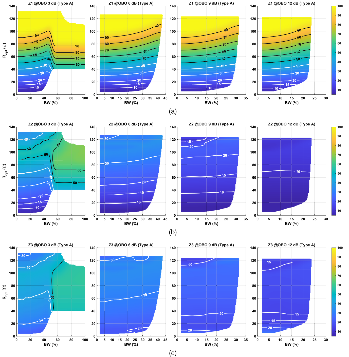
Fig. 9. Plots representing the value of (a) Z_1 , (b) Z_2 , and (c) Z_3 for Type A combiner at 3, 6, 9, 12 dB of OBO, as obtained from the optimization procedure.
