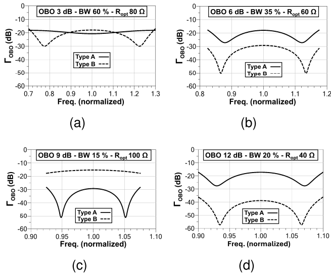
Fig. 11. Behavior of the reflection coefficient |\Gamma_{OBO}| in dB, for the various design requirements in Table I: (a) OBO = 3 dB, (b) OBO = 6 dB, (c) OBO = 9 dB, (d) OBO = 12 dB.
