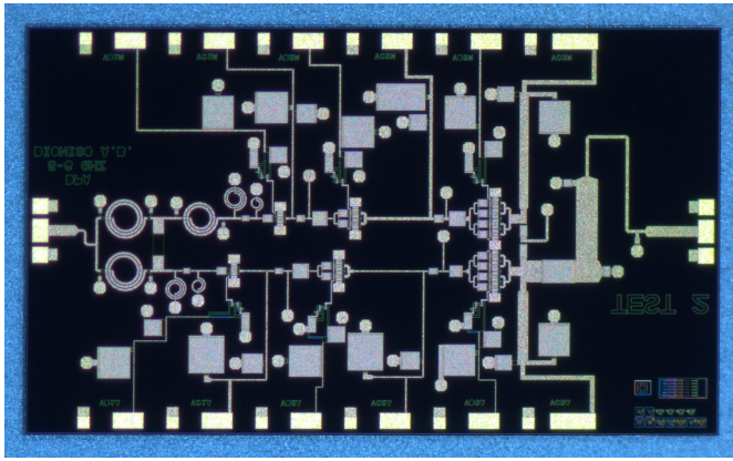
Fig. 17. Picture of the realized integrated DPA in HBT technology (size: 4.5 \times 2.5 mm).
