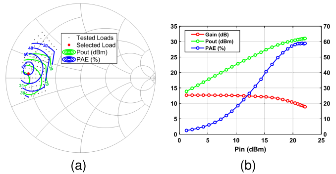
Fig. 14. (a) Investigated loads and selected one and (b) measured performance with the selected load.
