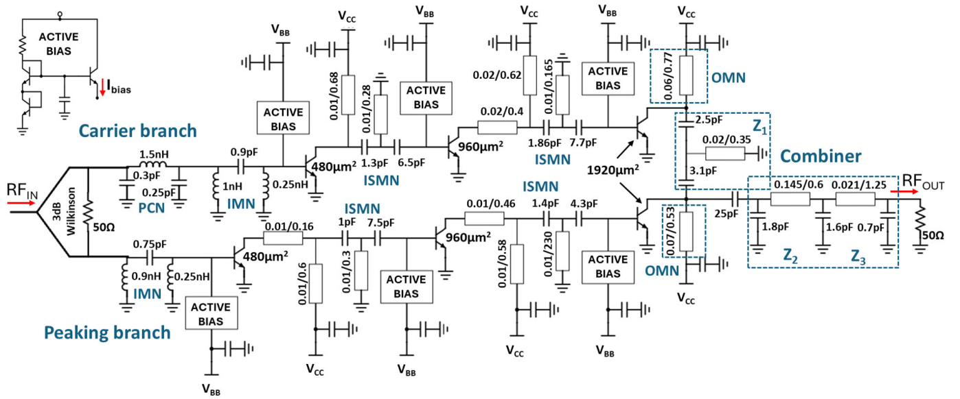
Fig. 16. Circuit diagram of the three-stage DPA, showing the values of lumped and distributed elements (length mm/width mm).
