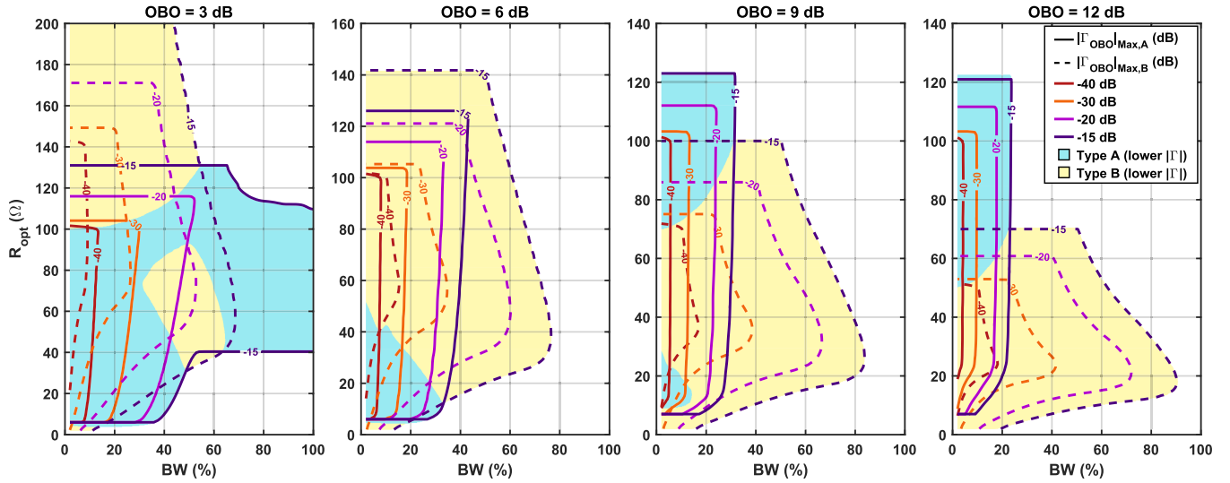
Fig. 8. Contour plots of the maximum value of |\Gamma_{OBO}| in dB for the Type A (solid lines) and B (dashed lines) combiner, in the case of 3-, 6-, 9-, and 12-dB OBO. Colored regions indicate which combiner provides the lower maximum reflection coefficient relative to R_{opt} and BW.
