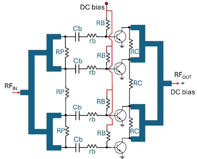
Fig. 13. Carrier and peaking final stage devices composed of four elementary HBTs.
