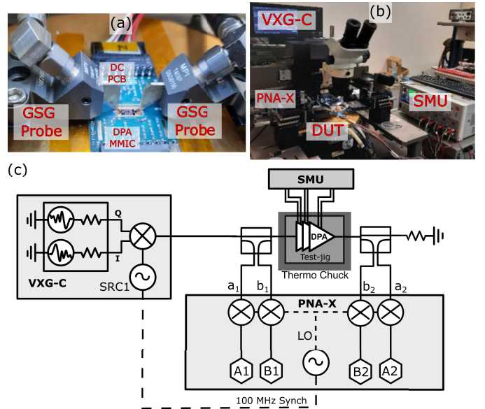
Fig. 18. (a) Test board for the DPA MMIC. Picture (b) and block diagram (c) of the measurement setup for the CW/modulated measurements.
