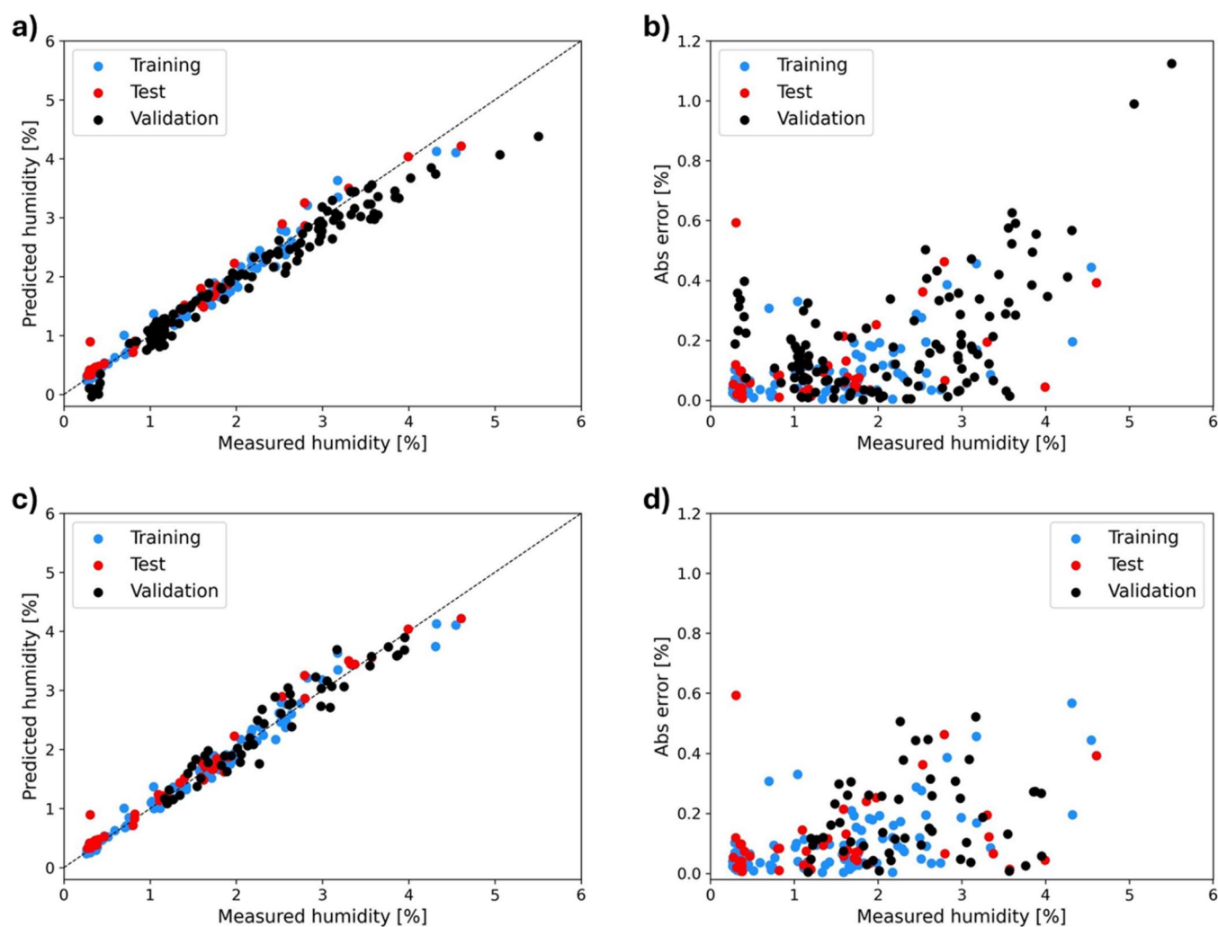
FIGURE 6 | Predicted humidity versus measured humidity of the ensemble model particularized for samples with different excipients, validated on mixed DPs (a) and on S3 + S9 samples (c). Absolute error [%] of the ensemble model particularized for samples with different excipients, validated on mixed DPs (b) and on S3 + S9 samples (d). Dataset from Massey et al. 2023 (Massey et al. 2023).
