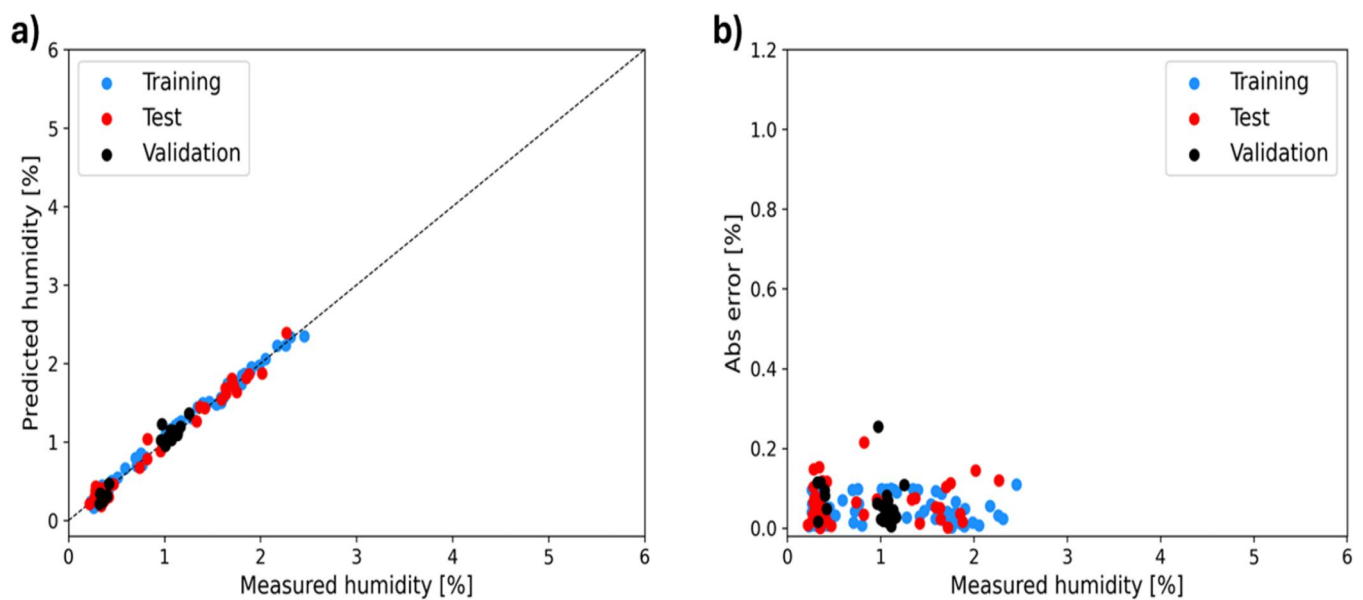
FIGURE 3 | Predicted humidity versus measured humidity (a) and absolute error [%] (b) of the ensemble model particularized for samples with DPs (Product 2 set), validated on DPs (Product 2 set).
