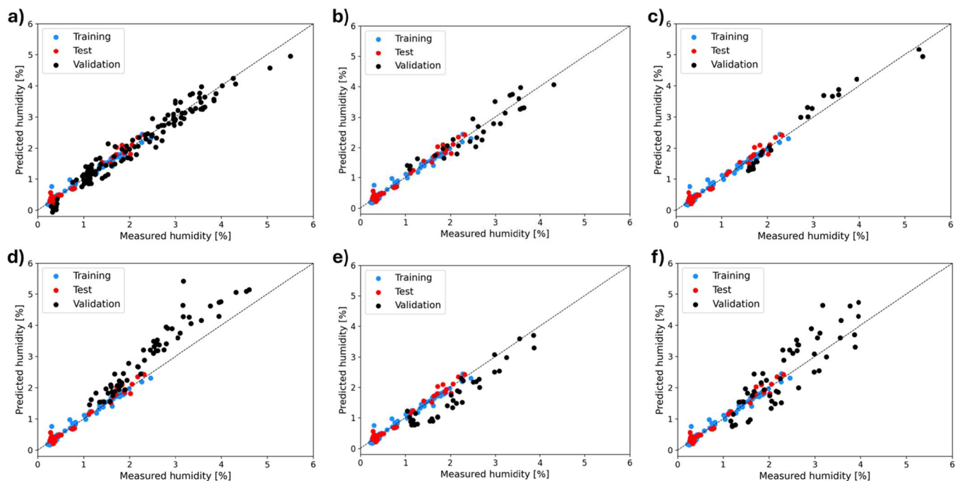
FIGURE 4 | Predicted humidity versus measured humidity for the ensemble model on: (a) mix DP, (b) SA3, (c) T6, (d) S3, (e) S9, (f) S3 + S9; datasets from Massey et al. 2023 (Massey et al. 2023).
