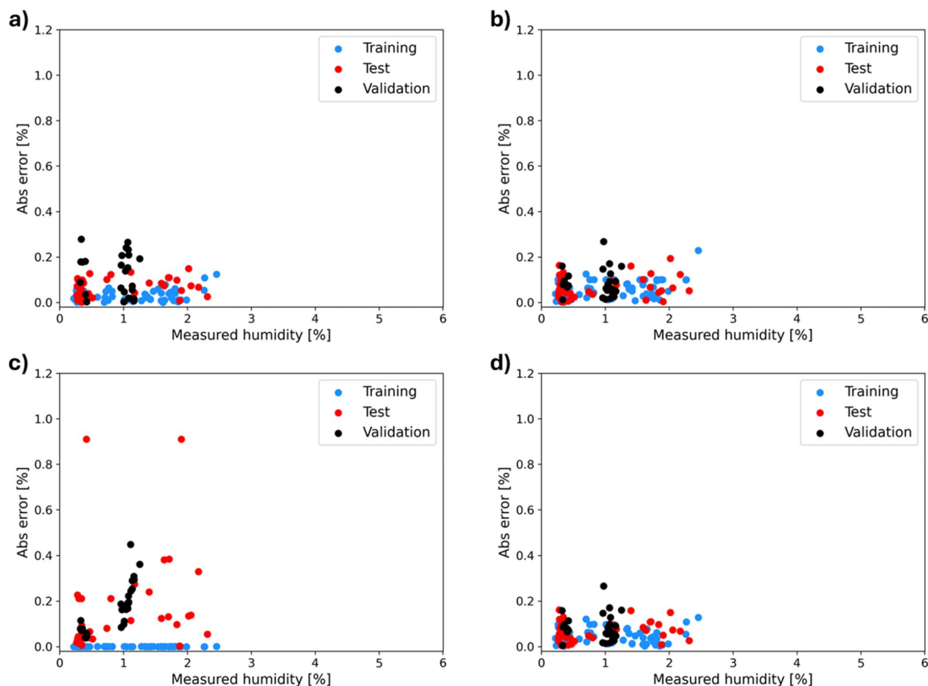
FIGURE 2 | Absolute error [%] of PLS model (a), SVR model (b), XGBoost model (c), and ensemble model (d) on the ad-hoc dataset.
