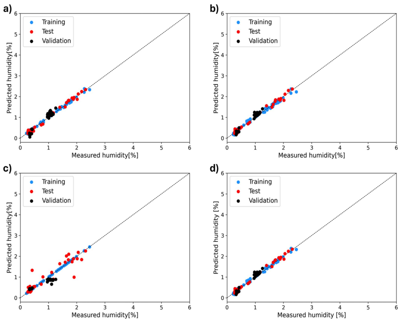
FIGURE 1 | Predicted humidity versus measured humidity for PLS model (a), SVR model (b), XGBoost model (c), and ensemble model (d) on the ad-hoc dataset.
