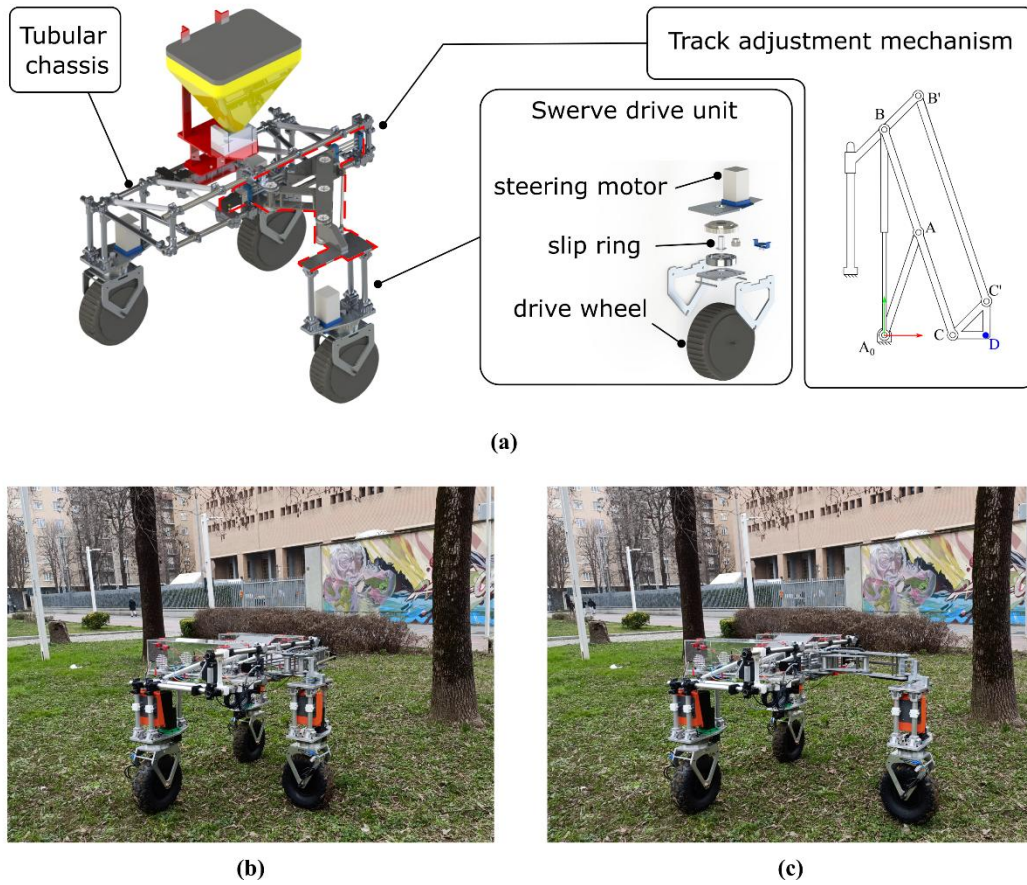
Figure 1 (a) AGRIMARO.Q drawing with main components highlighted. (b) Prototype made and pictured in its compact configuration (minimum track width). (c) Prototype in extended configuration.
