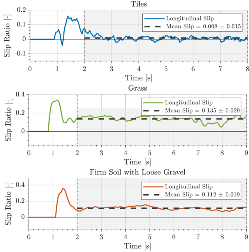
Figure 5 Real-Time Longitudinal Slip estimation on representative types of greenhouse terrains: Tiles, Grass, Firm Soil with Loose Gravel.
