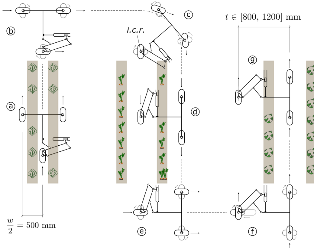
Figure 2 Representation of possible locomotion strategies of the AGRIMARO.Q UGV while navigating crop rows with variable spacing. (a) Forward motion in delta configuration, (b) wheel steering for transversal motion, (c) chassis rotation with one wheel as center of rotation, (d) forward motion in triangular configuration, (e) transversal motion, (f) wheel steering and track adjustment for a bigger crop spacing, (g) forward motion.
