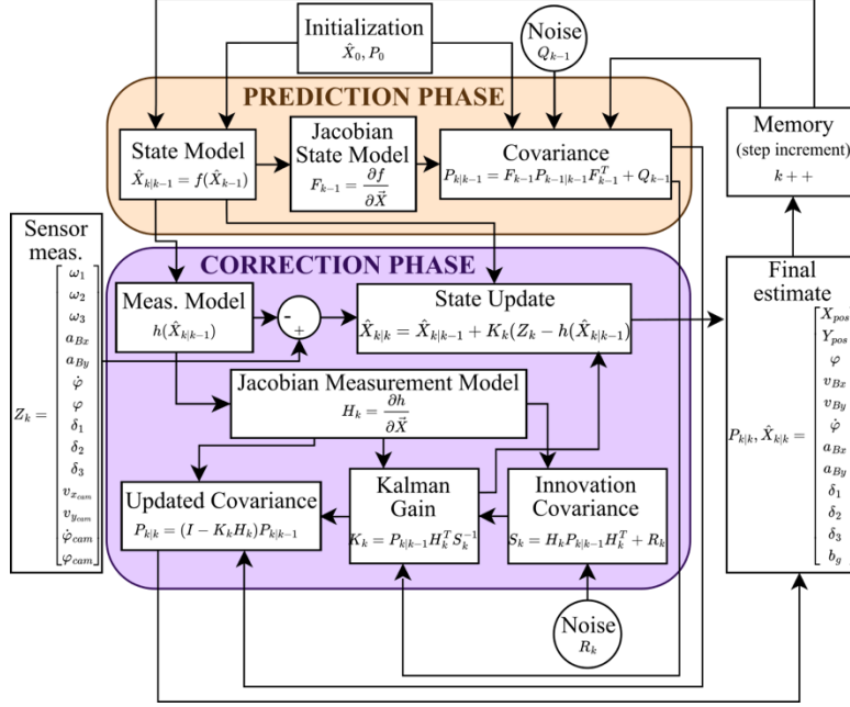
Figure 4 Schematic representation of the Extended Kalman Filter (EKF) developed for AgriMaRo.Q UGV.
