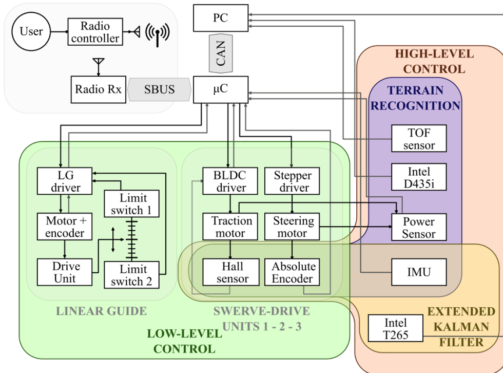
Figure 3 Schematic representation of the electronic control system including low and high-level control.
