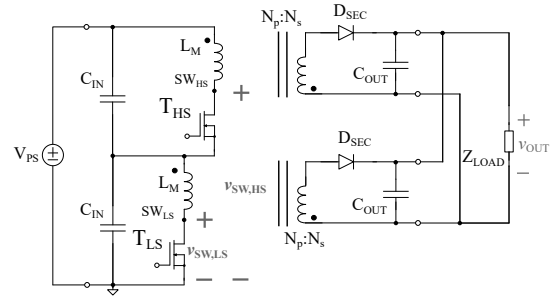
Fig. 1. Traditional ISOP flyback converter.
