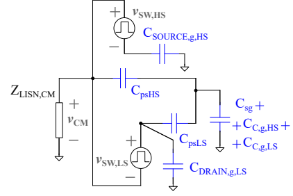
Fig. 3. Simplified equivalent common mode model of symmetrical ISOP flyback.
