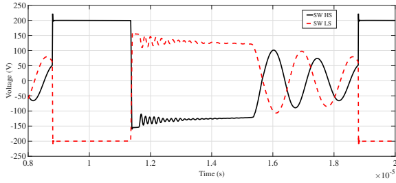
Fig. 5. High side and low side switching node voltages with only CMB condition satisfied
