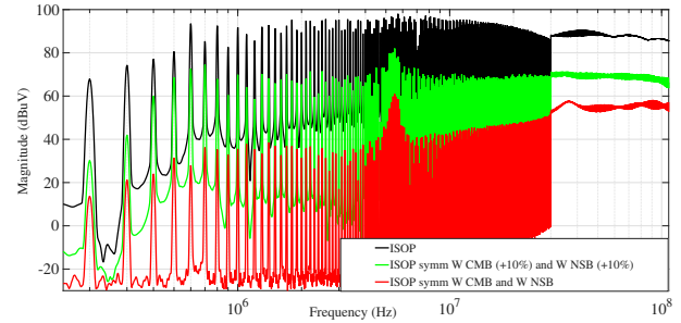
Fig. 8. Comparison of CM EMI frequency spectrum of traditional ISOP flyback, symmetrical ISOP flyback with nominal values of compensation capacitors, and with a relative variation of both capacitors of +10%.
