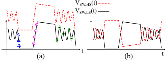
Fig. 4. High-side and low-side switching nodes waveforms for conventional ISOP flyback (a) and symmetrical ISOP flyback (b).
