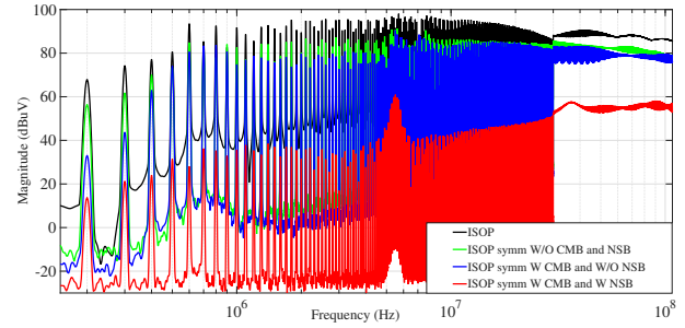
Fig. 7. Comparison of CM EMI frequency spectrum of traditional ISOP flyback, symmetrical ISOP flyback without CMB and NSB satisfied, with only CMB condition satisfied and with both conditions satisfied.
