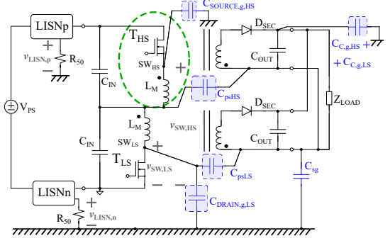
Fig. 2. Schematic of symmetrical ISOP flyback including LISNs for conducted EMI evaluation. The parasitic elements determining CM are encircled in dashed boxes.
