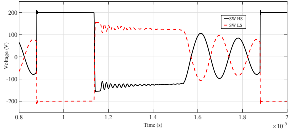
Fig. 6. High side and low side switching node voltages with both CMB and NSB conditions satisfied
