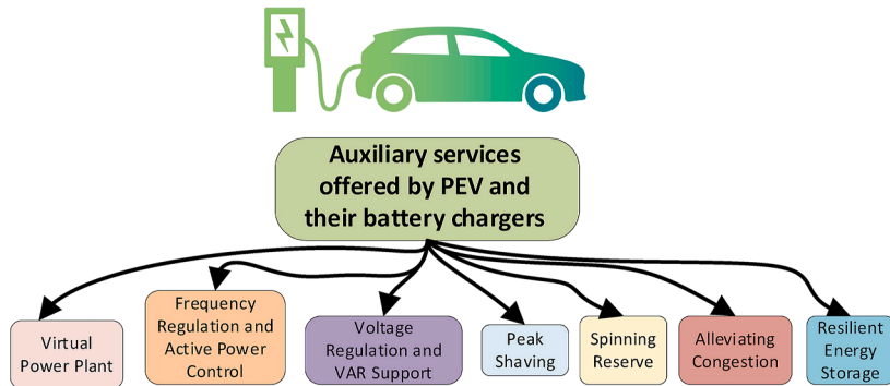
FIGURE 12.14 Potential vehicle-to-grid (V2G) auxiliary services from plug-in electric vehicles (PEVs).
