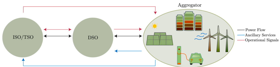
FIGURE 12.9 Conceptual framework for multiactor coordination in power systems.
