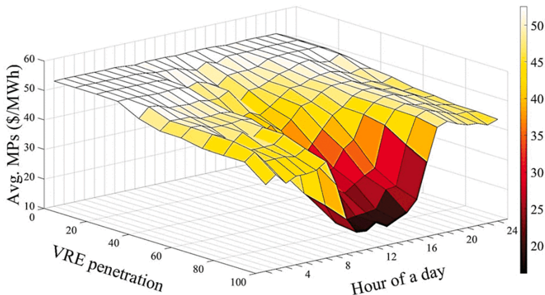
FIGURE 12.10 Impact of variable renewable energy (VRE) penetration on marginal electricity prices.
