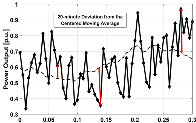
FIGURE 12.4 Deviation from the centered moving average (20-min window).
