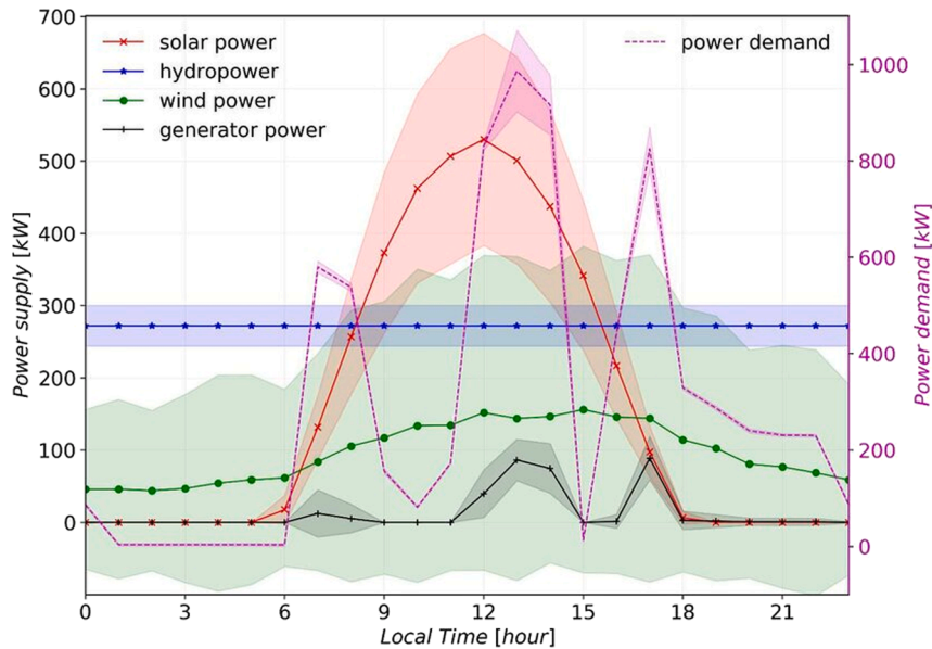
FIGURE 12.6 Diurnal variations in power generation from multiple renewable sources.
