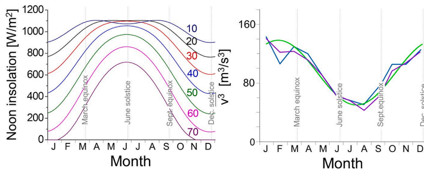
FIGURE 12.5 Seasonal variations in solar irradiance and wind resources.
