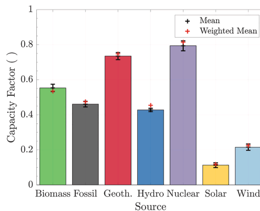
FIGURE 12.7 Capacity factors for renewable and nonrenewable power generation sources.
