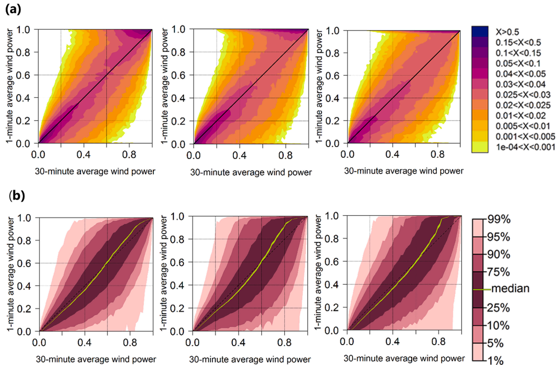
FIGURE 12.2 Conditional probability of short-term wind power fluctuations.
