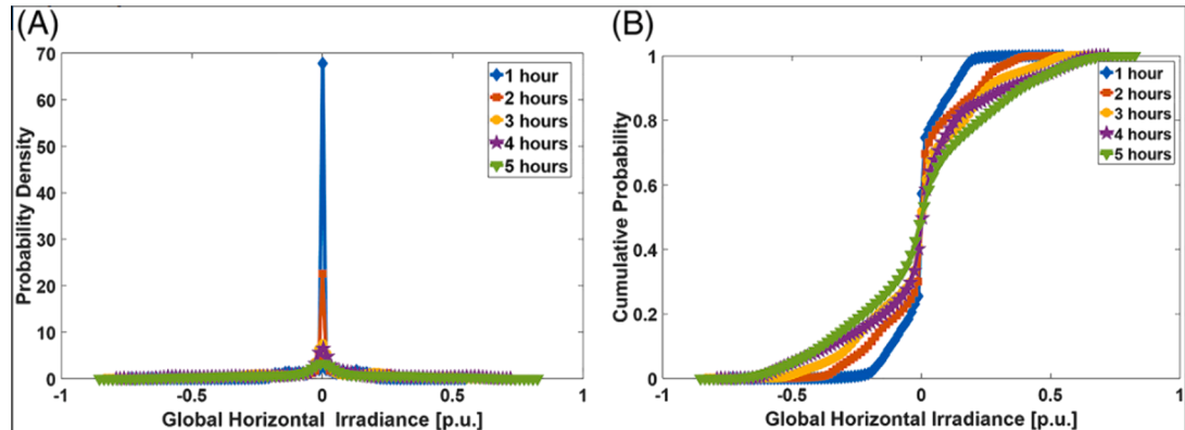
FIGURE 12.3 Step changes in wind power output and irradiance across temporal resolutions.
