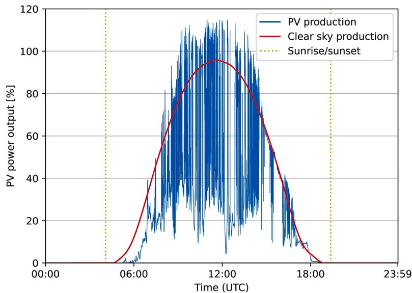
FIGURE 12.1 Variability of PV output under clear-sky and cloudy conditions.
