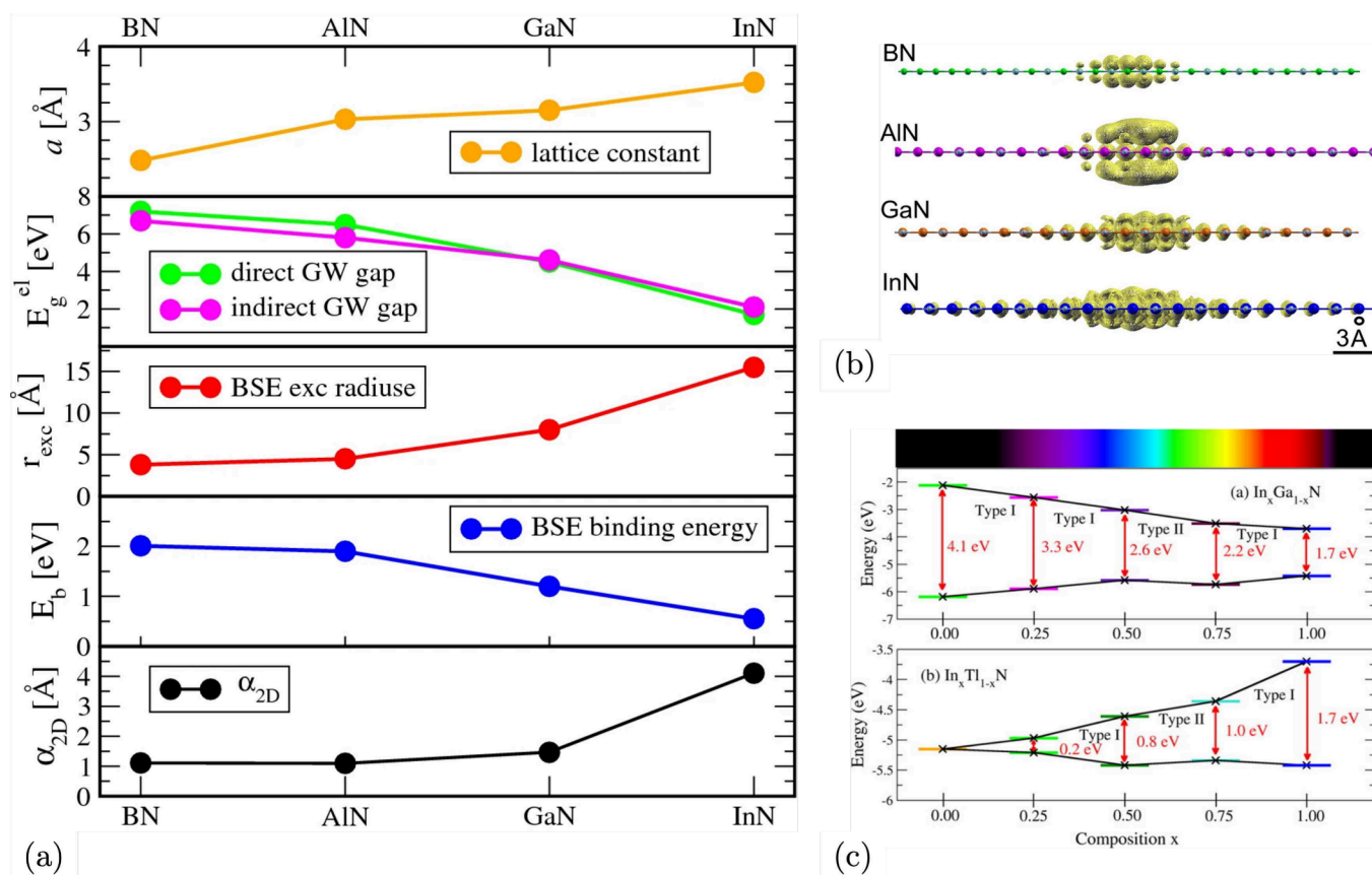
Figure 3. Trends in Group III-Nitrides. (a) Lattice constant, direct and indirect quasiparticle gaps, exciton radius, exciton binding energy and 2D static polarizability for BN, AlN, GaN, and InN. (b) Exciton wave functions for the 2D nitrides. Adapted from ref 9. CC BY 4.0. (c) Direct band gap and band extrema with respect to the vacuum level of In_xGa_{1-x}N (upper panel) and In_xTl_{1-x}N (lower panel). Adapted with permission from ref 65. Copyright 2017 AIP Publishing.
