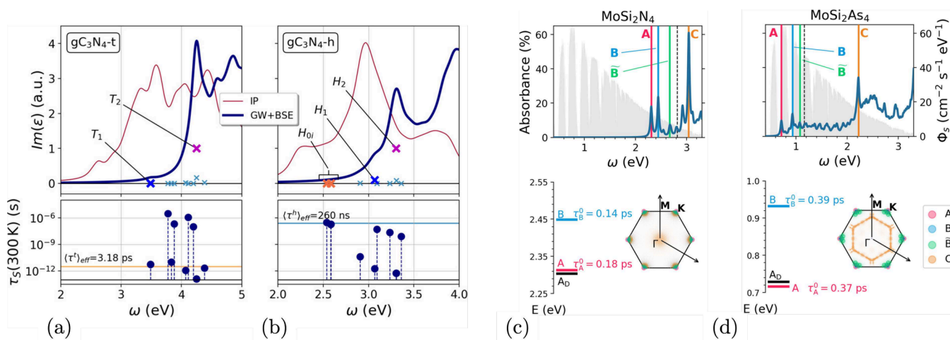
Figure 2. (a, b) Absorption spectra and radiative lifetimes in 2D materials. Optical absorption and exciton radiative lifetimes for the \text{gC}_3\text{N}_4 polymorphs triazine in (a) and heptazine in (b). Adapted from ref 11. CC BY 4.0. (c, d) Absorption, exciton energy ordering, radiative lifetimes, and exciton weights in the Brillouin zone for \text{MoSi}_2\text{N}_4 in (c) and \text{MoSi}_2\text{As}_4 in (d). Adapted from ref 12. CC BY 4.0.
