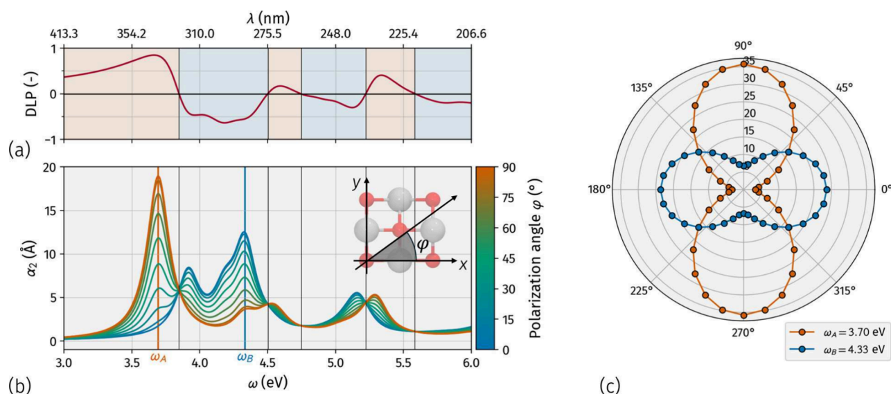
Figure 1. Linear dichroism inversion with photon energy in monolayer SnO. (a) Degree of linear polarization (DLP). (b) Absorption spectra for different in-plane light polarization angles \varphi . (c) Polar plot of absorption at lower ( \omega_A ) and higher ( \omega_B ) frequencies. Adapted from ref 15. Copyright 2025 American Chemical Society.
