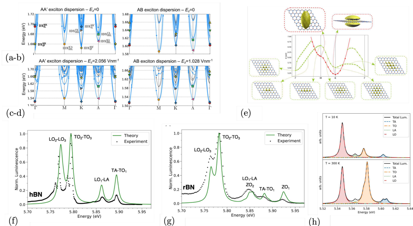
Figure 5. Exciton–phonon interactions in 2D materials. (a–d) Calculated exciton dispersion curves for bilayer WSe 2 : (a) AA' stacking at external electric field E_z = 0 ; (b) AB stacking at E_z = 0 ; (c) AA' stacking at E_z = 2.056 V/nm; (d) AB stacking at E_z = 1.028 V/nm. Labels indicate direct and indirect excitons (DX and IDX) and layer localization nature: in-plane (IP), interlayer (IL), or hybrid interlayer (HIL). Adapted with permission from ref 91. Copyright 2025 the authors of ref 91, exclusive license to American Chemical Society. (e) Exciton dispersion of monolayer hBN. The \pi \rightarrow \pi^* ( \pi \rightarrow \sigma^* ) exciton branch is in green (red). The corresponding real-space exciton wave functions at different momenta are plotted in the insets. Adapted with permission from ref 17. Copyright 2023 American Physical Society. (f, g) Phonon-assisted luminescence in AA'-stacking bulk BN (top) and ABC-stacking rhombohedral bulk BN (bottom). Black: cathodoluminescence experiment. Green: ab initio exciton–phonon calculation. The phonon modes responsible for the peaks are labeled. Adapted with permission from ref 43. Copyright 2023 American Physical Society. (h) Phonon-assisted luminescence in cubic BN. Top: T = 10 K. Bottom: T = 300 K. Adapted with permission from ref 45. Copyright 2026 AIP Publishing.
