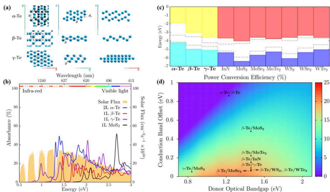
Figure 4. Optoelectronic properties of tellurene polymorphs. (a) Optimized geometric structures of 2L \alpha -Te, 1L \beta -Te, and 1L \gamma -Te. (b) Comparison of the optical absorption spectra of 2L \alpha -Te, 1L \beta -Te, and 1L \gamma -Te with MoS 2 (black). (c) Comparison of the band-offset alignment between 2L \alpha -Te, 1L \beta -Te, and 1L \gamma -Te and other monolayer 2D semiconducting materials calculated at the GW level. Black dashed lines show the relative alignment from DFT calculations. (d) Heatmap of the power conversion efficiency plotted as a function of the donor optical band gap and of the conduction band offsets. The black dots refer to the efficiency of the heterostructures shown in (c). Adapted with permission from ref 52. Copyright 2024 Wiley-VCH.
