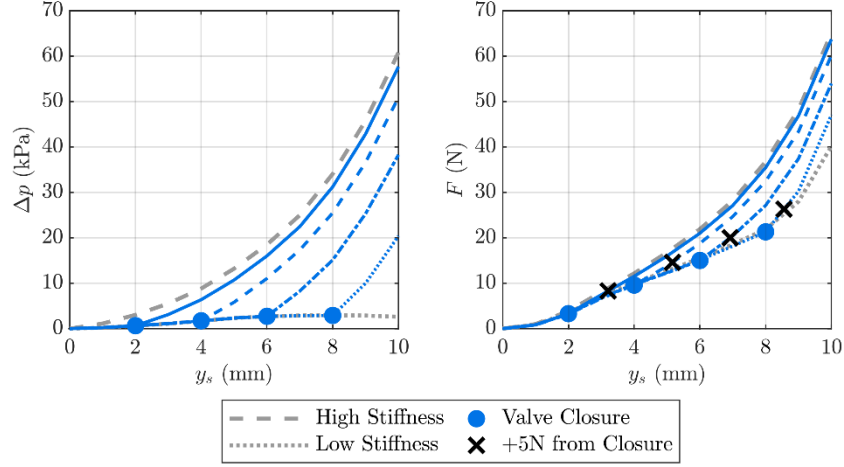
Fig. 5 – Analysis of the transition from low to high stiffness configuration at different contact depths y_s .
