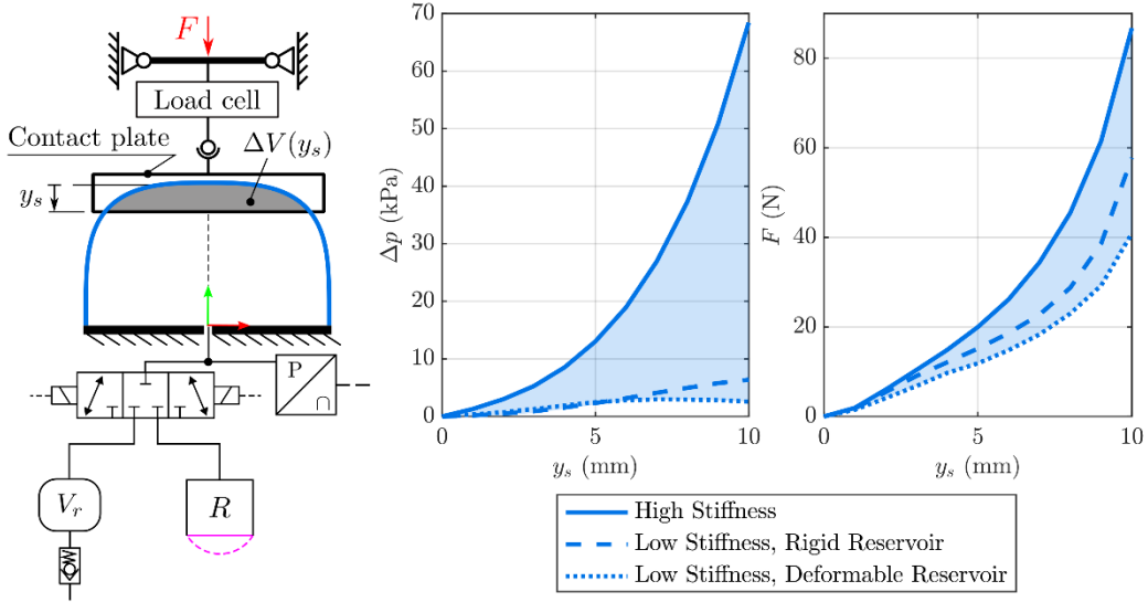
Fig. 4 – Comparison of the static pressures and forces obtained by connecting the SPSC unit either to a rigid or a deformable reservoir. The performance with the SPSC unit isolated is reported as well.
