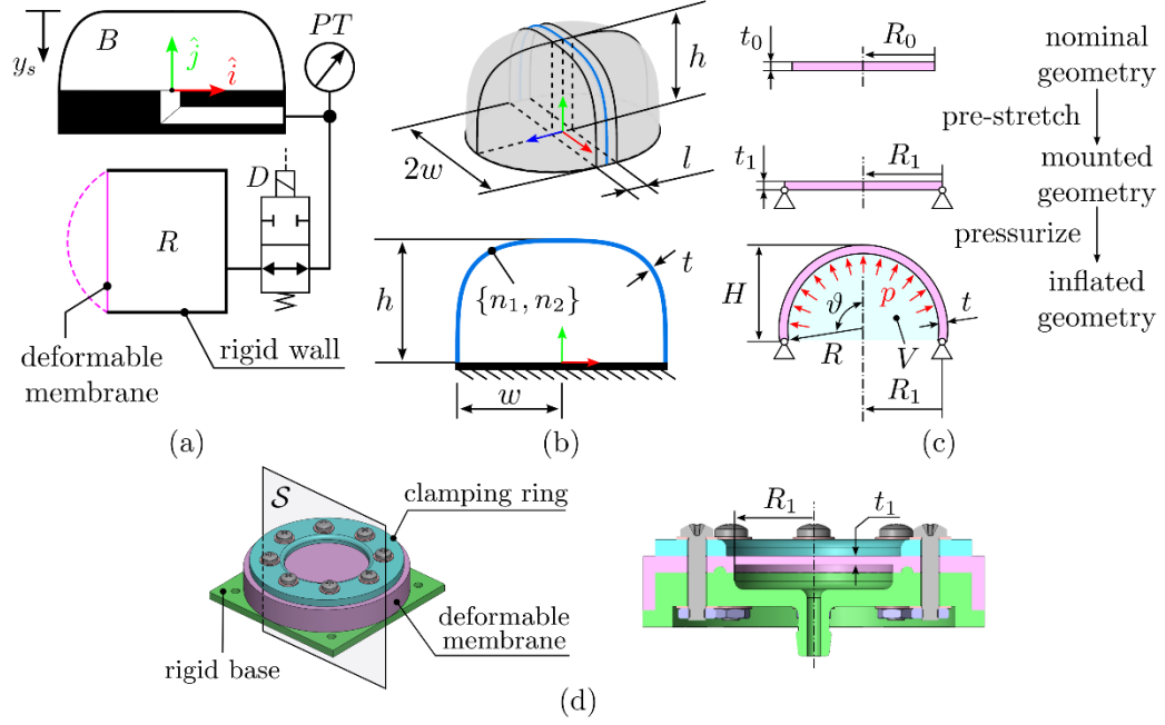
Fig. 1 – (a) SPSC system with a deformable reservoir. The pink solid line represents the initial configuration, while the dashed line the deformed one. (b) Geometric definition of the SPSC unit and its relevant parameters. (c) Nominal, mounted, and inflated geometry of the deformable membrane, with relevant parameters. Mounting the membrane on the rigid base requires to pre-stretch the membrane to increase its radius from R_0 to R_1 . (d) Axonometric view of the deformable reservoir and section view through plane \mathcal{S} .
