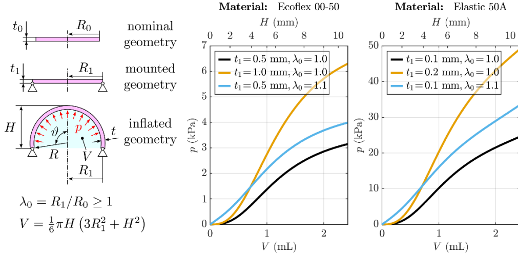
Fig. 2 – Parametric analysis of the pressure–volume curve obtained by combining different materials, thicknesses and pre-stretching ratios. In this instance, R_1 is fixed at 10.5 mm.
