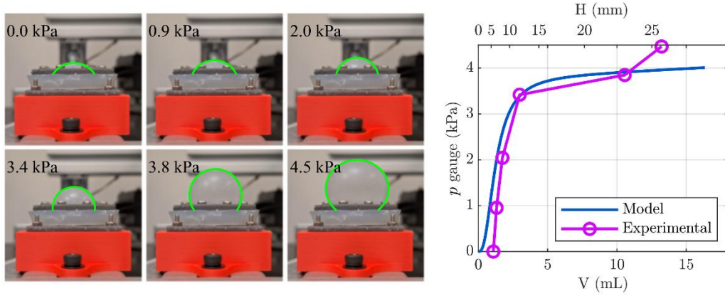
Fig. 3 – Experimental characterization of a deformable reservoir with R_0 = 10.5 mm, t_0 = 0.5 mm and \lambda_0 = 1 , and comparison between the experimental and estimated pressure–volume curves.
