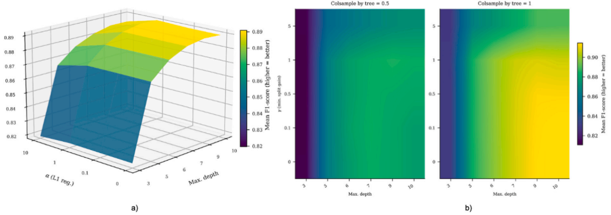
Fig. 6. Adjusting hyperparameters of the XGBoost classifier using grid search.
