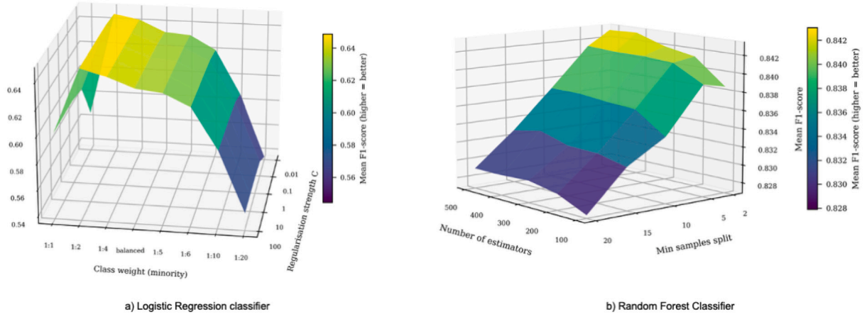
Fig. 5. Adjusting hyperparameters of a) Logistic regression and b) Random Forest using grid search.
