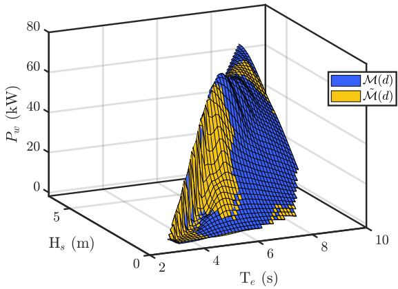
Fig. 25. P(H_s, T_e, d) comparison between the numerical model \mathcal{M}(d) and the meta-model \tilde{\mathcal{M}}(d) for a selected PEWEC design, in the CDS case.
