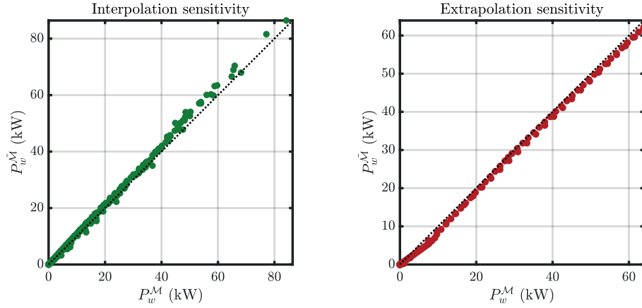
Fig. 28. Sensitivity analysis outcomes, comparing power production of the surrogate model and the reference numerical model for the two investigated sets of sea states.
