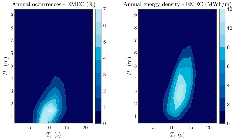
Fig. 20. Wave energy occurrences and energy density matrices for the EMEC test site.
