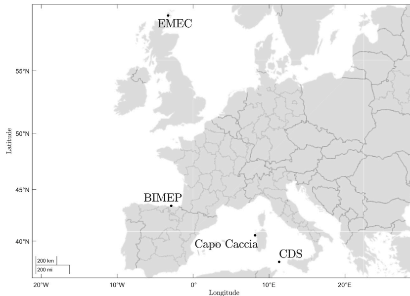
Fig. 18. North sea (BIMEP, EMEC) and Mediterranean (CDS and Capo Caccia) sites analyzed.
