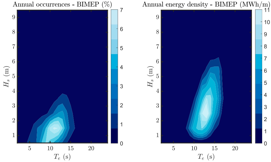
Fig. 19. Wave energy occurrences and energy density matrices for the BIMEP test site.
