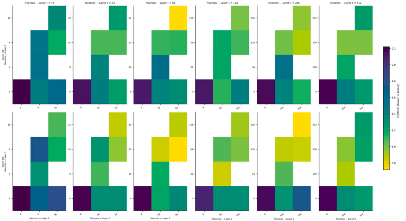
Fig. 11. Adjusting hyperparameters of a Feedforward Neural Network regressor using grid search.
