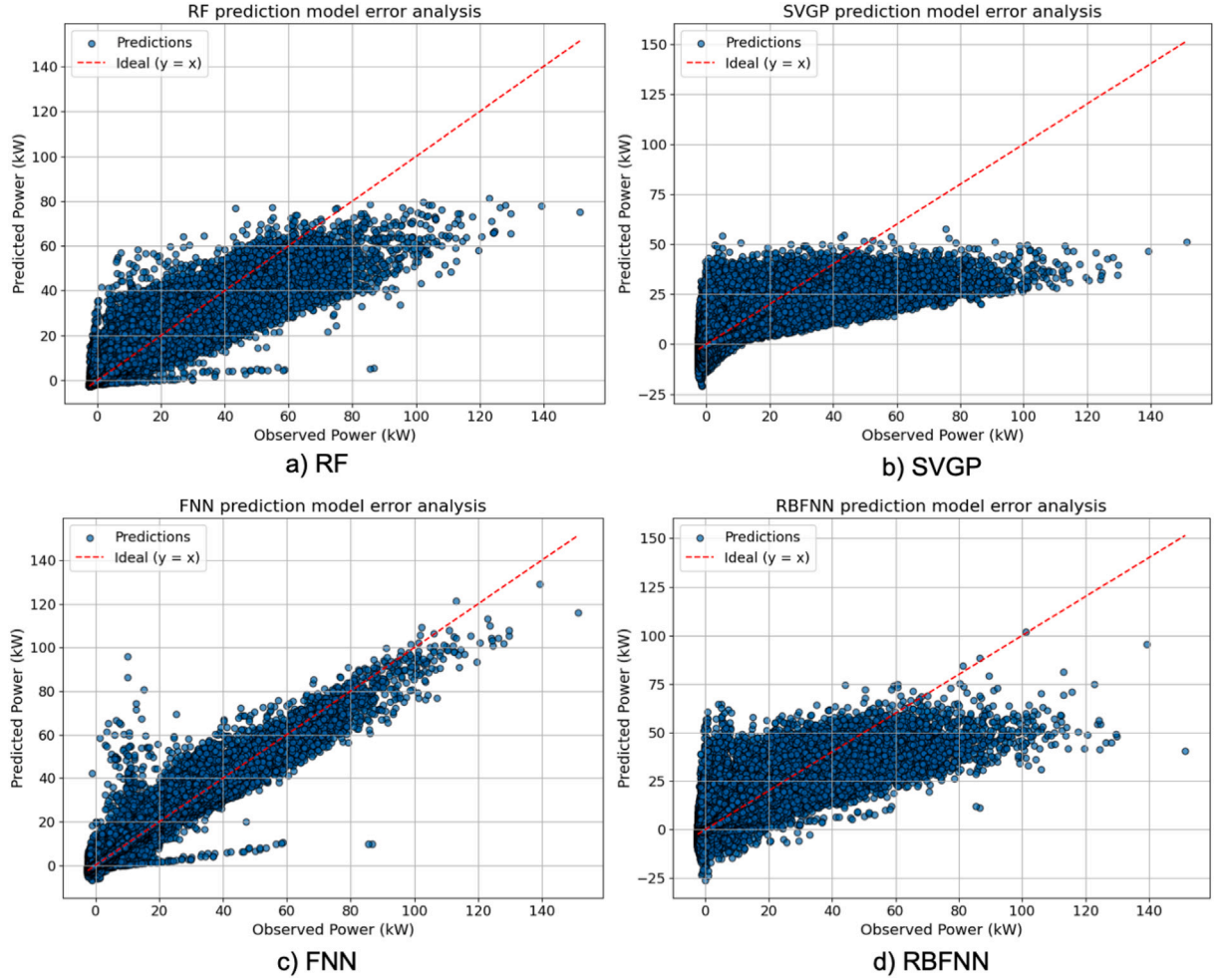
Fig. 14. Comparison of regression models, power predictions, and observed values of the test set.
