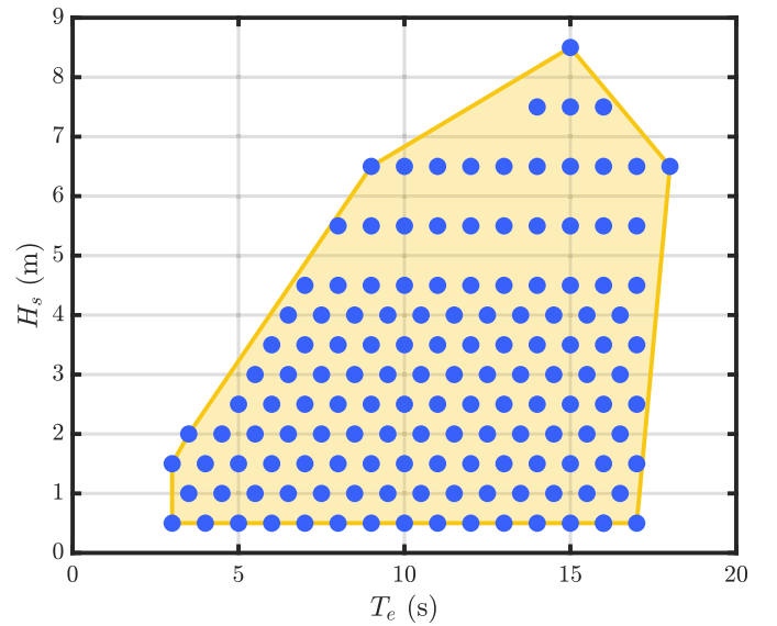
Fig. 4. Set of the 141 representative waves. In blue dots are shown the 141 sea states and in yellow the covered area. (For interpretation of the references to colour in this figure legend, the reader is referred to the web version of this article.)
