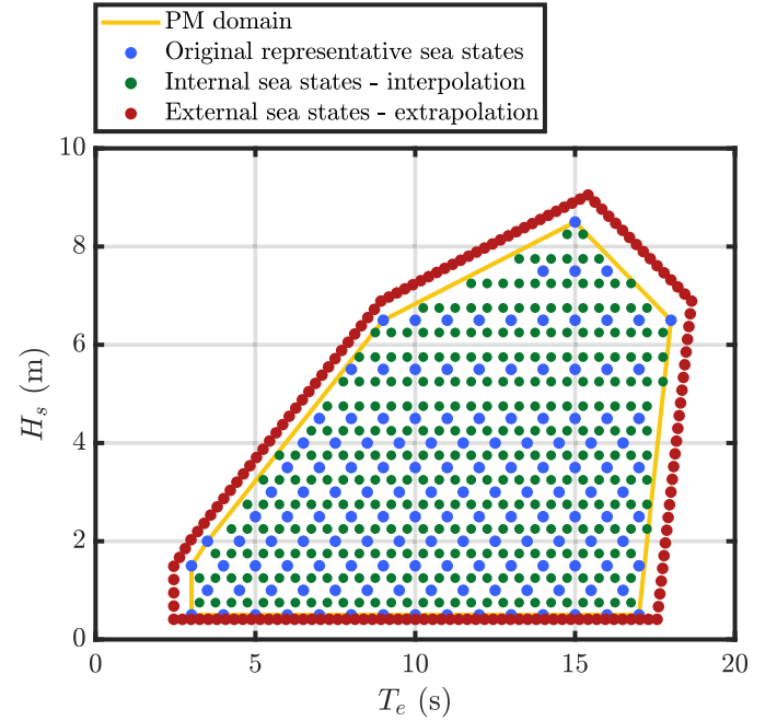
Fig. 27. Sets of sea states employed for the sensitivity analysis.
