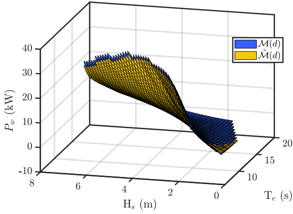
Fig. 23. P(H_s, T_e, d) comparison between the numerical model \mathcal{M}(d) and the meta-model \tilde{\mathcal{M}}(d) for a selected PEWEC design, in the BIMEP case.
