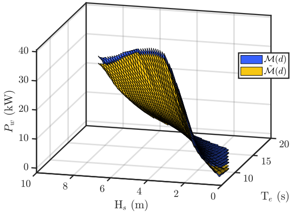
Fig. 24. P(H_s, T_e, d) comparison between the numerical model \mathcal{M}(d) and the meta-model \tilde{\mathcal{M}}(d) for a selected PEWEC design, in the EMEC case.
