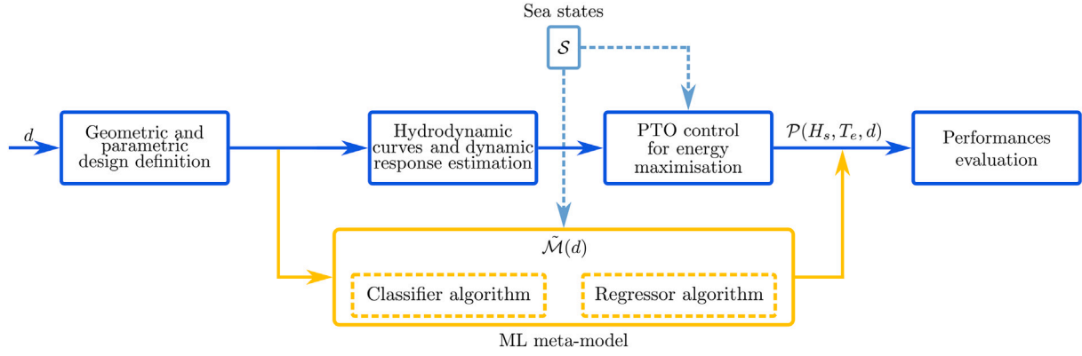
Fig. 1. Schematization of the DD/DB general surrogate model approach.
