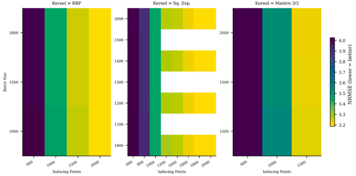
Fig. 10. Adjusting hyperparameters of Stochastic Variational Gaussian process model using grid search.
