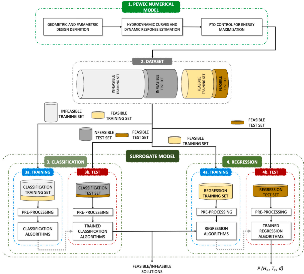
Fig. 2. Schema of the proposed methodology.
