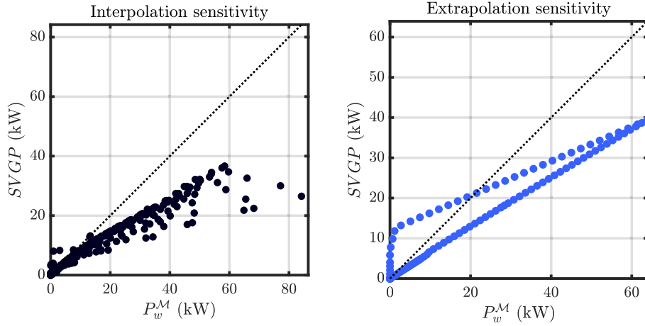
Fig. 30. Sensitivity analysis of the SVGP baseline, comparing the power production of the SVGP model and the reference numerical model for the two investigated sets of sea states.
