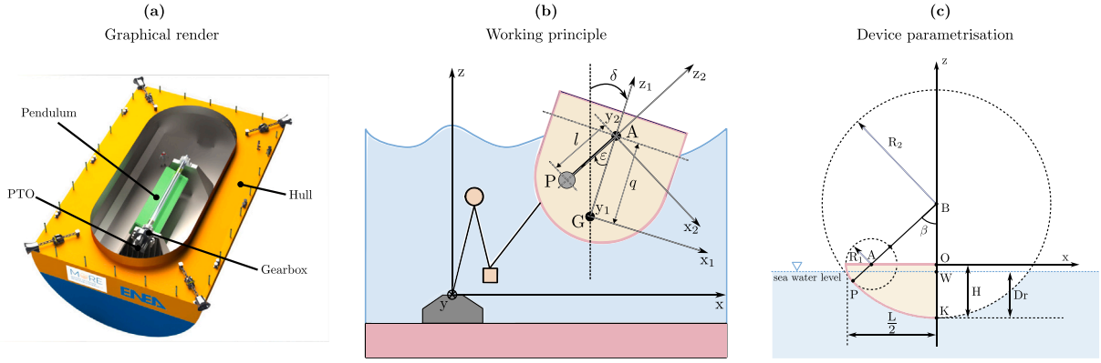
Fig. 3. PEWEC graphical rendering (a), working principle (b), and device parametrization (c).
