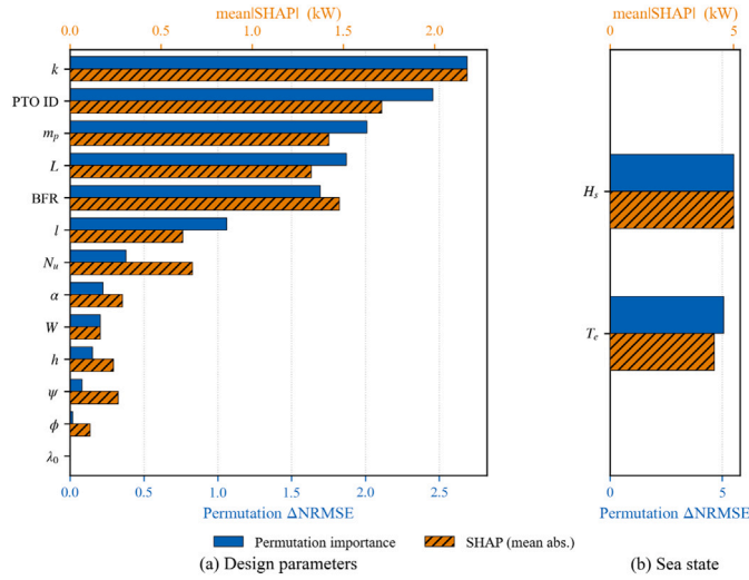
Fig. 17. Feature importance of the FNN regressor, obtained by permutation importance bottom axis and by SHAP (top axis), for (a) the thirteen design parameters and (b) H_s and T_e .
