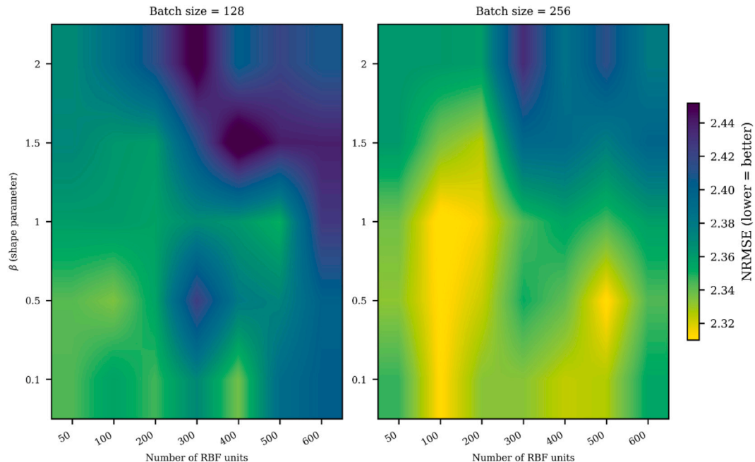
Fig. 12. Adjusting the hyperparameters of a Radial Basis function Neural Network regressor using grid search.
