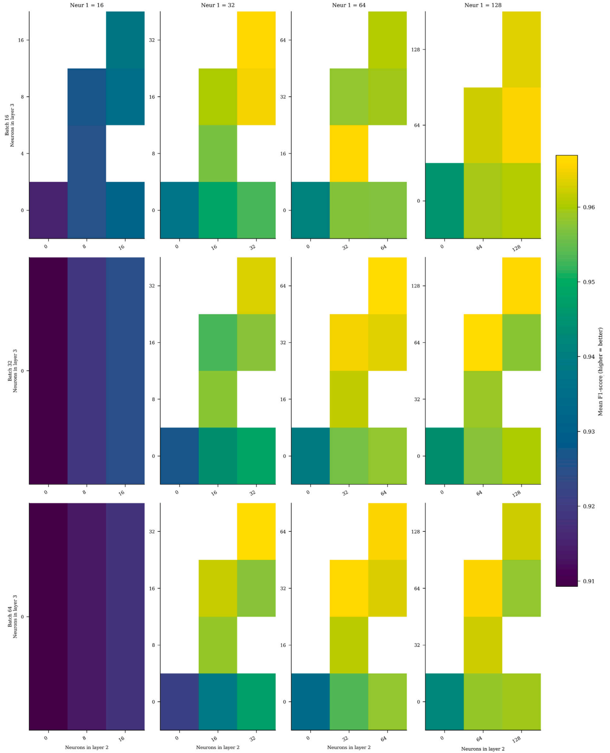
Fig. 8. Adjusting the hyperparameters of a Feedforward Neural Network classifier using grid search.
