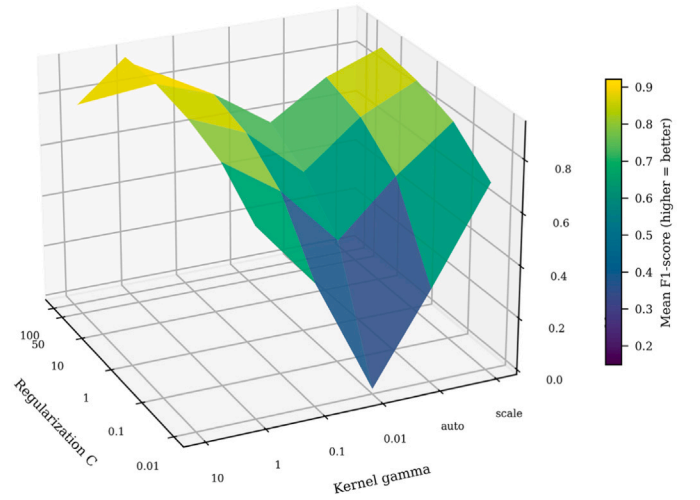
Fig. 7. Adjusting hyperparameters of a Support vector classifier using grid search.
