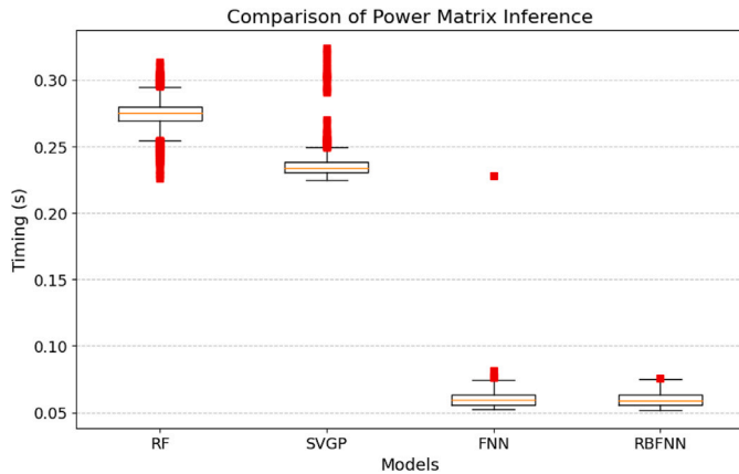
Fig. 15. Comparison of regression models inference times for the power matrix of the 141 N_c sea states.
