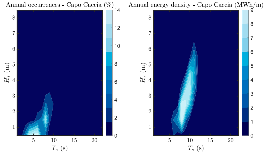
Fig. 22. Wave energy occurrences and energy density matrices for the Capo Caccia test site.
