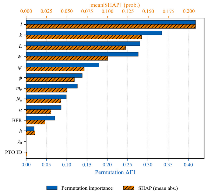
Fig. 16. Feature importance of the FNN classifier, obtained by permutation importance bottom axis) and by SHAP (top axis), for the thirteen design parameters.
