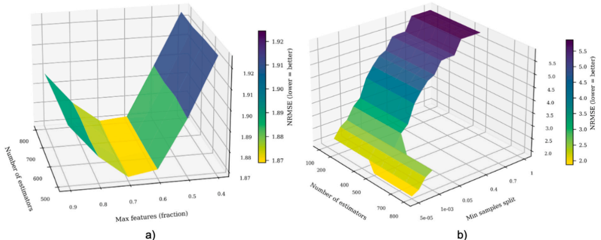
Fig. 9. Adjusting the hyperparameters of a Random Forest regressor using grid search.
