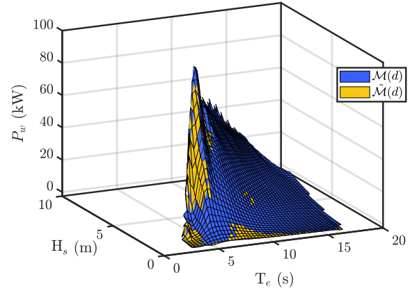
Fig. 26. the P(H_s, T_e, d) comparison between the numerical model \mathcal{M}(d) and the meta-model \tilde{\mathcal{M}}(d) for a selected PEWEC design, Capo Caccia case.
