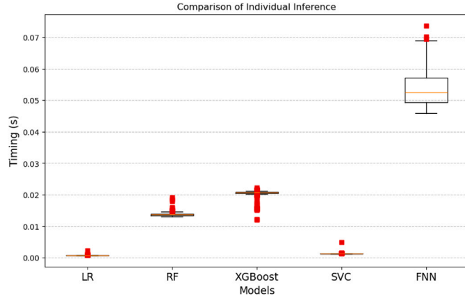
Fig. 13. Comparison of classifier algorithms inference time.
