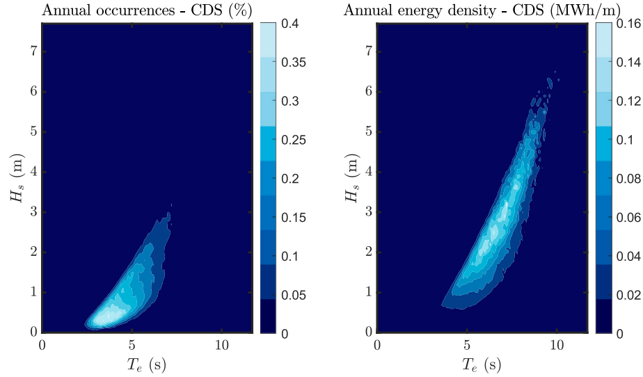
Fig. 21. Wave energy occurrences and energy density matrices for the CDS test site.
