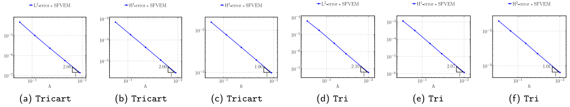
Fig. 2. Test 2. Convergence plots of the L^2 , H^1 and H^2 errors on the Tricart mesh and the Tri mesh. The reported convergence rate is obtained using the four finest refinements.
