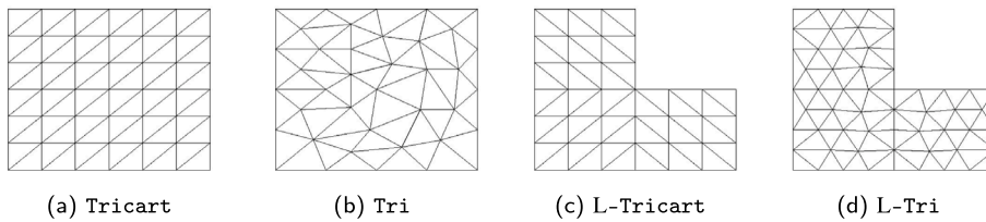
Fig. 1. Meshes used in the numerical tests on the source and spectral problems.
