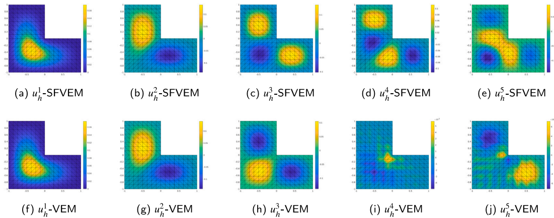
Fig. 3. Test 2. Eigenfunctions u_h^i , corresponding to the eigenvalues \lambda_h^i , i = 1, \dots, 5 , on the L-Tricart mesh with N^{\text{dof}} = 483 , solving Problem 4 (SFVEM) and solving (11) (VEM).
