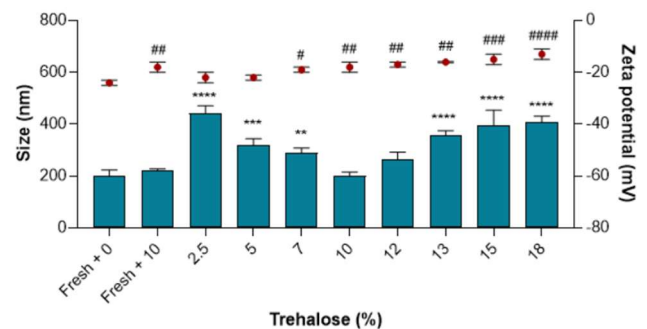
Fig. 2: Hydrodynamic diameter (blue bars) and Z-potential (red dots) of rehydrated hybrid NPs after freeze-drying in the presence of varying trehalose concentrations (2.5, 5, 7, 10, 12, 13, 15, and 18% (w/v)), compared to freshly prepared hybrid NPs (with 0% and 10% (w/v) trehalose).
