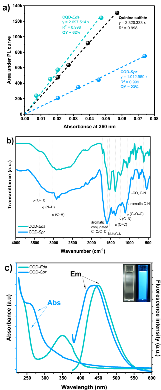
Fig. 1 (a) Quantum yield (QY), (b) FTIR spectra, and (c) UV–vis absorption and photoluminescence (PL) emission spectra (excitation at 360 nm) of CQD-Eda and CQD-Spr. Inset: photograph of the CQD-Eda aqueous solution under visible and UV irradiation
