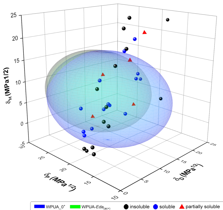
Fig. 5 Hansen solubility sphere calculated from the HSPs and R_0 values for WPUA-0 + (blue sphere) and WPUA-Eda (ac+) (green sphere). Blue circles, black circles, and red triangles represent soluble, insoluble, and partially soluble solvents, respectively, as listed in Table 6
