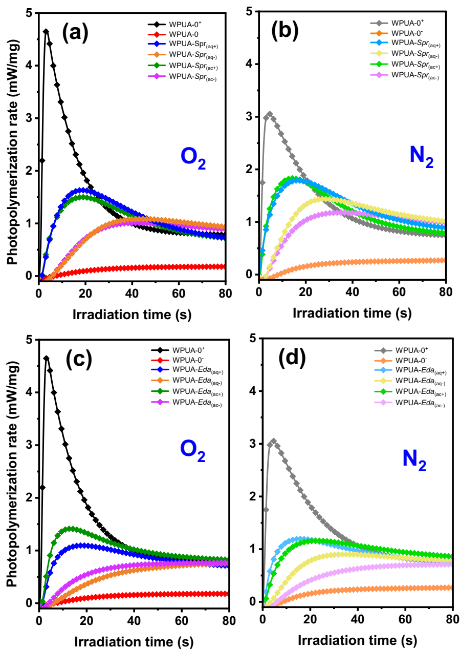
Fig. 3 (a–d) Photo-DSC thermograms and (e–h) C=C conversion ( \alpha ) as a function of irradiation time for WPUA-Spr and WPUA-Eda systems under inert ( N_2 ) and oxygen ( O_2 ) atmospheres
