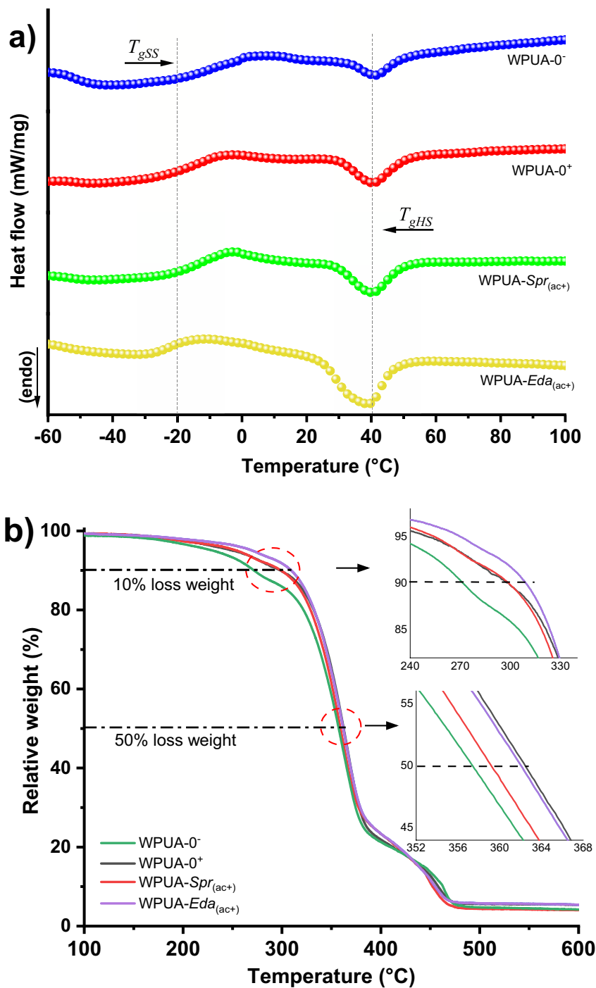
Fig. 4 (a) DSC and (b) TGA curves of cured neat WPUA and WPUA/CQDs nanocomposites
