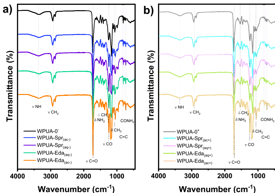
Fig. 2 FTIR spectra of the neat WPUA and WPUA/CQDs nanocomposites (a) before and (b) after UV curing
