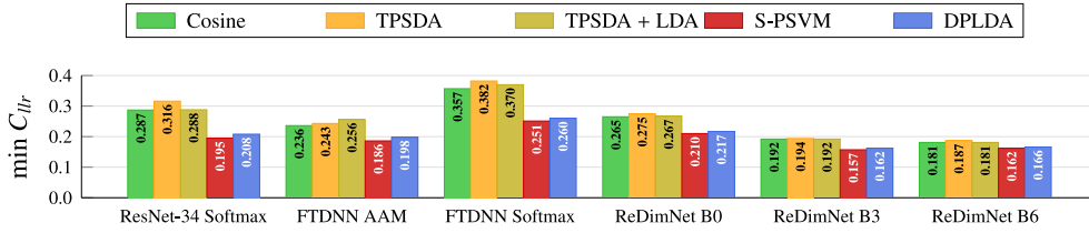
Fig. 9. Comparison of TPSDA and TPSDA with an additional LDA pre-processing step.
