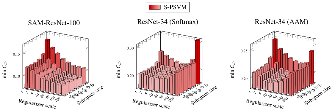
Fig. 12. S-PSVM results as a function of the speaker subspace dimension and the regularization scaling coefficient \lambda_S .
