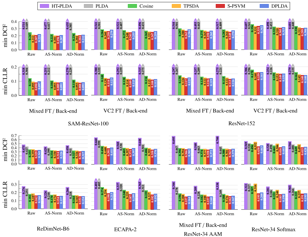
Fig. 14. Minimum DCF and minimum C_{IIr} for SAM-ResNet-100, ResNet-152, ReDimNet-B6, ECAPA-2 and ResNet-34 front-ends, without score normalization, with AS-norm and with AD-norm.
