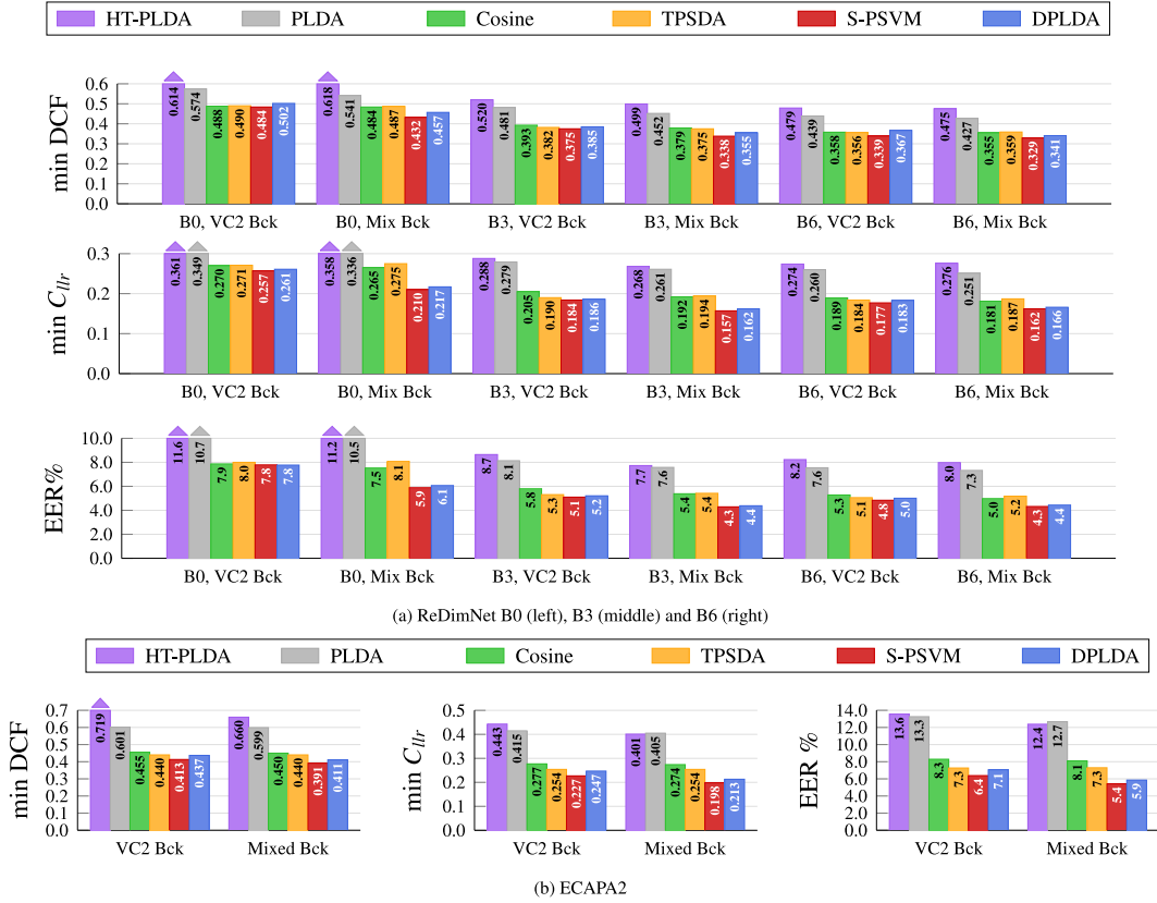
Fig. 4. Minimum DCF, minimum C_{lr} and EER % for different back-ends with off-the-shelf front-ends. For each back-end, we consider both models trained with VC2 (VC2 Bck) and Mixed CTS + VC2 (Mix Bck) data.
