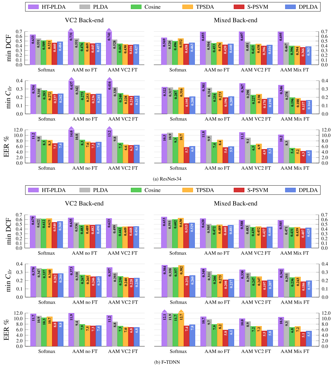
Fig. 3. Minimum DCF, minimum C_{lfr} and EER % for different back-ends with different front-ends. For each front-end, we consider models trained with Softmax, and models trained with AAM without (No FT), with VC2 (VC2 FT), and with CTS + VC2 (Mix FT) fine-tuning. As back-ends we consider both models trained with VC2 (VC2 Back-end) and CTS + VC2 (Mixed Back-end) data.
