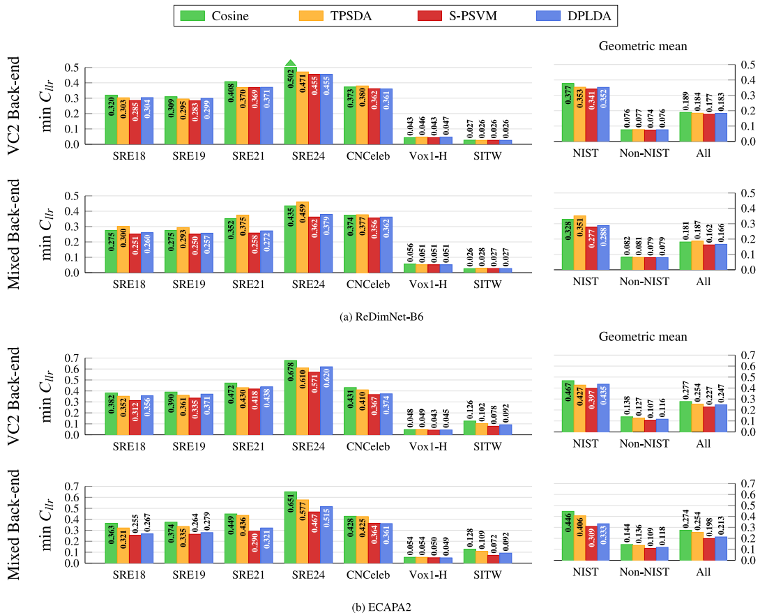
Fig. 6. Individual evaluation set results and corresponding geometric averages, ReDimNet-B6 and ECAPA2 off-the-shelf extractors.
