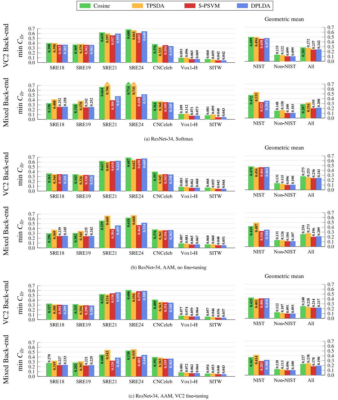
Fig. 7. Individual evaluation set results, and corresponding geometric averages, for ResNet-34 front-ends trained with different losses and fine-tuning strategies.
