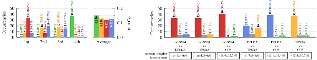
(c) Summary of individual evaluation set results corresponding to the ResNet-152 and SAM-ResNet-100 configurations in Figure 5, for a total of 42 individual benchmarks.
