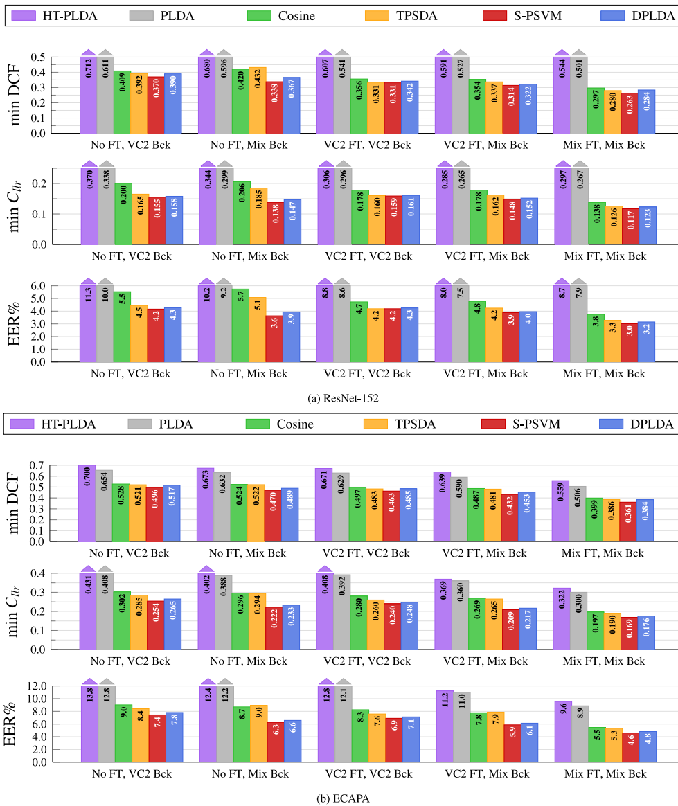
Fig. 2. Minimum DCF, minimum C_{lr} and EER % for different back-ends with different front-ends. For each front-end, we consider both models without fine-tuning (No FT), and models fine-tuned with VC2 (VC2 FT) and CTS + VC2 (Mix FT) data. As back-ends we consider both models trained with VC2 (VC2 Bck) and CTS + VC2 (Mix Bck) data.
