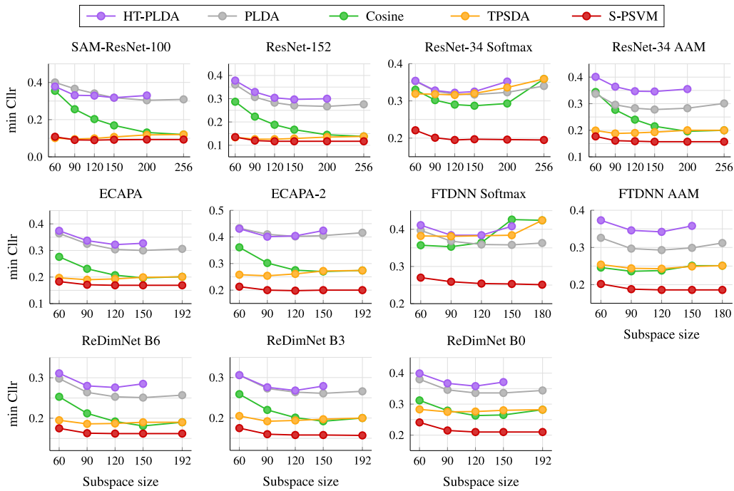
Fig. 8. Results for different front-end/back-end combinations with varying speaker subspace sizes. The SAM-ResNet-100, ResNet-152, ResNet-34 AAM, FTDNN AAM, and ECAPA models employ CTS + VC2 fine-tuning. All back-ends are trained with CTS + VC2 data.
