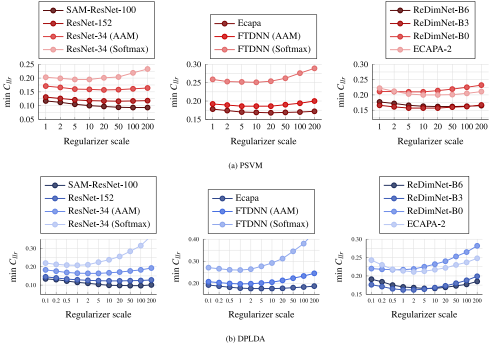
Fig. 11. Average minimum C_{lr} on the evaluation sets as a function of the PSVM and DPLDA regularization scaling coefficient \lambda_s .
