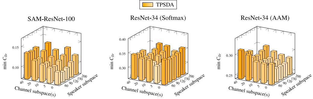
Fig. 10. TPSDA results as a function of the speaker and channel subspace(s) dimension.
