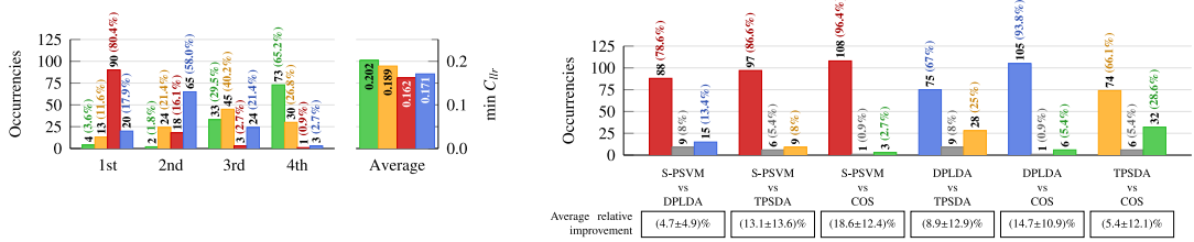
(b) Summary of individual evaluation set results corresponding to the front-end / back-end combinations in Figures 5 to 7, for a total of 112 individual benchmarks.
