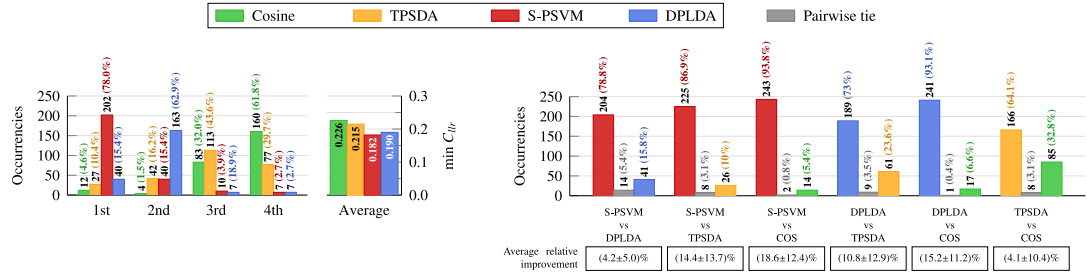
(a) Summary of individual evaluation set results corresponding to all analyzed front-end / back-end combinations, described in Figures 1 to 4, for a total of 259 individual benchmarks.
