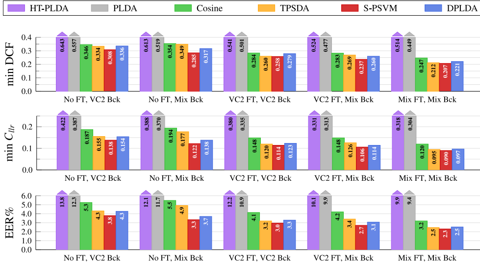
Fig. 1. Minimum DCF, minimum C_{illr} and EER % for different back-ends with SAM-ResNet-100 front-ends, without fine-tuning (No FT), fine-tuned with VC2 (VC2 FT), and with CTS + VC2 (Mix FT) data. As back-ends we consider both models trained with VC2 (VC2 Bck) and CTS + VC2 (Mix Bck) data.
