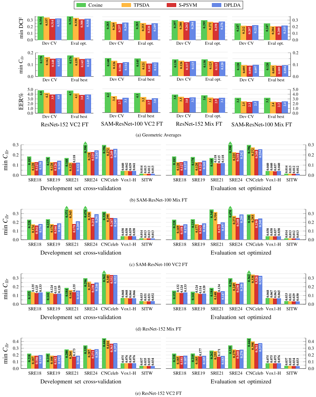
Fig. 13. Effects of per-dataset hyper-parameter tuning. Development set cross-validation (Dev CV): hyper-parameters are selected by cross-validation optimizing the average development sets results. Evaluation set optimized (Eval best): for each evaluation set the hyper-parameters that provide the best results are employed.
