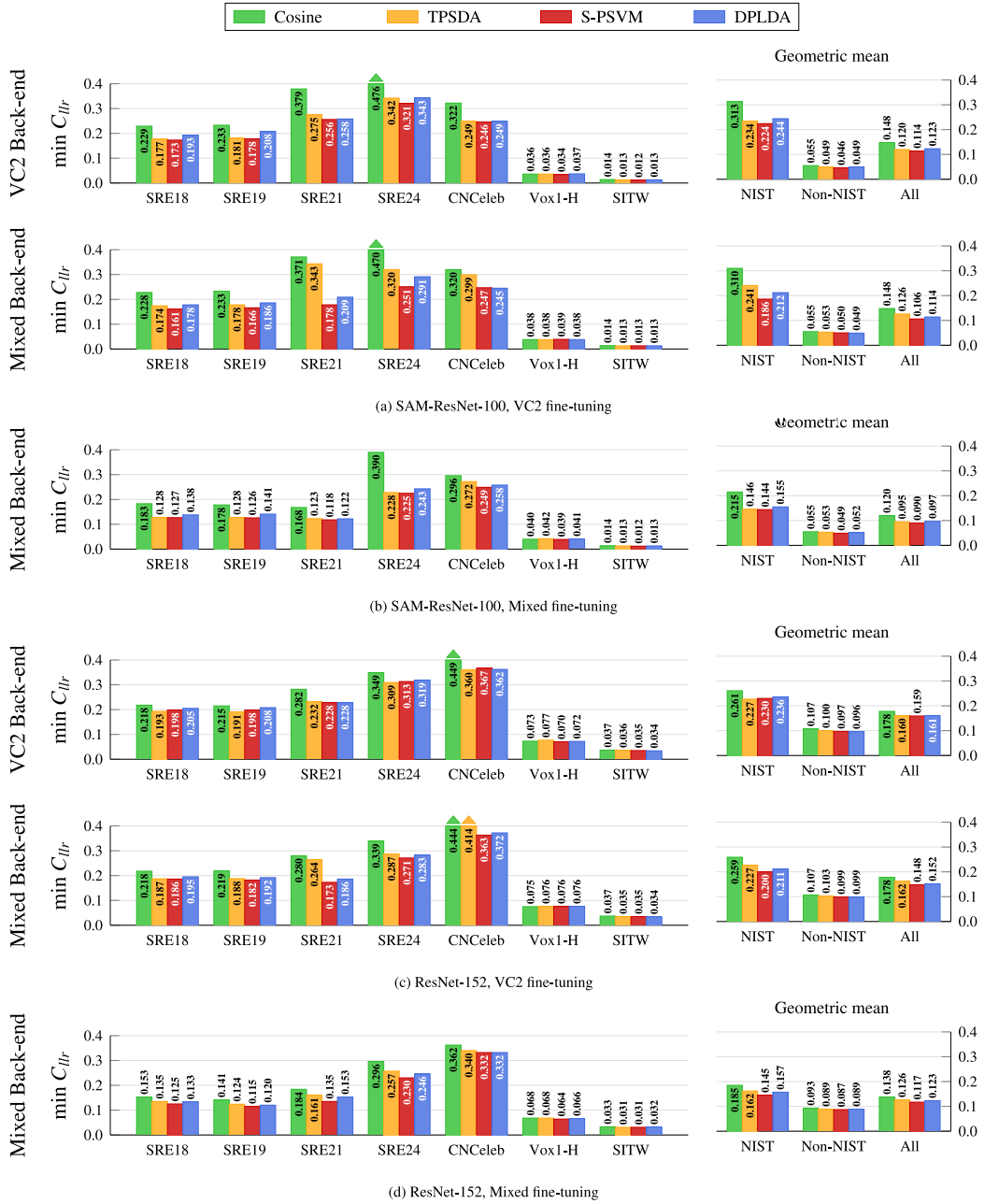
Fig. 5. Individual evaluation set results and corresponding geometric averages, SAM-ResNet-100 and ResNet-152.
