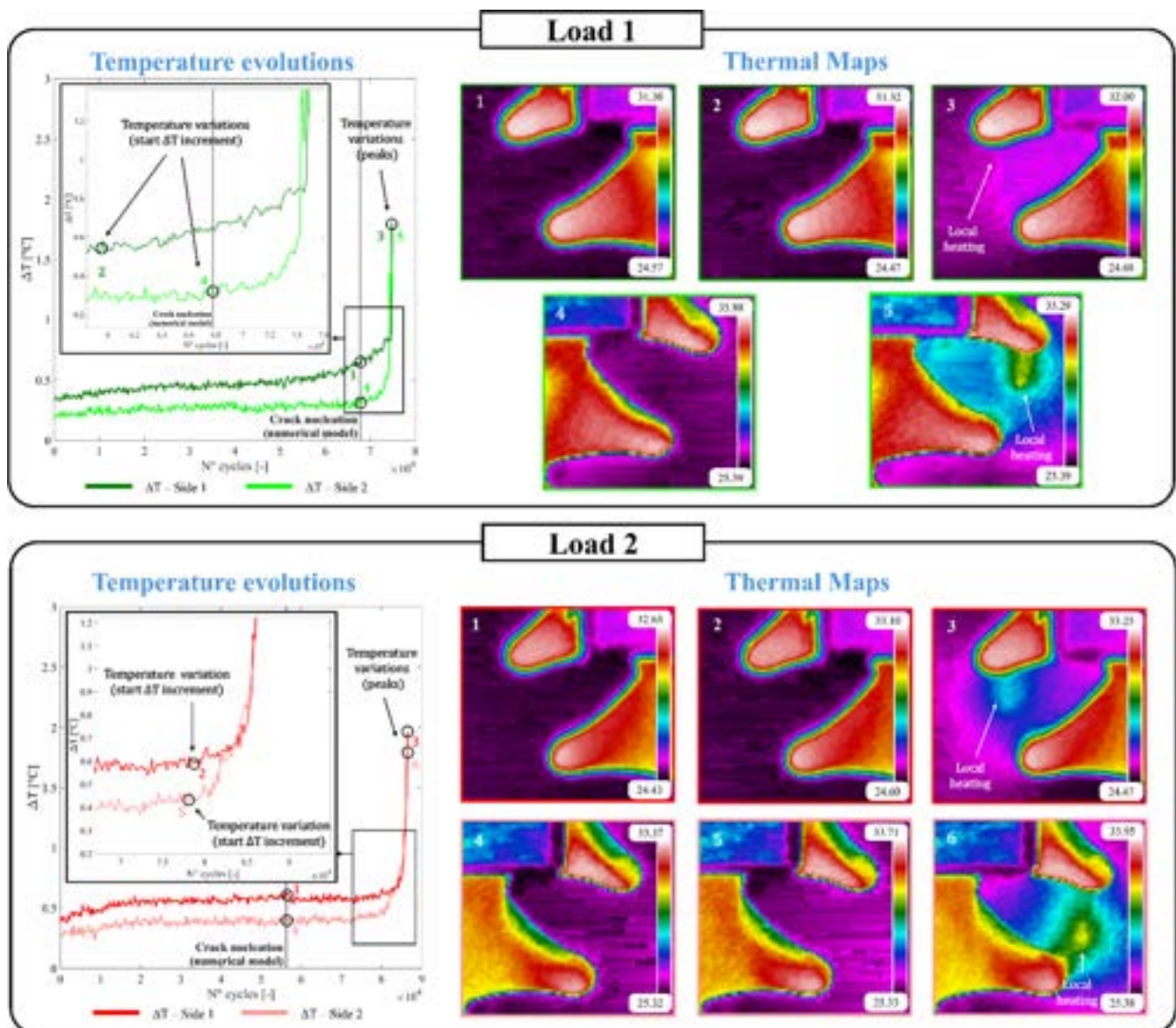
FIGURE 8 | Temperature evolutions and thermal maps for Gear 2. [Colour figure can be viewed at wileyonlinelibrary.com ]
