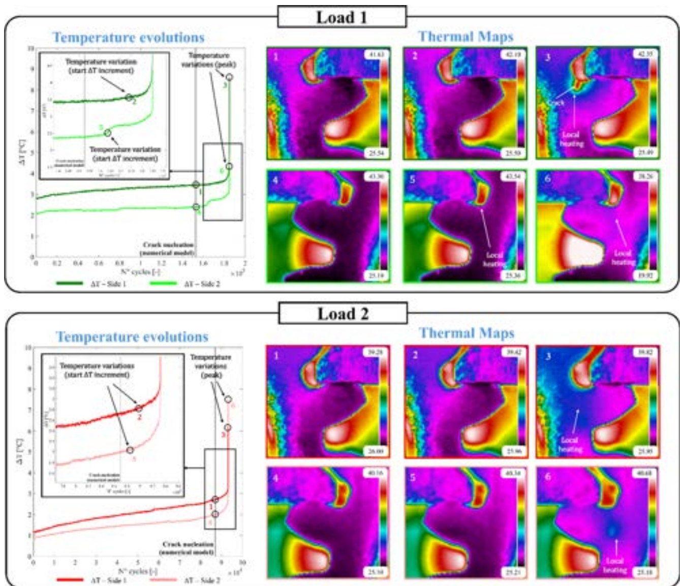
FIGURE 9 | Temperature evolutions and thermal maps for Gear 3. [Colour figure can be viewed at wileyonlinelibrary.com ]
