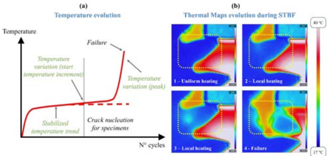
FIGURE 4 | Thermal dissipations: temperature evolution variations (a) and local heating over thermal maps for gears (b). [Colour figure can be viewed at wileyonlinelibrary.com ]
