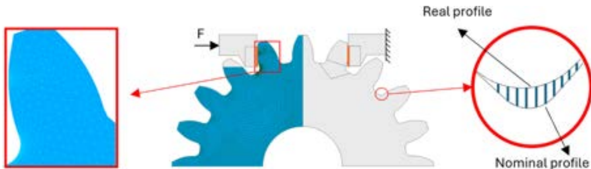
FIGURE 6 | Finite element model definition. [Colour figure can be viewed at wileyonlinelibrary.com ]
