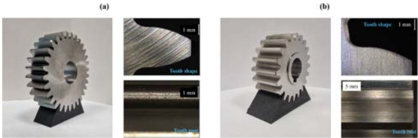
FIGURE 2 | Gears samples: (a) Gear 1 and Gear 2; (b) Gear 3. [Colour figure can be viewed at wileyonlinelibrary.com ]
