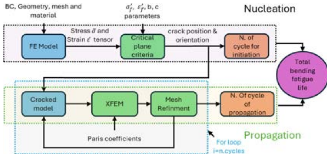
FIGURE 5 | Numerical algorithm. [Colour figure can be viewed at wileyonlinelibrary.com ]
