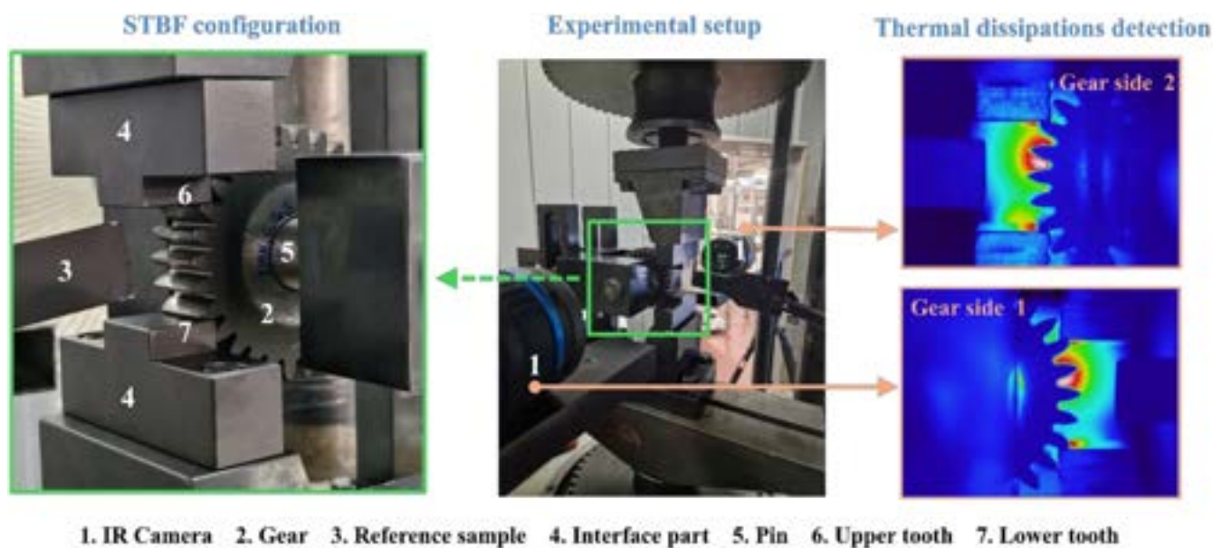
FIGURE 3 | Experimental setup during the STBF tests. [Colour figure can be viewed at wileyonlinelibrary.com ]
