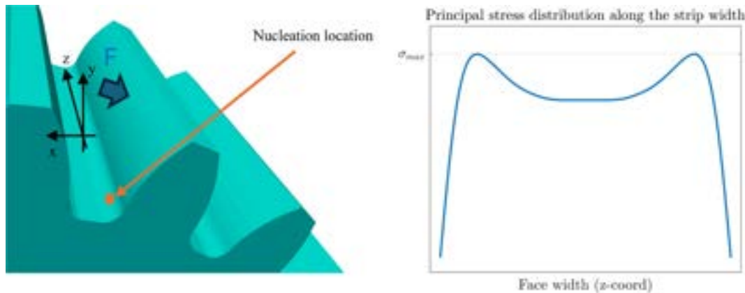
FIGURE 1 | Stress distribution at the tooth root. [Colour figure can be viewed at wileyonlinelibrary.com ]
