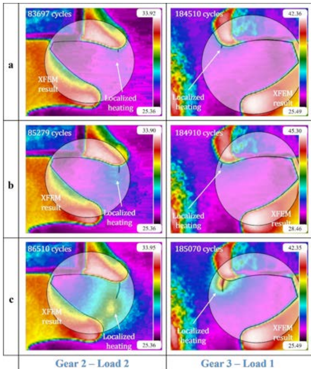
FIGURE 10 | Crack path comparison before failure. [Colour figure can be viewed at wileyonlinelibrary.com ]
