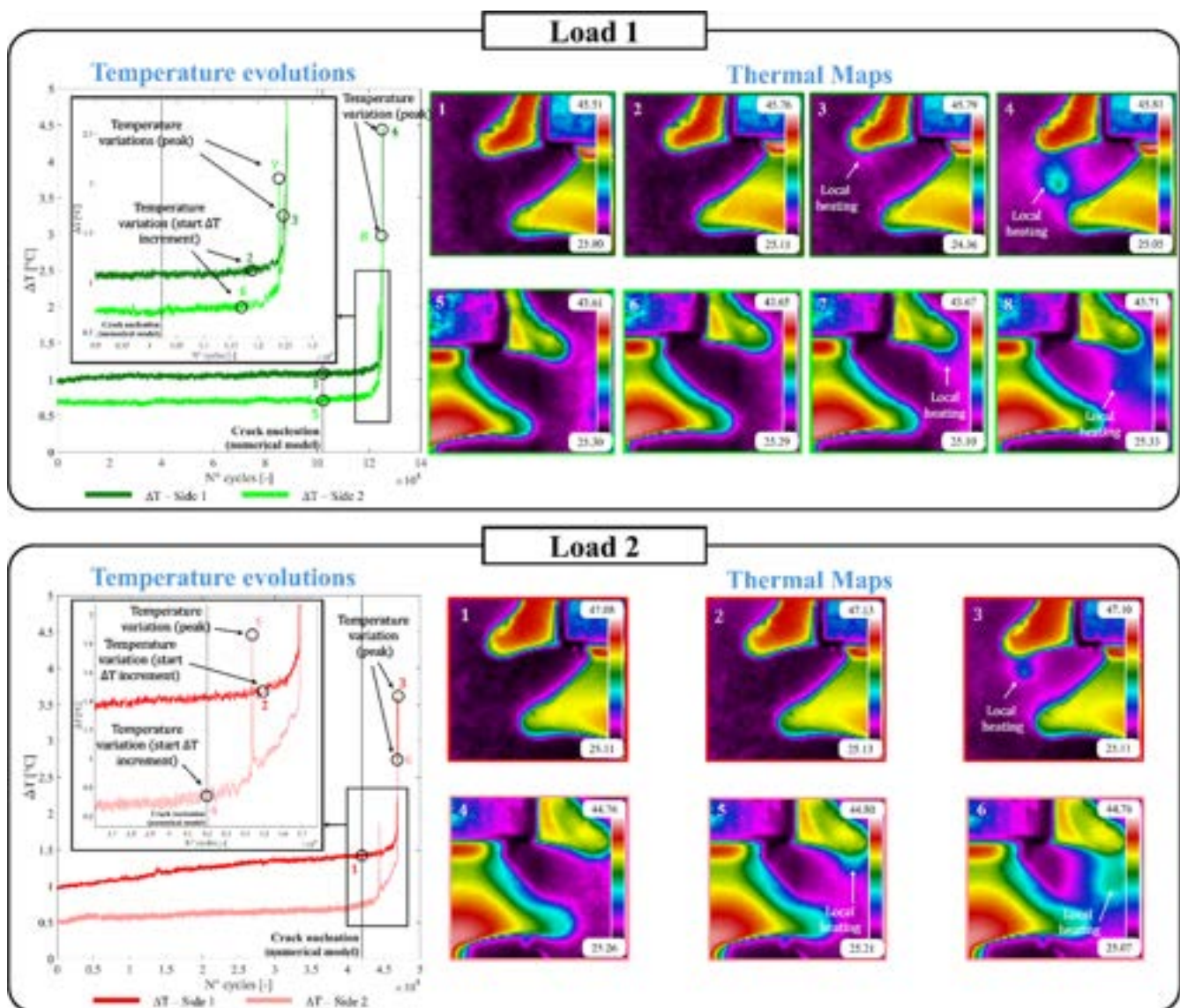
FIGURE 7 | Temperature evolution and thermal maps for Gear 1. [Colour figure can be viewed at wileyonlinelibrary.com ]
