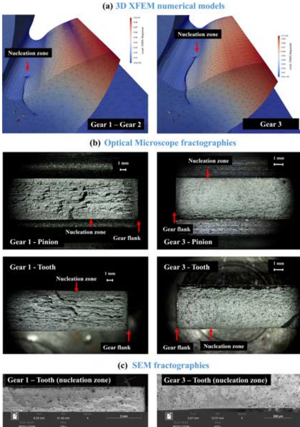
FIGURE 11 | Crack process comparison: numerical results and fractographic analysis. [Colour figure can be viewed at wileyonlinelibrary.com ]
