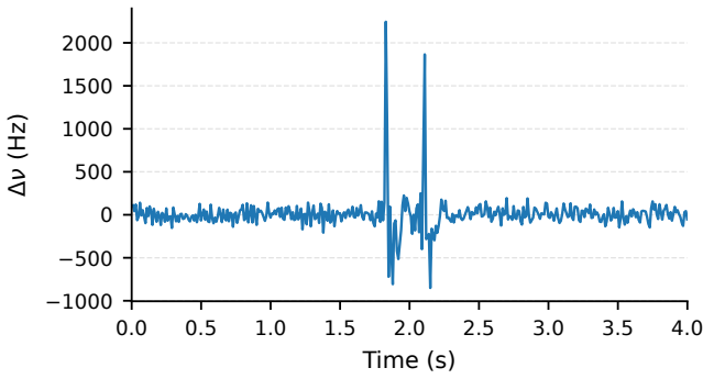
Fig. 2. Interferometric phase-derived frequency-deviation waveform recorded during a vehicle-passage event on the AP-TE link.
