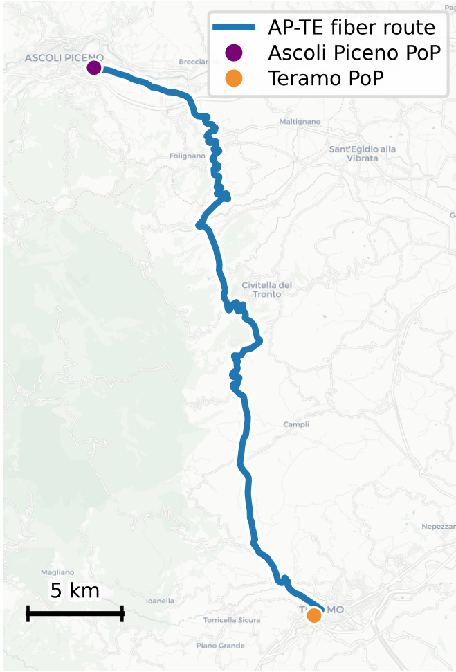
Fig. 1. Geographical layout of the AP-TE fiber route between the Ascoli Piceno and Teramo points of presence.
