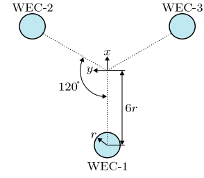
Fig. 2. WEC array composed of three point absorbers considered in the study.
