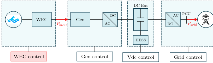
Fig. 1. Integrated W2G modelling and control framework for the WEC array.
