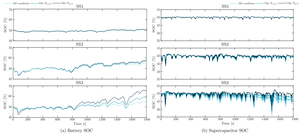
Fig. 6. Battery (a) and supercapacitor (b) state of charge for the three different sea states (SS1, SS2, SS3) in the three optimal conditions (Grid Opt, Mech Opt, IM).
