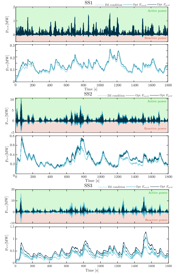
Fig. 5. Mechanical power P_{\text{mech}} and grid power P_{\text{grid}} profiles for the three controller configurations considered across the sea states (SS1, SS2, SS3): IM tuning, maximum mechanical energy, and maximum grid energy.
