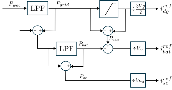
Fig. 3. Energy management system framework.
