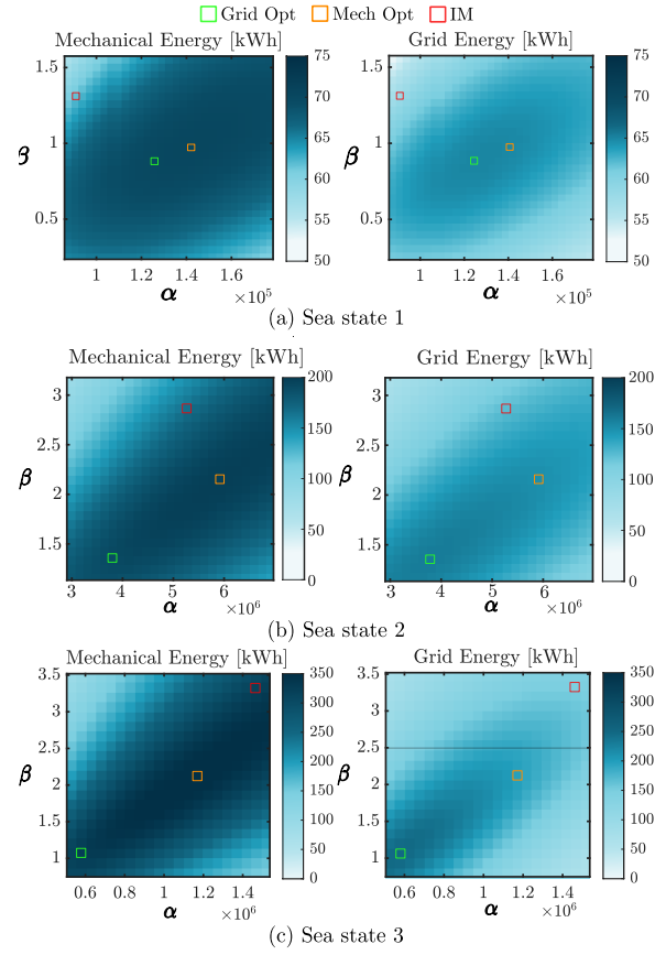
Fig. 4. Heatmap comparison of E_{mech} and E_{grid} versus \alpha and \beta for the three sea states (SS1, SS2, SS3), with highlighted the three optimal combinations: IM, Mech Opt, Grid Opt.
