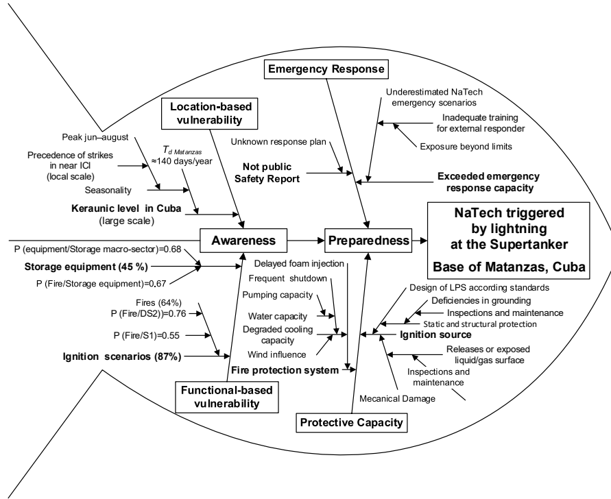
Figure 3: Fishbone Diagram of lightning-triggered NaTech accident at the Matanzas Supertanker Base.
