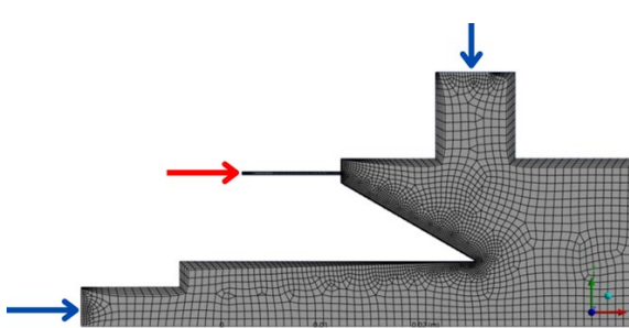
Figure 6: Hyd. burner - Low fidelity mesh (40k nodes)
