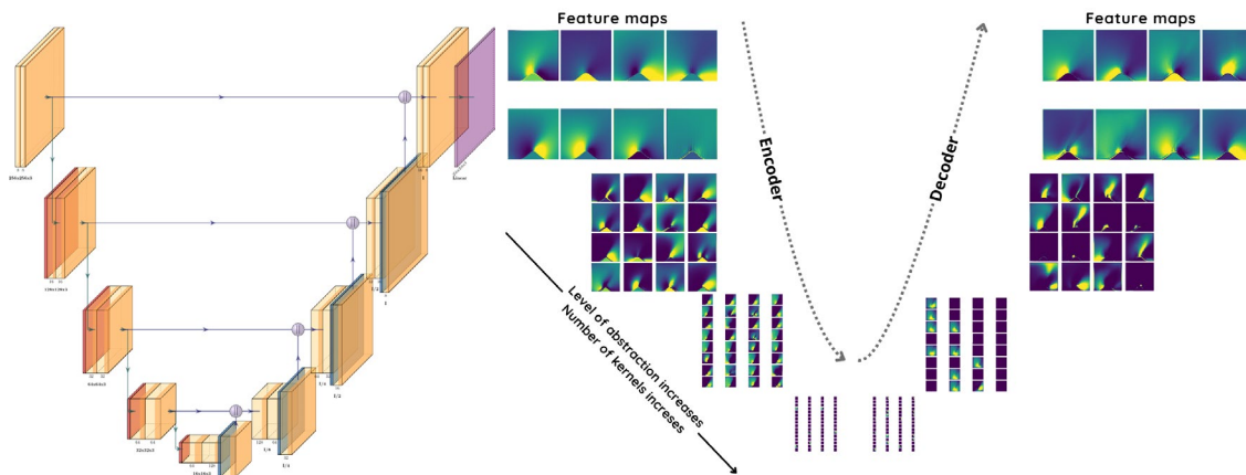
Figure 1 : The U-net structure.
