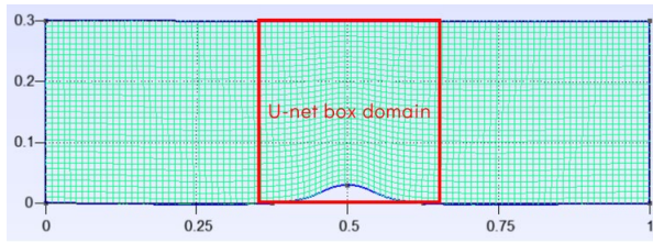
Figure 4 : Bump - low fidelity mesh (3k nodes)
