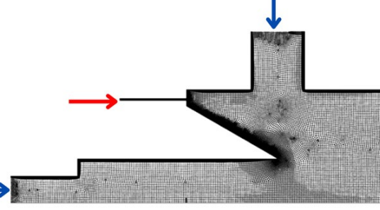
Figure 7 : Hyd. burner - high fidelity mesh (200k nodes)
