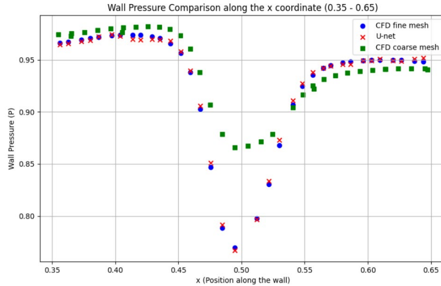
Figure 8 : Reconstruction of the high-fidelity wall pressure in the bump-in-a-duct configuration.
