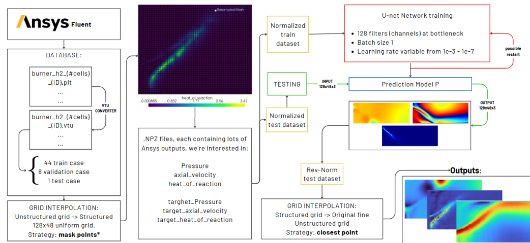
Figure 3 : The workflow of the framework
