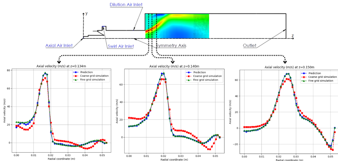
Figure 9 : Reconstruction of the high-fidelity velocity field for the hydrogen burner case. Radial profiles are shown at three different axial positions.
