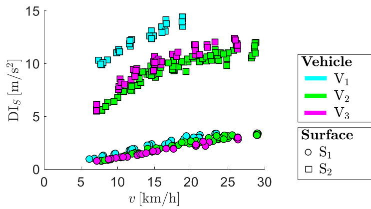
Figure 8. Discomfort index evaluated at the hand-steering interface for the three vehicles on asphalt and pavé surfaces for different vehicle velocities.
