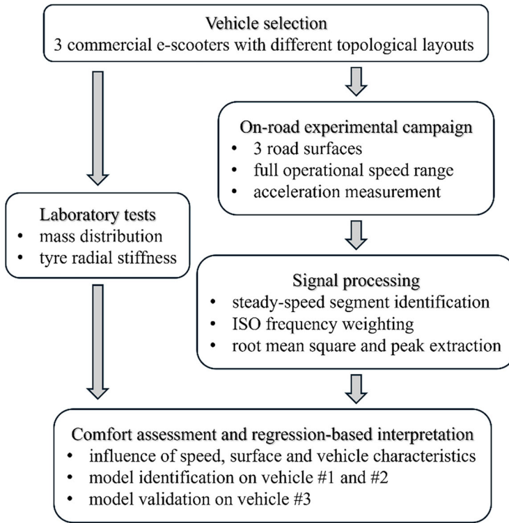
Figure 1. Overview of the proposed framework for e-scooter ride comfort assessment, linking vehicle characterisation, on-road vibration measurements, ISO-based signal processing and regression-based interpretation.
