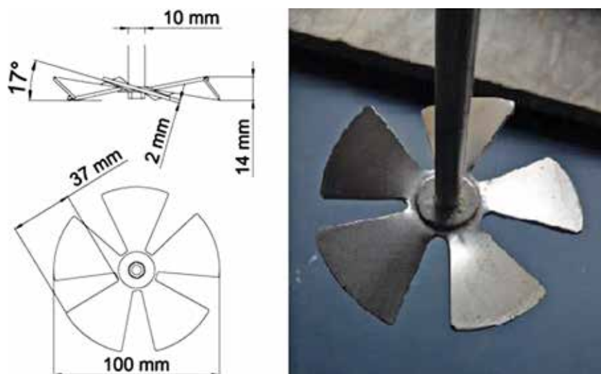
Fig. 3 – Scheme and photo of the used impeller (Todaro et al. , 2019).
