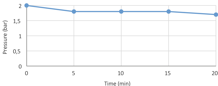
Fig. 8 – Pressure holding capacity of the cake over time.
