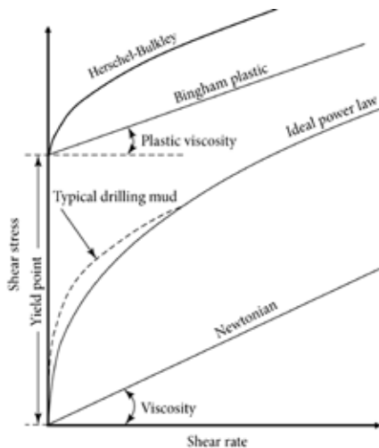
Fig. 4 – Consistency chart for Newtonian and Bingham fluids (modified from Caenn et al. 2011).
