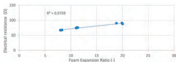
Figure 6. Results of tests at constant FER.
