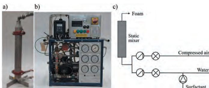
Figure 1. Static mixer (a), foam generator used (b), scheme of the foam generator (c).
