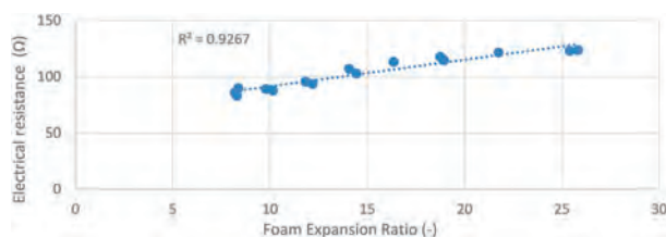
Figure 5. Results of tests with progressive variation of FER.
