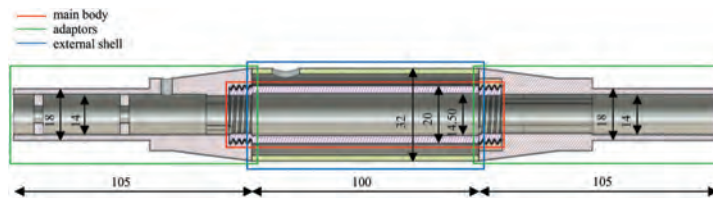
Figure 2. Section view of the prototype showing the main dimensions expressed in mm.
