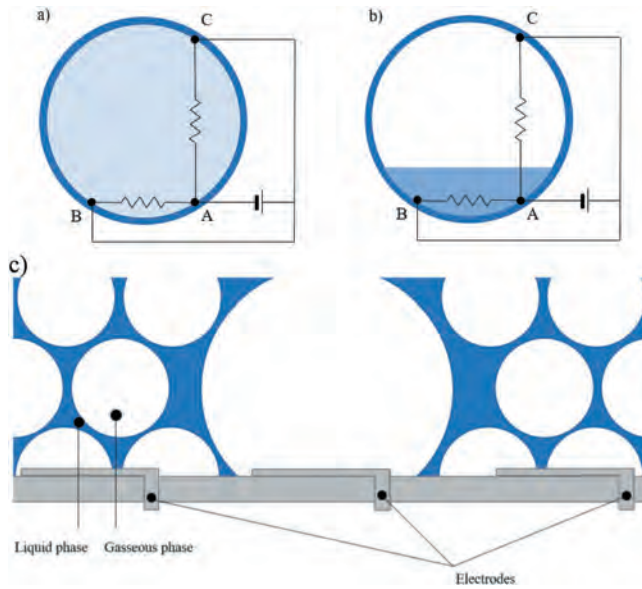
Figure 3. Position of the electrodes in the cross-section of the device. a) In homogeneous foam, both pairs of electrodes measure the same resistivity. b) In the presence of lamination, different resistivities are detected. c) Positioning of electrodes to avoid spikes in resistivity due to single bubbles.
