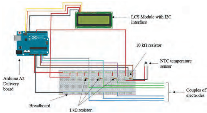
Figure 4. Wiring of the electrical circuit.
