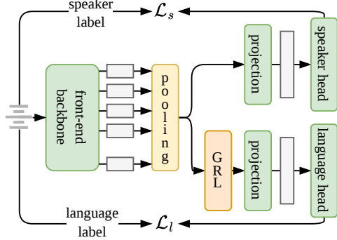
Figure 1: A scheme of incorporating a gradient reversal layer (GRL) into an embedding extractor with a language classifier.
