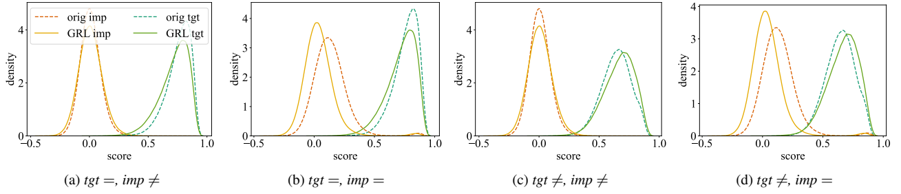
Figure 2: Score distributions for tv26_dev sublists obtained with w2v-BERT 2.0 w/ MFA (w/ or w/o GRL) and cosine similarity scoring.
