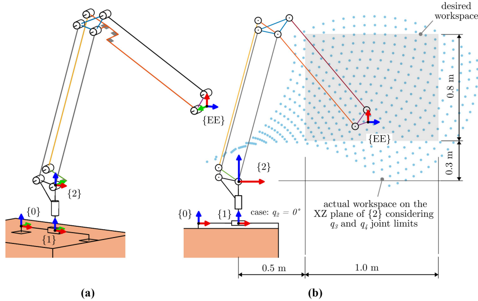
Figure 6 Robotic arm scaled functional scheme: (a) 3D representation and (b) 2D representation with q_2 = 0^\circ . The gray rectangle represents the desired workspace, while the blue dots represent the actual workspace section on the XZ plane of \{2\} considering q_3 and q_4 joint limits
