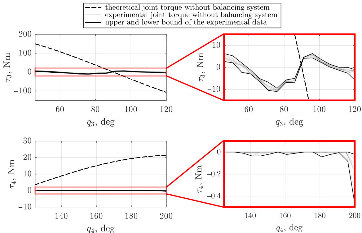
Figure 14 Measured joint torques to balance the system within the range of motion of the robot, zoomed sections of the plots are highlighted with red lines
