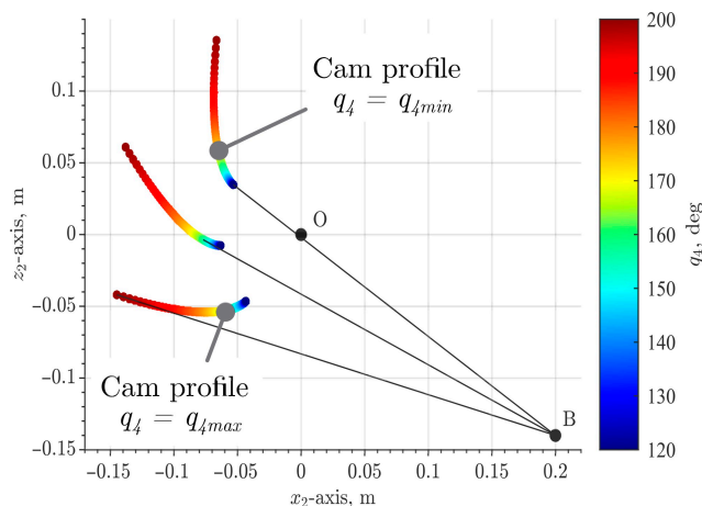
Figure 11 Result of the cam synthesis procedure
