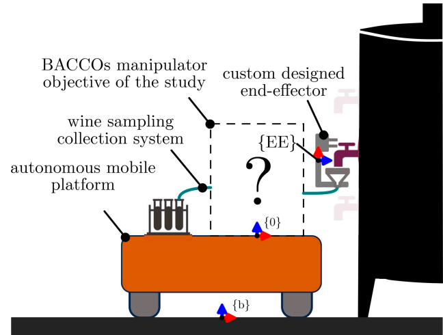
Figure 1 BACCOS concept and reference frames definition: \{b\} base platform reference frame, \{0\} BACCOS base reference frame and \{EE\} end-effector reference frame
