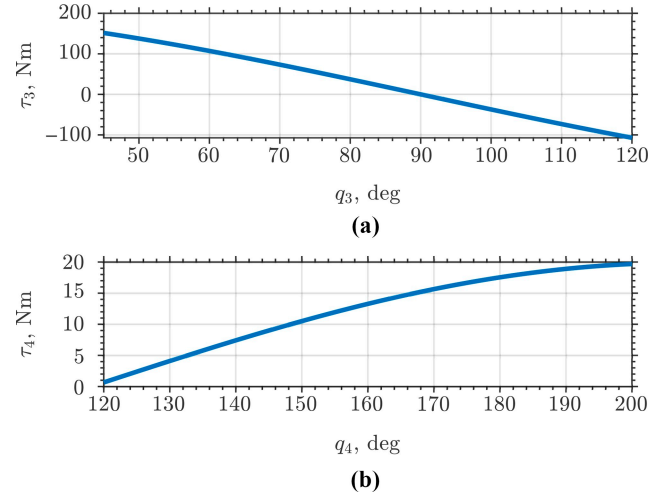
Figure 8 Torques (a) \tau_3 and (b) \tau_4 to compensate the gravity forces acting on the double-parallelogram mechanism
