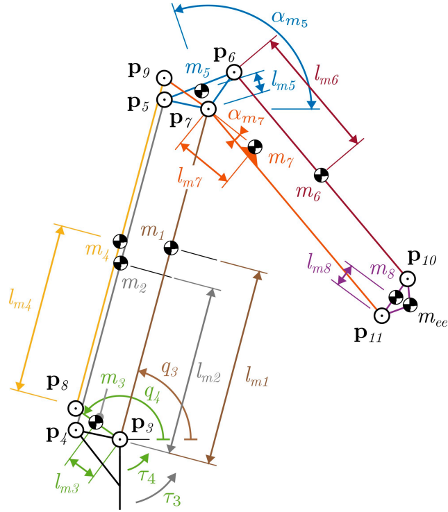
Figure 7 Double-parallelogram planar mechanism functional scheme: definition of the centers of gravity of all links
