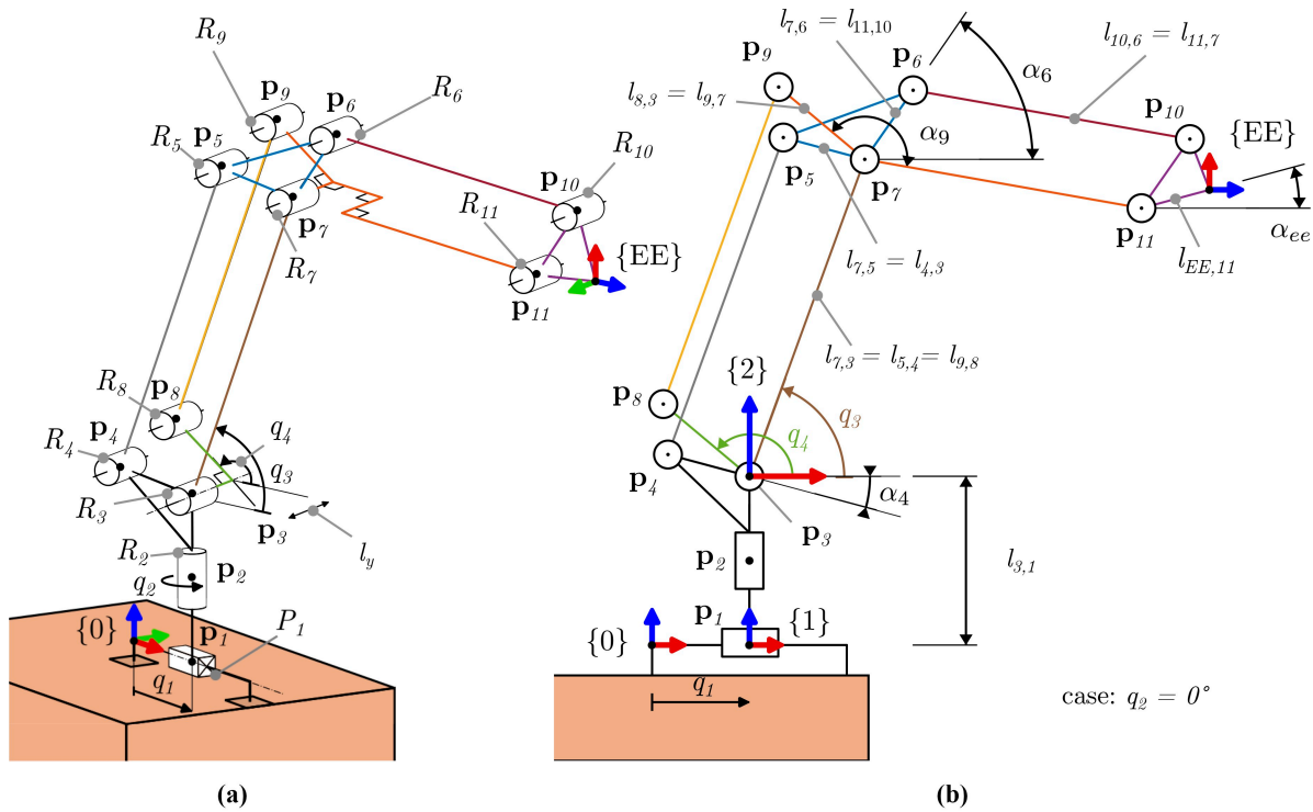
Figure 3 Robotic arm functional scheme: (a) 3D representation and (b) 2D representation with q_2 = 0^\circ
