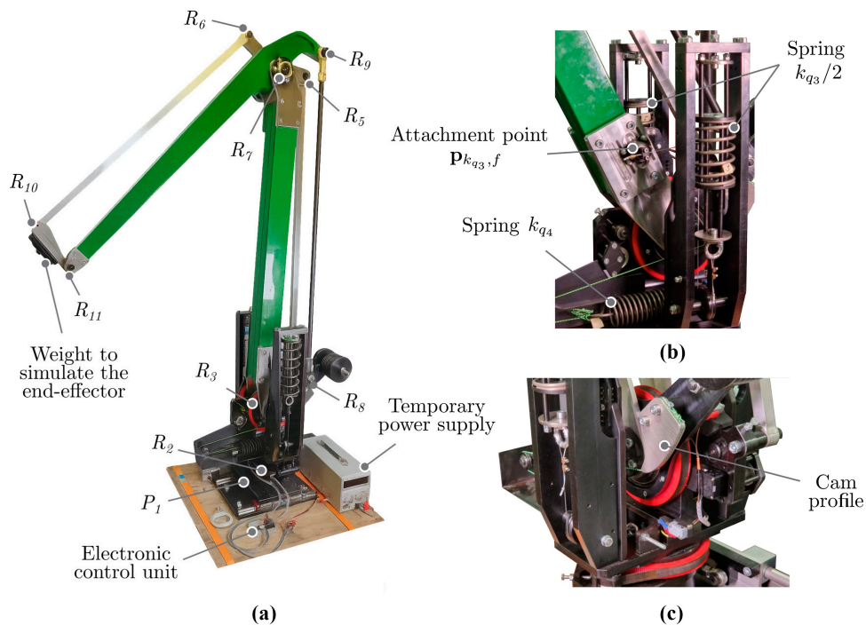
Figure 13 BACCOS prototype without safety covers on the balancing systems: (a) 3D view; (b) spring-wire balancing system; and (c) spring-wire-cam balancing system
