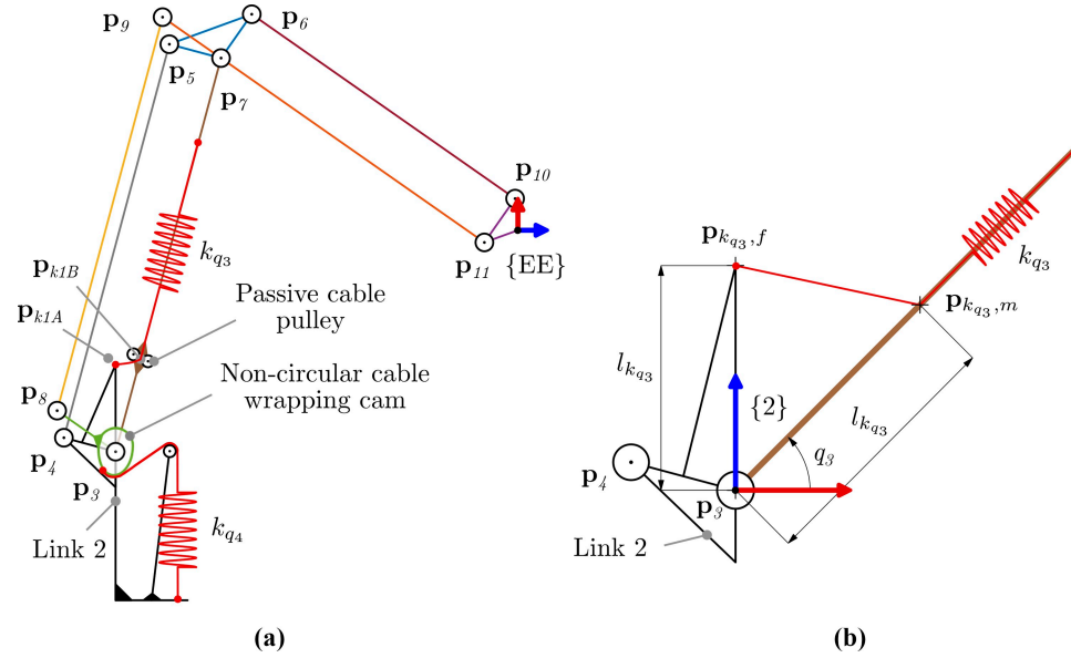
Figure 9 Functional schemes: (a) double-parallelogram planar mechanism with balancing systems and (b) details of the spring-wire balancing system used to obtain the gravity compensation on q_3
