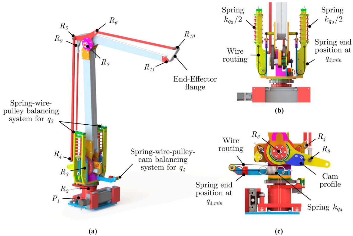
Figure 12 CAD view of BACCOS prototype without safety covers on the balancing systems: (a) 3D view; (b) spring-wire balancing system details; and (c) spring-wire-cam balancing system details
