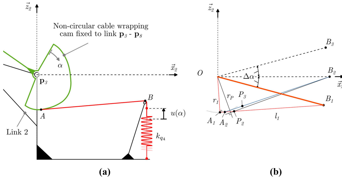
Figure 10 Functional schemes: (a) spring-wire-cam system to balance the degree-of-freedom described by the variable q_4 and (b) graphic method for cam synthesis and nomenclature definition
