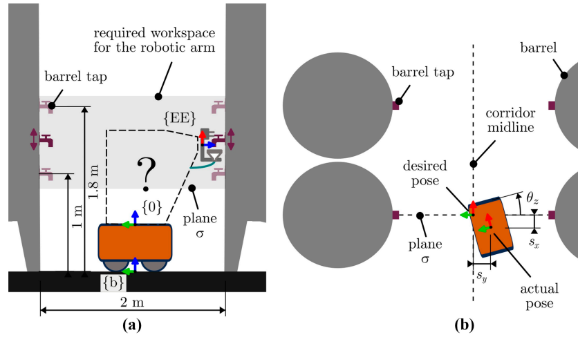
Figure 2 (a) Workspace definition: corridor and barrel taps and (b) possible pose errors of the mobile base
