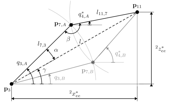
Figure 5 Geometric problem equivalent to the system of equation (10)
