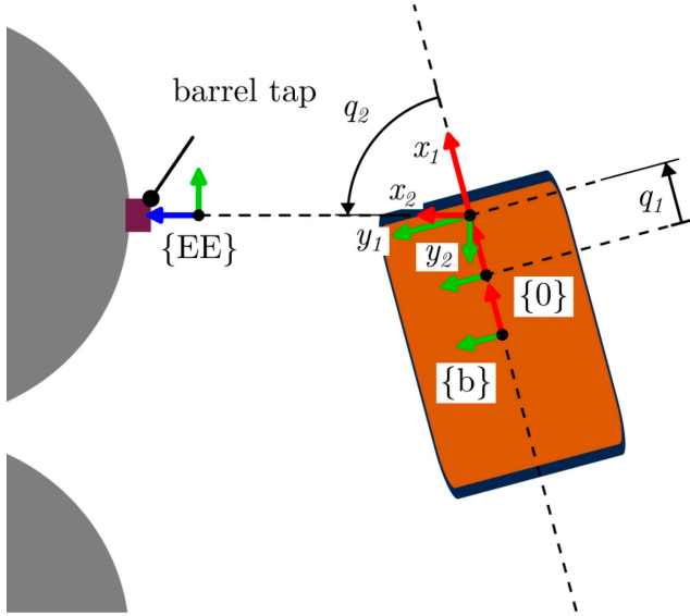
Figure 4 Robotic system approaching a barrel tap: top view reference frames definition
