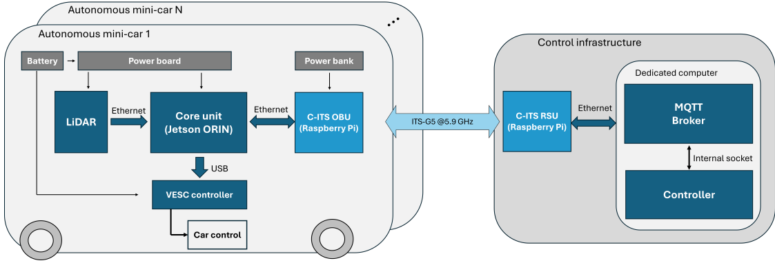
Fig. 1: Testbed architecture.
