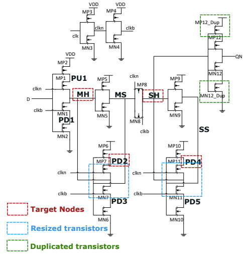
Fig. 4: Transistor-level schematic of the SET hardened DFF proposed in [21].
