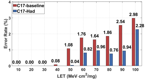
Fig. 8: SET error-rate comparison between the baseline and SH implementations of the C17 benchmark.
