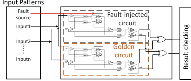
Fig. 7: The developed test setup circuit.
