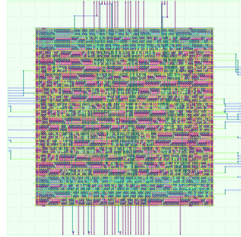
Fig. 5: The physical layout of the proposed SH-BLE.
