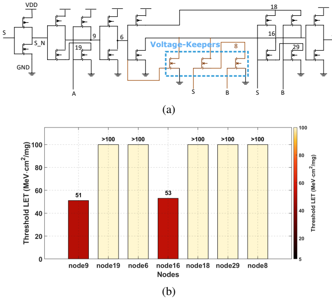
Fig. 3: Proposed SH 2:1 MUX: (a) transistor-level schematic with conditional voltage keepers and (b) threshold-LET values of its internal nodes.
