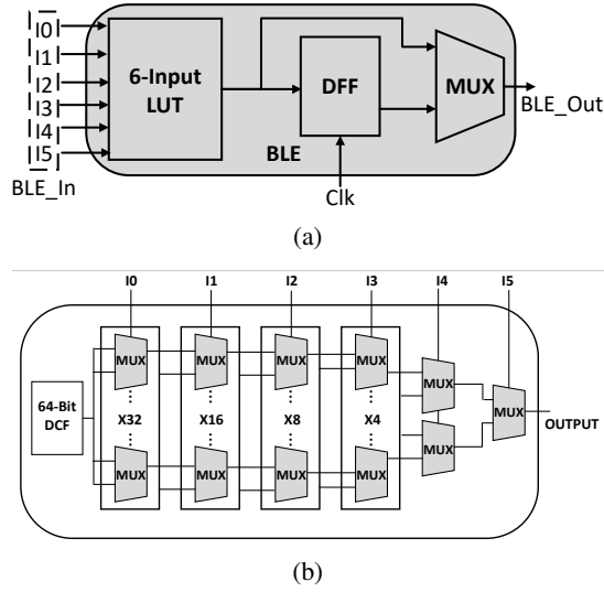
Fig. 1: The architecture of the BLE (a) and the 6-input LUT (b).
