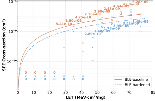
Fig. 6: Estimated SET cross sections of the baseline and proposed SH-BLEs with 95% Clopper–Pearson confidence intervals.
