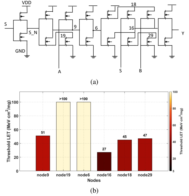
Fig. 2: Baseline 2:1 MUX: (a) transistor-level schematic and (b) threshold-LET values of its internal nodes.
