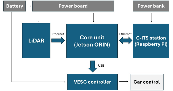
Fig. 2: Block scheme of the hardware components.
