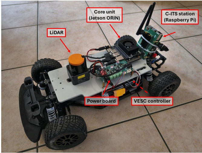
Fig. 1: Cooperative, connected and automated mini-car, equipped with the low-cost OBU.
