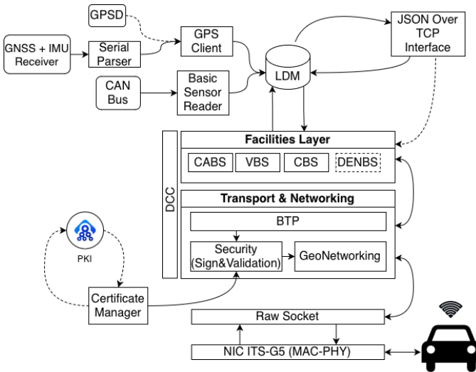
Fig. 3: Block diagram of the Oscar stack and its main functional components
