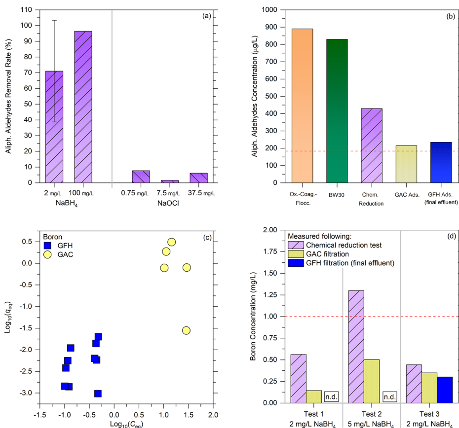
Fig. 4 | Behavior of aliphatic aldehydes and boron during selected treatment steps. a Percentage removal of aliphatic aldehydes in batch chemical reduction tests using two different concentrations of sodium borohydride ( \text{NaBH}_4 ). For the 2 mg/L \text{NaBH}_4 test (corresponding to 0.57 mg/L boron), the bar represents the mean \pm one standard deviation from two independent experiments. Transformation was calculated as \left(1 - \frac{c_{\text{FIN}}}{c_0}\right) \times 100 , where c_0 and c_{\text{FIN}} are the initial and final concentrations, respectively. b Aliphatic aldehyde concentrations measured after sequential treatment steps; the horizontal red dashed line indicates the target concentration limit in the final effluent of the treatment train. c Adsorption behavior of boron on vegetal granular activated carbon (GAC; yellow circles) and granular ferric oxide-hydroxide (GFH; blue squares). d Boron concentrations measured across different treatment steps for three independent tests using \text{NaBH}_4 . The horizontal red dashed line again indicates the concentration limit in the final effluent. “n.d.” indicates that no data were determined for that specific case.
