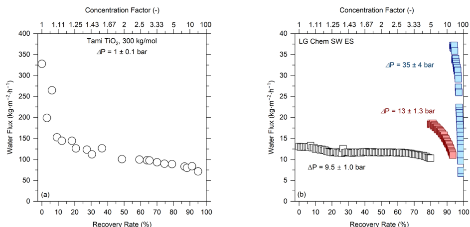
Fig. 6 | Membrane performance in terms of water flux from pilot-scale batch experiments. a Water flux (kgMH) as a function of recovery rate for the ultrafiltration (UF) unit, using a Tami TiO 2 membrane with a molecular weight cutoff of 300 kg/mol. The applied hydraulic pressure difference, \Delta P , is indicated in the panel. b Water flux (kgMH) as a function of recovery rate for the three stages of reverse osmosis (RO), each using different operating pressures and the same membrane type, as indicated. The top axis reports the corresponding concentration factor, enabling estimation of solute concentration buildup along the treatment process.
