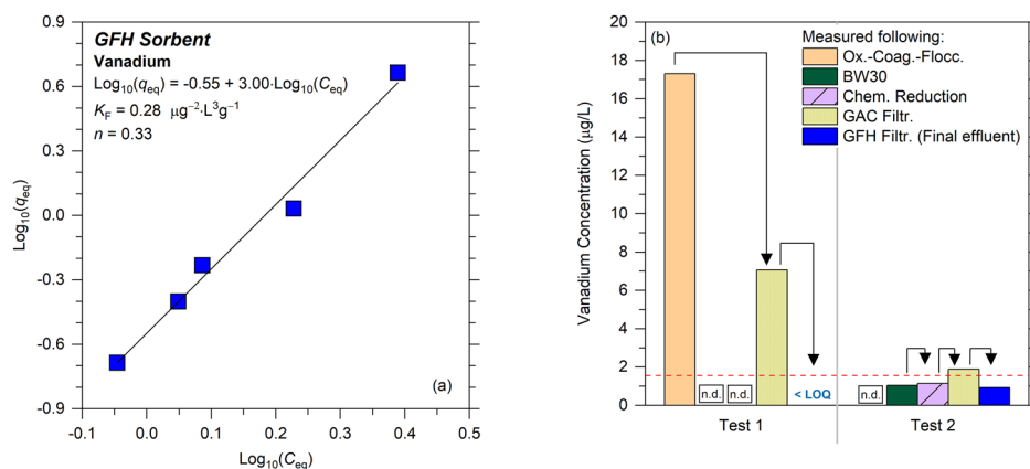
Fig. 5 | Behavior of vanadium during selected treatment steps. a Adsorption isotherm of vanadium onto granular ferric hydroxide (GFH) measured at room temperature. The plot displays experimental data (blue squares) and the corresponding Freundlich model fit (black line), expressed as q_{eq} = K_F C_{eq}^n , and linearized as \text{Log}_{10} q_{eq} = \text{Log}_{10} K_F + \frac{1}{n} \text{Log}_{10} C_{eq} . The estimated Freundlich parameters, K_F and n , as well as the linearized equation, are reported in the graph. b Vanadium concentrations measured after sequential treatment steps in two independent tests. The red dashed horizontal line indicates the target concentration limit in the final effluent of the treatment train. “n.d.” indicates “not determined”; “< LOQ” denotes concentrations below the limit of quantification.
