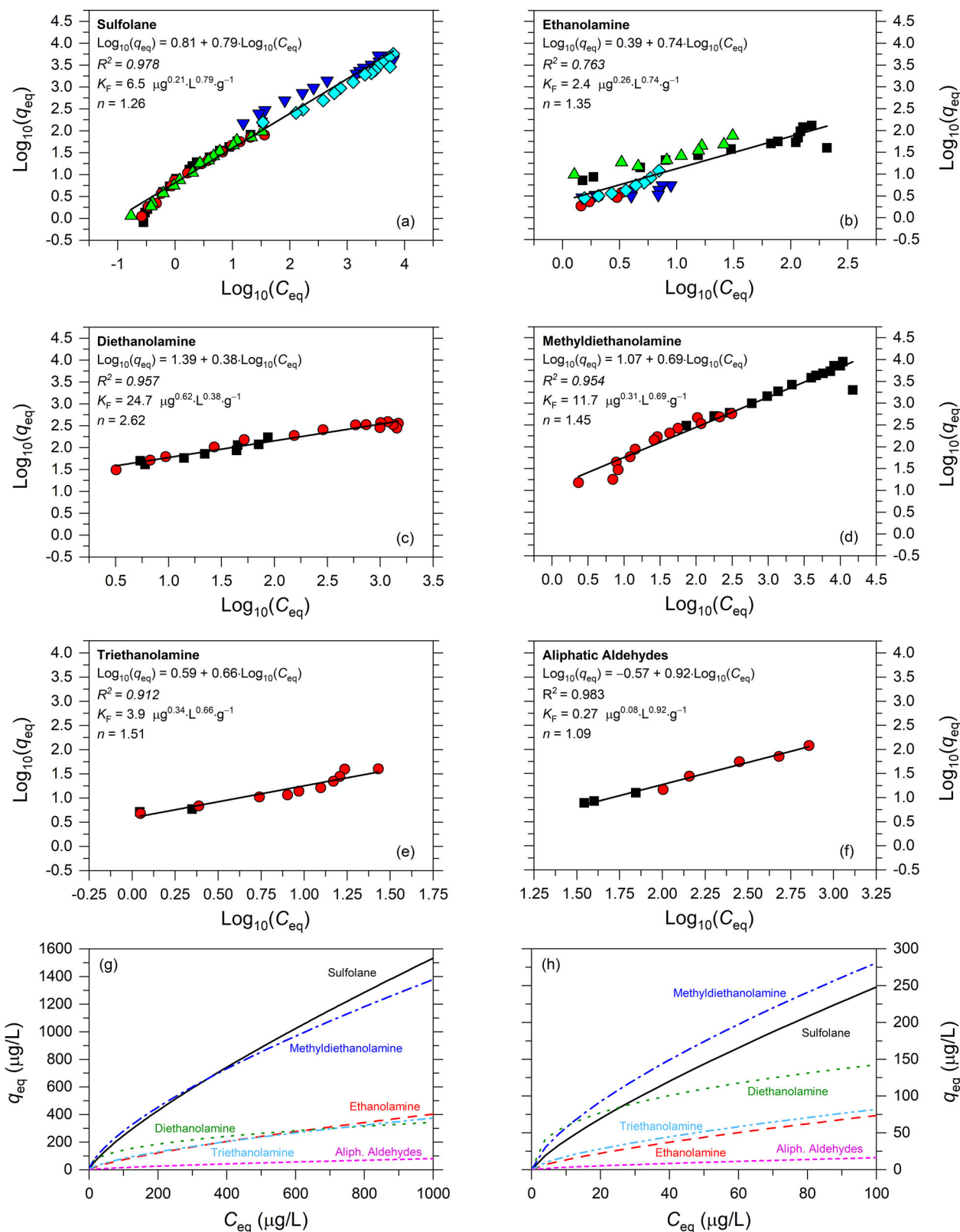
Fig. 2 | Adsorption isotherms of selected compounds on vegetal granular activated carbon (GAC). a–f show experimental data (symbols) and corresponding Freundlich model fits (black lines), expressed as q_{eq} = K_F C_{eq}^{1/n} , and linearized as \text{Log}_{10} q_{eq} = \text{Log}_{10} K_F + \frac{1}{n} \text{Log}_{10} C_{eq} . Different symbols represent independent experiments. The estimated Freundlich parameters, K_F and n , along with the
