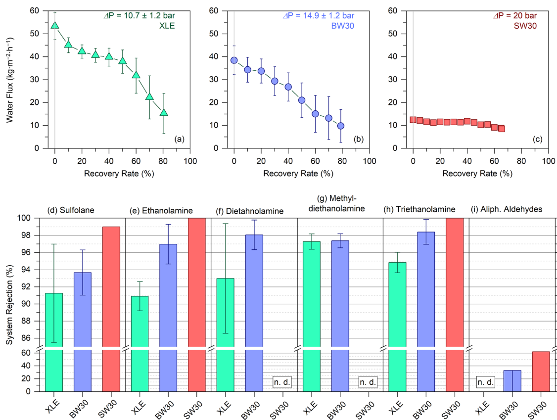
Fig. 3 | Performance of different reverse osmosis membranes in terms of water flux and compound rejection based on lab-scale batch experiments. a–c show measured water flux (LMH) as a function of recovery rate for the XLE (a; green triangles), BW30 (b; blue circles), and SW30 (c; red squares) membranes. The applied hydraulic pressure for each membrane is indicated in the respective panel. Data points represent the mean \pm one standard deviation from six (XLE) or seven (BW30) independent replicate experiments; no replicates were performed for SW30. Lines connecting the data points are included solely as a visual aid. d–i present
