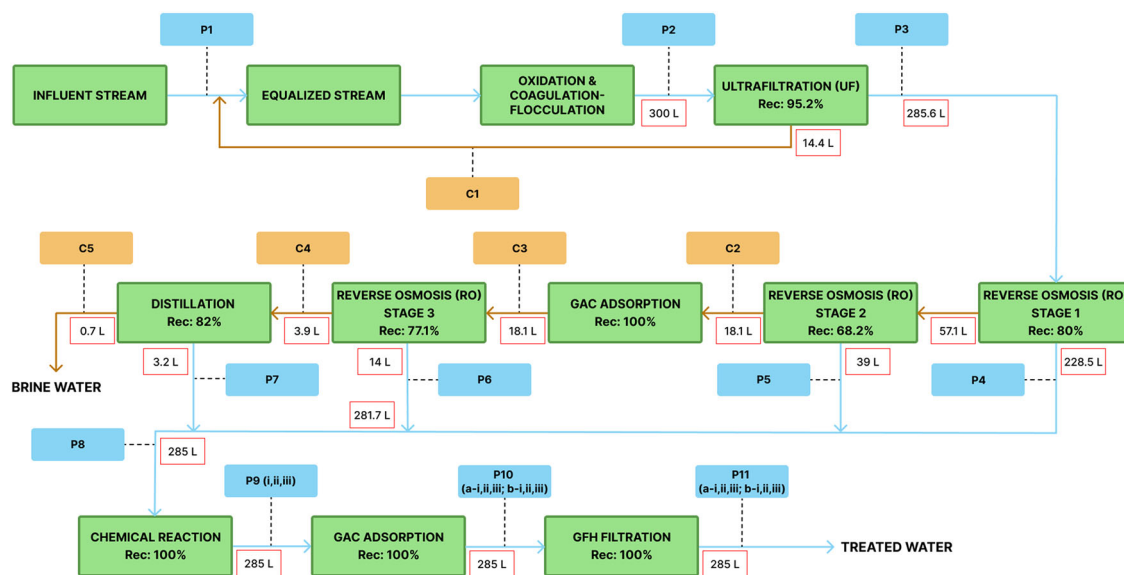
Fig. 8 | Block diagram of the treatment train developed for the remediation of contaminated groundwater. Green boxes indicate the unit processes investigated in this study. Blue arrows represent treated effluent streams, while orange arrows correspond to concentrate streams generated by unit operations with recovery rates below 100%. Recovery rate values are reported within the green boxes. The overall treatment train achieved a total water recovery of 99.75%. Volumes of water utilized
