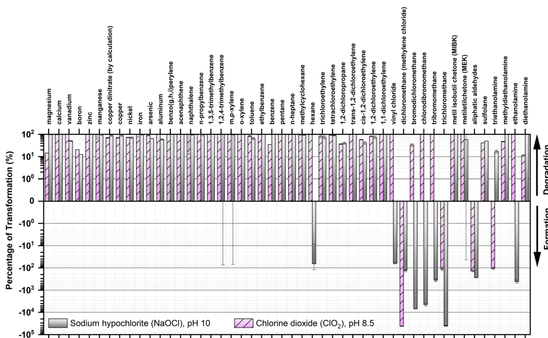
Fig. 1 | Percentage transformation of contaminants in the physico-chemical pre-treatment unit consisting of an oxidation–coagulation–flocculation process (OCF). Transformation was calculated as \left(1 - \frac{c_{FIN}}{c_0}\right) \times 100 , where c_0 is the influent concentration, and c_{FIN} is the effluent concentration. Bars represent the mean \pm one standard deviation from three independent replicate experiments. Gray solid bars correspond to treatment with sodium hypochlorite at pH 10, while pink
