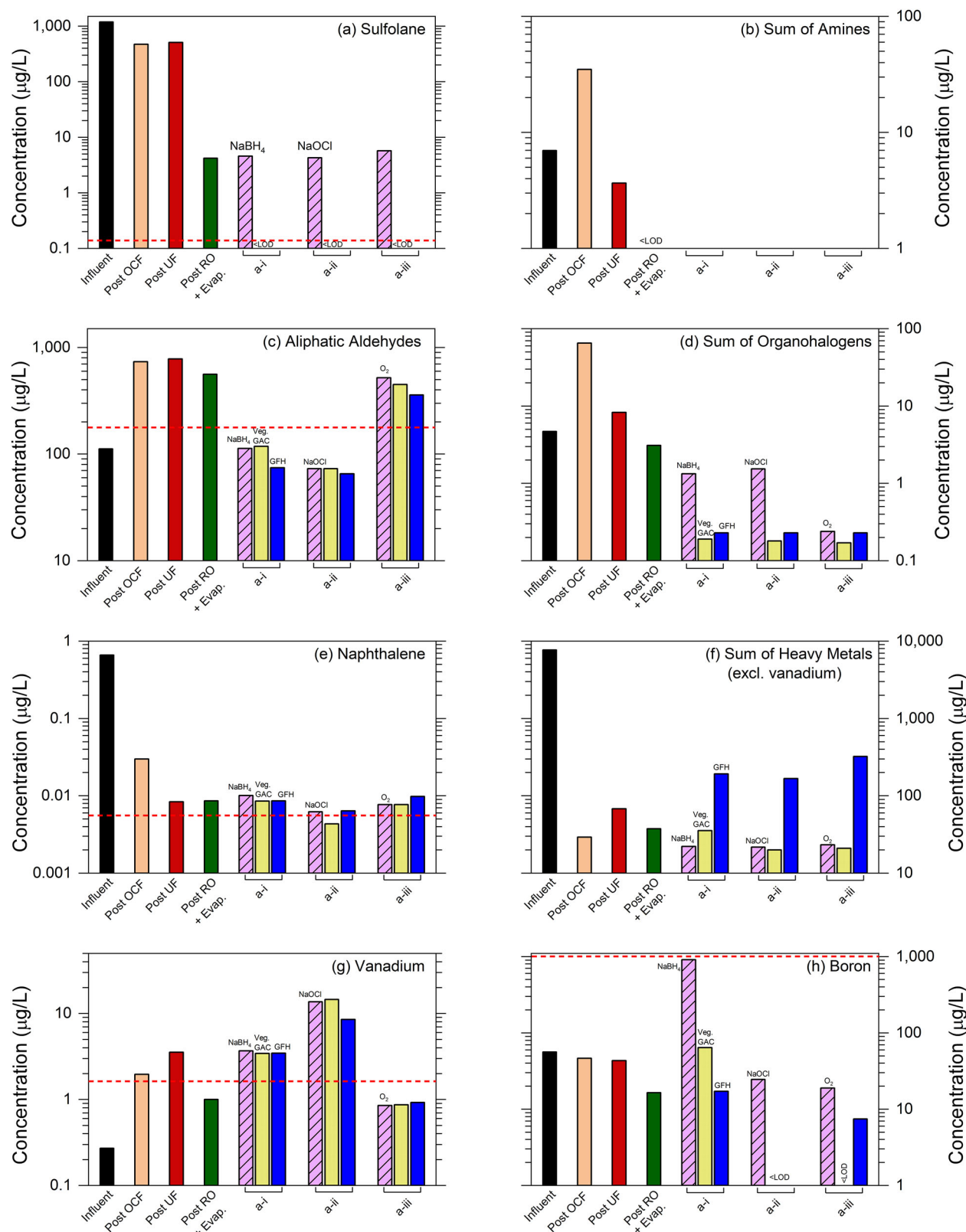
Fig. 7 | Concentrations of selected compounds or compound classes measured after sequential treatment steps. The red dashed horizontal line indicates the target concentration limit in the final effluent of the treatment train. “< LOD” denotes concentrations below the limit of detection. Bar colors correspond to the following sampling points: Black: influent; Light orange: effluent of oxidation–coagulation–flocculation (OCF); Red: effluent of ultrafiltration (UF); Green: combined permeate from the three
