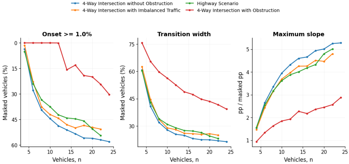
Fig. 7. Exposure Risk in case of CPM transmission, transition characteristics as a function of the number of vehicles in the scene, evaluated at maximum penetration rate. Each panel corresponds to one scenario. Left: onset threshold (masked-vehicle fraction at which CPM risk first exceeds 1%). Center: transition width. Right: maximum slope. Curves are colored by scenario type.
