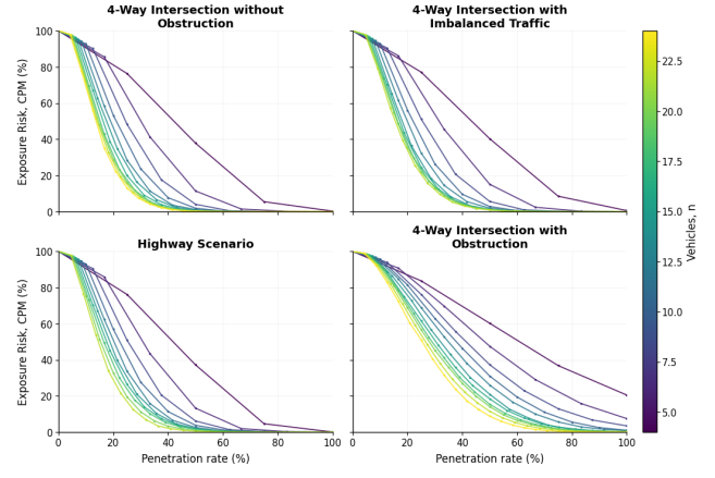
Fig. 5. CPM-based exposure risk as a function of the penetration rate. Each panel corresponds to one scenario, and each curve is colored according to the total number of vehicles present in the scene.
