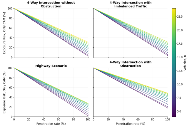
Fig. 3. CAM-only exposure risk as a function of the penetration rate. Each curve corresponds to a different number of vehicles, indicated by the colorbar.
