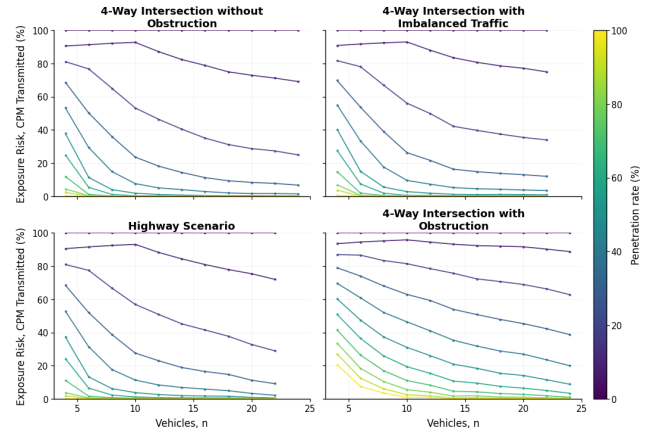
Fig. 6. CPM-based exposure risk as a function of the number of vehicles in the scene. Each panel corresponds to one scenario, and each curve is colored according to the penetration rate, i.e. the percentage of vehicles equipped with sensors and capable of sharing perception information.
