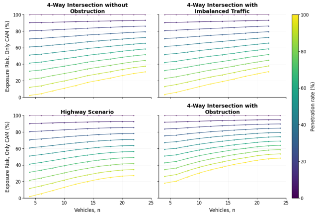
Fig. 4. CAM-only exposure risk as a function of the number of vehicles in the scene. Each panel corresponds to one scenario, and each curve is colored by the penetration rate, i.e. the percentage of vehicles equipped with sensors.
