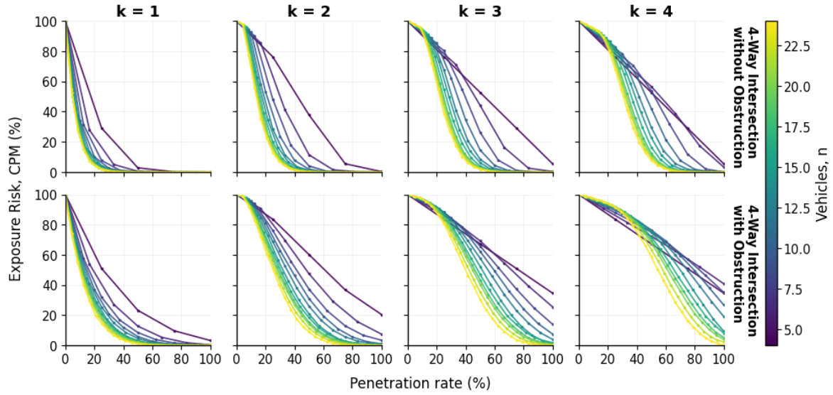
Fig. 8. Sensitivity of the CPM exposure risk to the detection threshold k (a ghost is undetected if observed by fewer than k equipped vehicles), for the open (top) and obstructed (bottom) intersections. Curves are colored by the number of vehicles in the scene.
