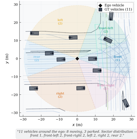
Fig. 1. Example of automatic labeling
