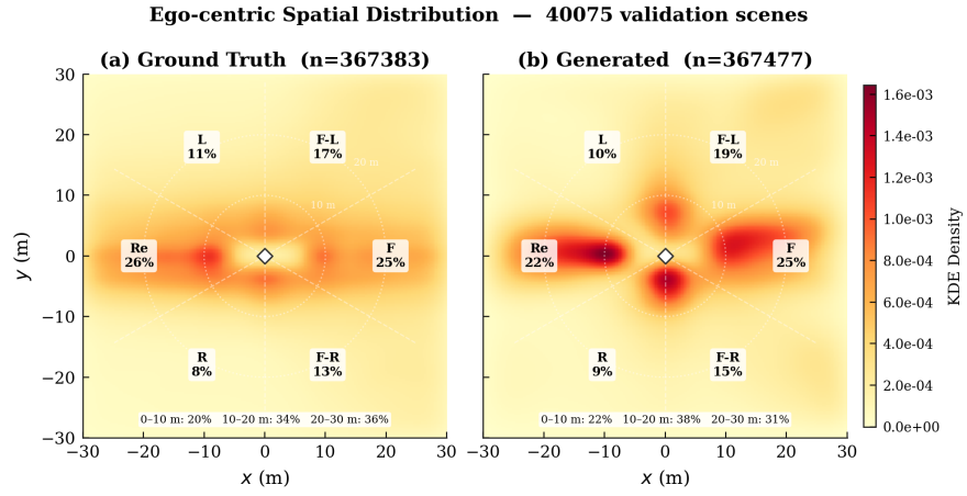
Fig. 4. Ego-centric spatial distribution of generated agents compared to ground truth, estimated via kernel density estimation (KDE, bandwidth = 2 m) over the validation dataset
