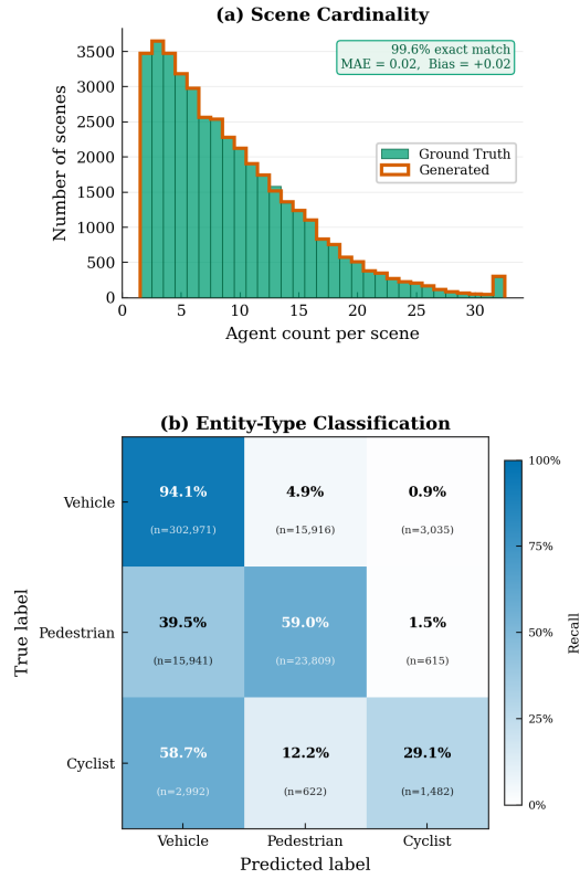
Fig. 3. Scene-level fidelity on the full Waymo Open Dataset validation set (40,075 scenes)
