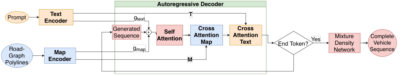
Fig. 2. Overview of the proposed model. A text encoder maps the input text prompt to a scene embedding, which conditions the Transformer decoder via cross-attention. The map encoder processes road-graph polylines into lane tokens, also attended by the decoder. At each autoregressive step, the decoder predicts a stop token probability; if generation continues, a Mixture Density Network outputs the next agent’s position, heading, velocity, and entity type. The process repeats until the end token is predicted or the maximum agent count is reached.
