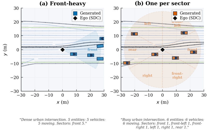
Fig. 5. Qualitative comparison of text-conditioned generation
