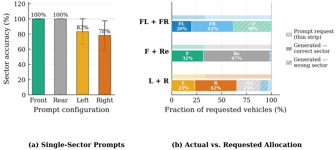
Fig. 6. Text-to-Sector Compliance. (a) Fill-rate for single-sector prompts (b) Vehicle allocation for mixed-sector prompts. Each row shows the actual distribution (solid bars) compared to the requested one (thin strip above). Hatched segments mark vehicles placed in the wrong sector.
