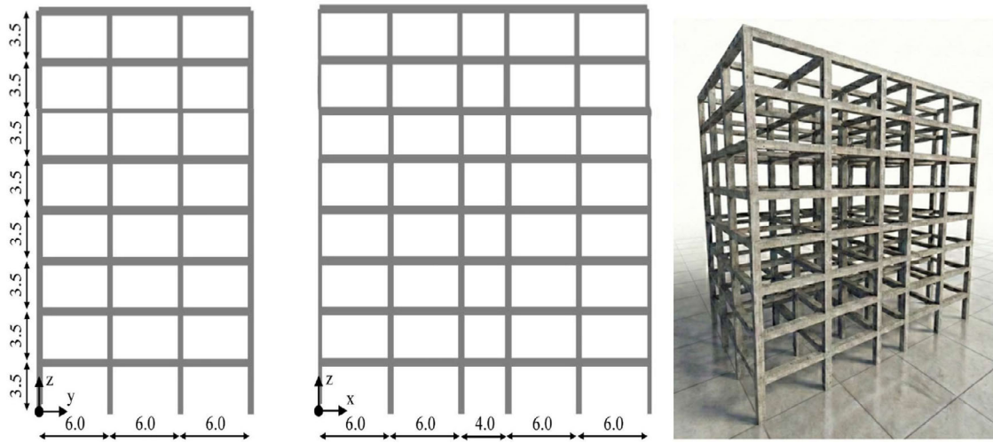
FIGURE 7 | Elevation views of the building structure. Y-Y axis elevation (left) and X-X axis elevation (center) and 3D isometric view of the structural frame (right).
