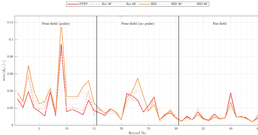
FIGURE 13 | Comparison of Maximum Storey Drift in X between standard approaches (FNFP, Rot 30°/60°) and the Intensity-based PP-RIO protocol (PP-RIO SED). The SED methodology consistently envelopes the demand, whereas fixed rotations exhibit volatile performance.
