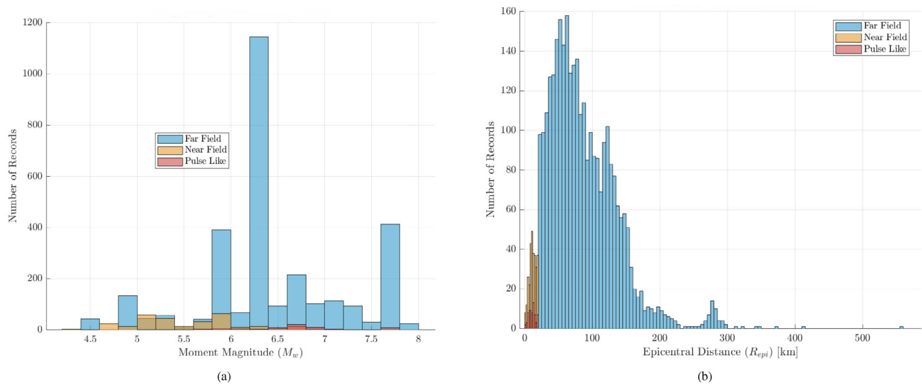
FIGURE 2 | Distribution of the selected records by class. (a) Moment magnitude ( M_w ) distribution of events contributing to the dataset. (b) Epicentral distance ( R_{epi} , km) distribution of the recordings, showing the overall distance span and the relative contribution of far-field, near-field, and pulse-like subsets.
