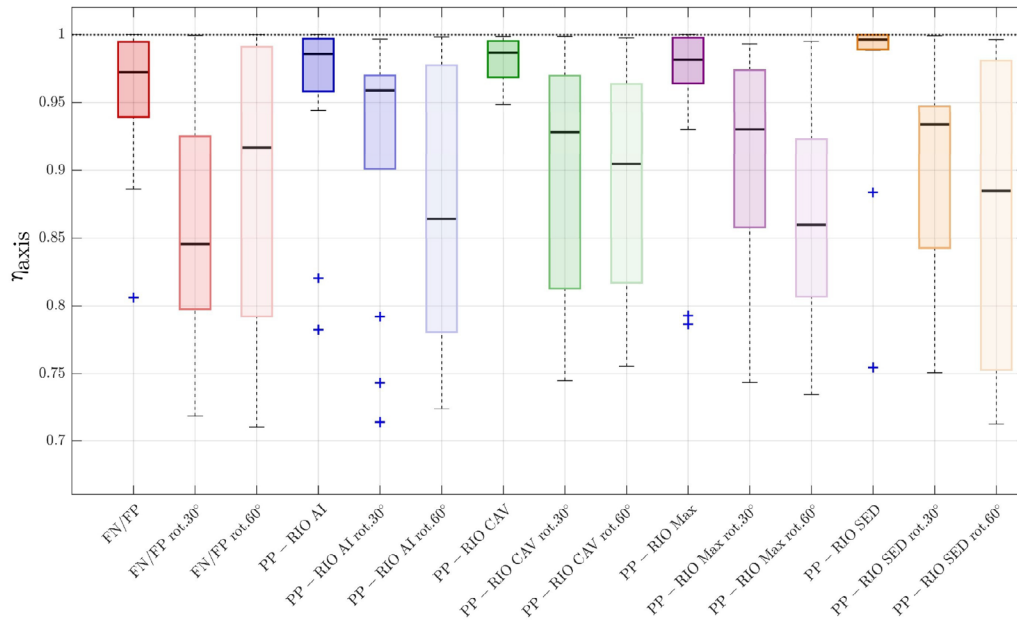
FIGURE 14 | Quantile bands of the directionality efficiency index \eta for top-floor displacement. The compact distributions for integral IM, particularly the SED and CAV, based protocols indicate a statistically superior capability to capture the maximum structural demand and lower dispersion compared to geometric fixed-rotations ( 30^\circ/60^\circ ) or FN/FP PGA-based (PP-RIO Max) methods.
