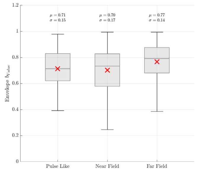
FIGURE 6 | Global statistical comparison of the envelope ellipticity descriptor b_{value} across the PL, NF, and FF subsets. The box limits represent the first and third quartiles, the horizontal line inside each box denotes the median, the whiskers indicate the lower and upper non-outlier ranges, and the red cross marks the mean value. Lower b_{value} values correspond to more elongated and directionally concentrated polar envelopes, whereas values approaching unity indicate a more isotropic distribution of horizontal intensity.
