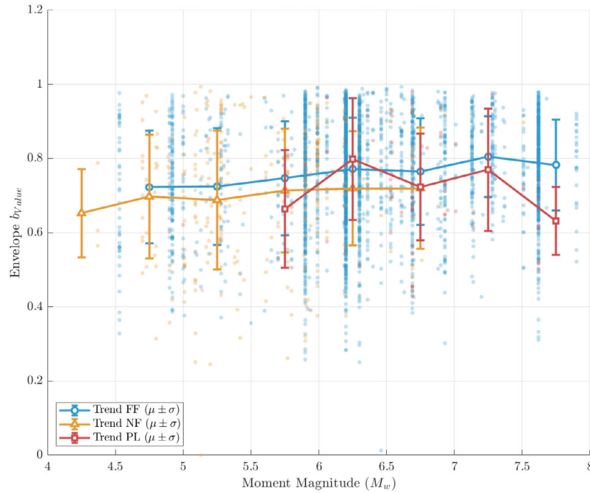
FIGURE 5 | Scatter and trend analysis of the envelope ellipticity descriptor b_{value} as a function of moment magnitude ( M_w ) for the FF, NF, and PL subsets. Individual points represent single records, while connected markers indicate the mean b_{value} computed within each magnitude bin. Error bars denote \mu \pm \sigma , where \mu and \sigma are the mean and STD of b_{value} within the corresponding bin.
