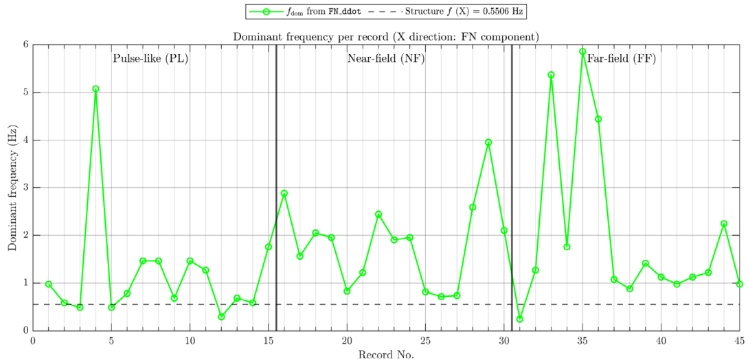
FIGURE 11 | Distribution of dominant frequencies ( f_{dom} ) for the FN component across the analyzed datasets. The fundamental structural frequency ( f_{struct} = 0.5506 Hz) is denoted by the dashed line, highlighting potential pulse-period compatibility conditions particularly within specific events in the PL regime.
