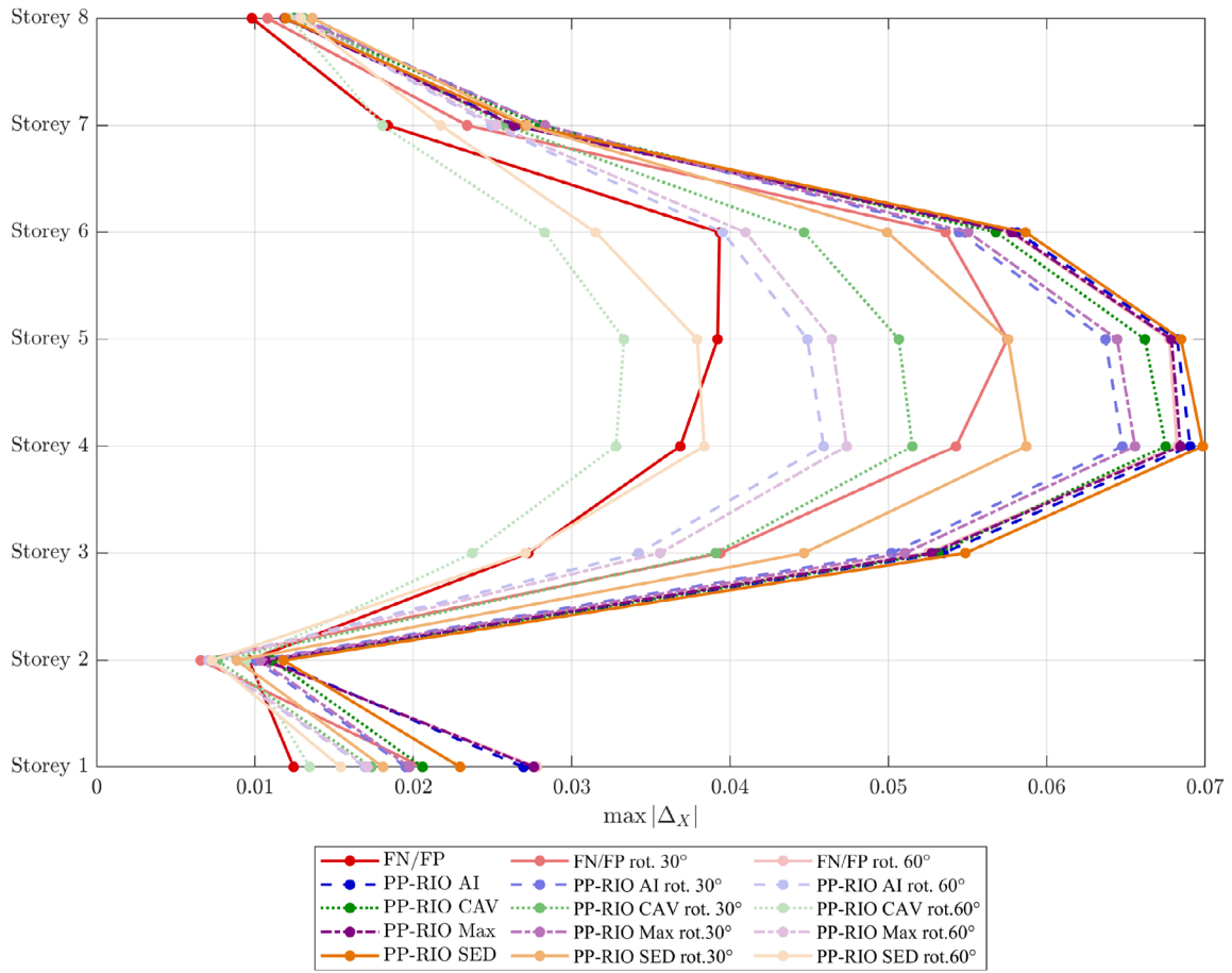
FIGURE 10 | Vertical profiles of maximum storey drift ratios (SDR) for Record ID 034. The standard orientation is observed to underestimate the deformation demand ( \approx 3.9\% ) compared to the Intensity-based PP-RIO orientations which reveal critical drifts reaching \approx 7.0\% .
