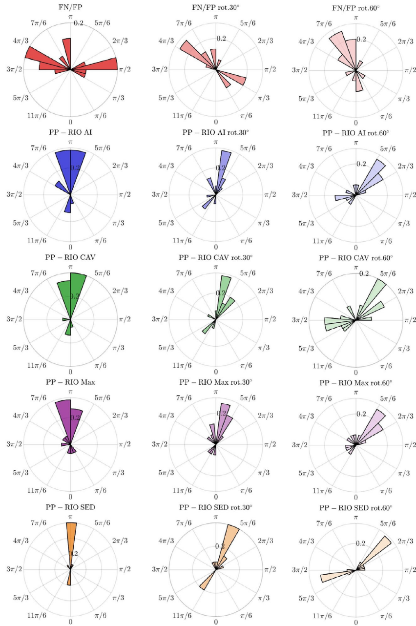
FIGURE 15 | Polar histograms of the response angle associated with the peak resultant top-floor displacement for the complete Pulse-Like dataset ( N = 69 ). The response angle is evaluated at the time instant at which the resultant roof displacement reaches its maximum value. Rows correspond to the fault-aligned FN/FP protocol and to the PP-RIO orientations derived from different scalar IMs, while columns show the reference orientation and additional rotations of 30^\circ and 60^\circ . The broader, multi-lobed distributions observed for the geometric FN/FP-based protocols indicate greater sensitivity of the peak response direction to the adopted reference frame. In contrast, the PP-RIO protocols show increased directional clustering, particularly for the SED-based orientation, suggesting a more stable alignment between the intensity-based input direction and the resulting structural response.
