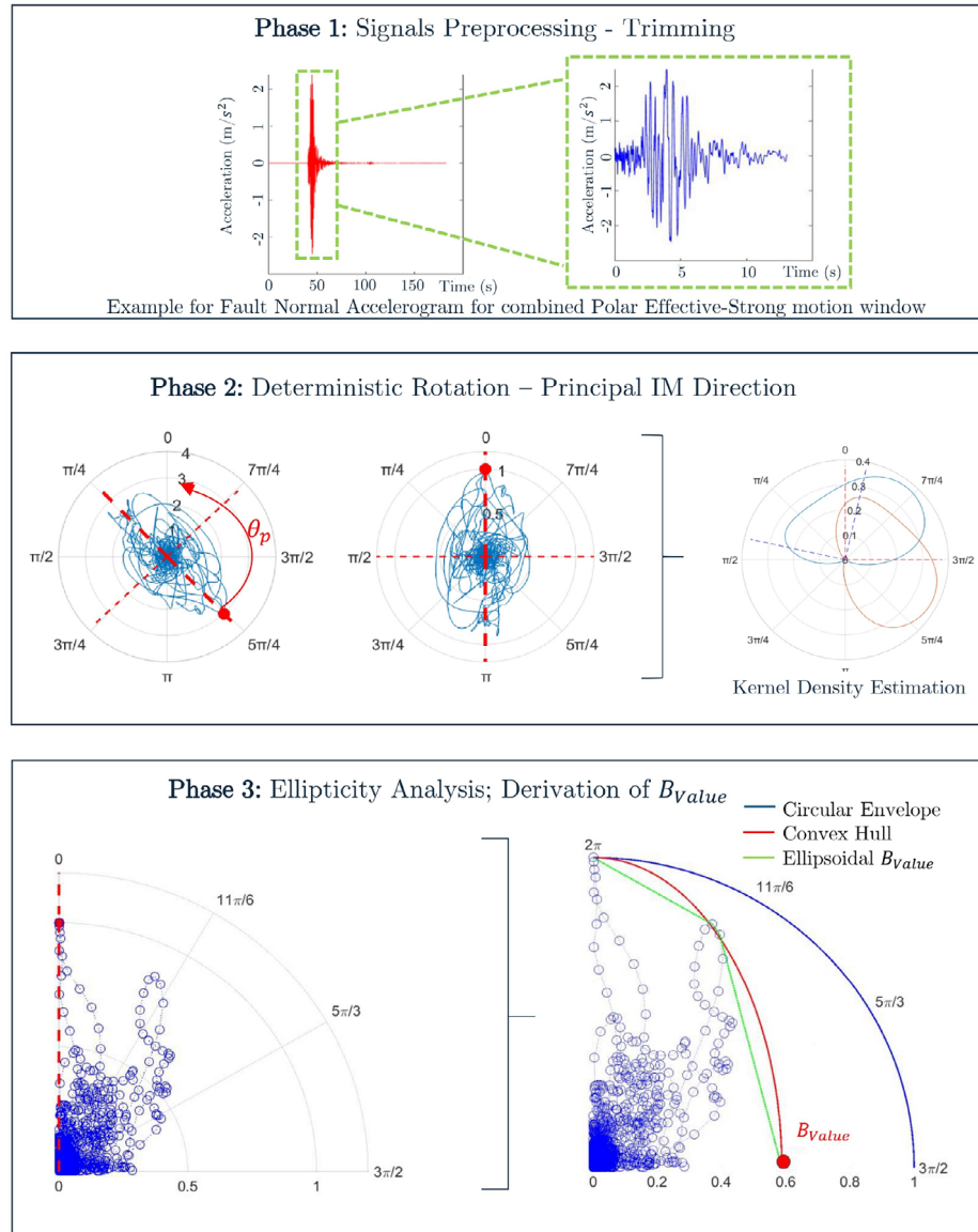
FIGURE 4 | Workflow of the PP-RIO procedure for identifying the polar principal orientation and deriving the b_{value} polarization descriptor. Phase 1 shows the preprocessing and trimming of the accelerometric signal. Although one horizontal component is illustrated for clarity, the effective strong-motion window is defined from the combined polar resultant of the two synchronized horizontal components and is then applied consistently to both records. Phase 2 presents the deterministic rotation of the bidirectional acceleration trajectory toward the principal IM direction, defined by the angle \theta_p associated with the maximum polar intensity. The Kernel Density Estimation is included only as an illustrative diagnostic to visualize the directional concentration of the rotated samples in polar space. Phase 3 shows the normalized and folded polar trajectory used for the ellipticity analysis. The convex hull defines the outer directional support of the acceleration point cloud, while the fitted ellipsoidal envelope provides the scalar descriptor b_{value} . Lower b_{value} values indicate stronger polarization and a more elongated trajectory, whereas values approaching unity indicate a more isotropic distribution of horizontal intensity.
