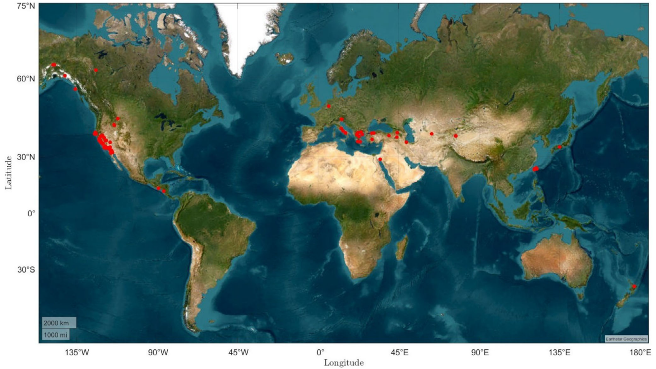
FIGURE 1 | Global distribution of epicenters, with clusters in the western U.S., the Mediterranean (Italy–Turkey–Greece), Japan, Taiwan, and New Zealand. This coverage spans major faulting mechanisms and plate-boundary settings, so the derived statistics are representative of global active crustal seismicity.
