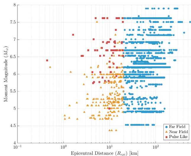
FIGURE 3 | Magnitude–distance distribution of the selected ground motions. Moment magnitude ( M_w ) is plotted against epicentral distance ( R_{epi} , km; log-scale), with markers distinguishing FF, NF, and PL records, highlighting the complementary coverage of the dataset across source size and recording distance.
