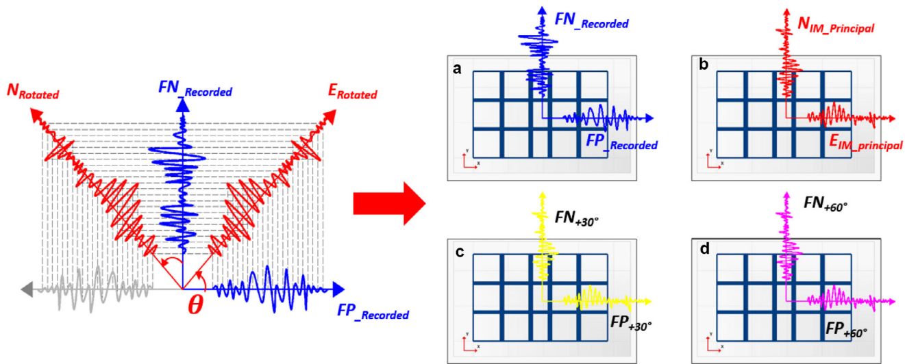
FIGURE 8 | Schematic representation of the PP-RIO methodology. The left panel depicts the continuous coordinate transformation of the fault-aligned orthogonal components ( FN_{Recorded} , FP_{Recorded} ) to identify the critical incidence angle \theta that maximizes a selected IM. The right panels illustrate the comparative application strategies: (a) the original fault-aligned orientation relative to the structural plan; (b) the proposed methodology, wherein the structural axes are rigorously aligned with the principal intensity axes ( N_{IM\_Principal} , E_{IM\_Principal} ) corresponding to the maximum demand; and (c, d) conventional arbitrary rotation schemes (e.g., 30^\circ and 60^\circ ).
