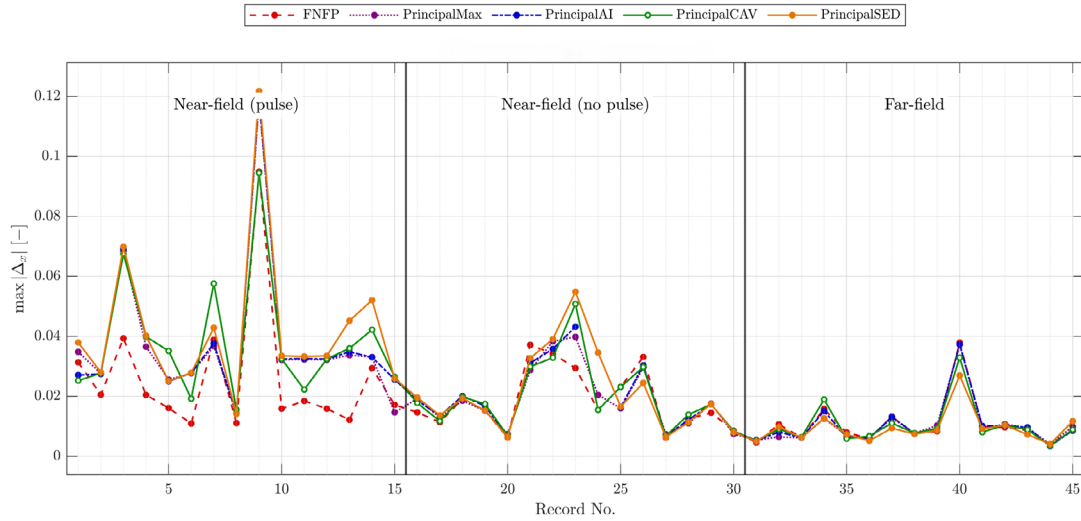
FIGURE 12 | Global comparison of maximum X-direction storey drift ( \max |\Delta_x| ) across all records. Note the critical divergence in the Pulse-Like regime (e.g., Record 9), where standard recording orientations significantly underestimate the potential demand identified by principal metrics.
