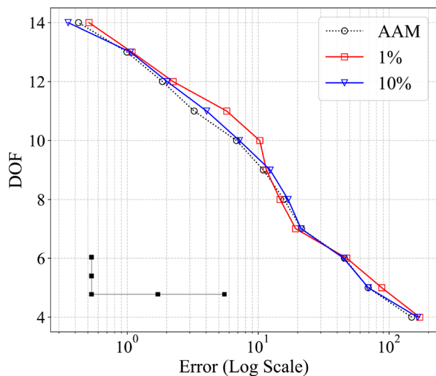
Fig. 13 BTD of the L beam included in the network training. For each DOF level, curve report the minimum error achieved by the structural theories evaluated by FEM or NN
