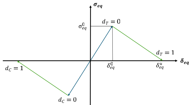
Fig. 1 Bilinear damage evolution
