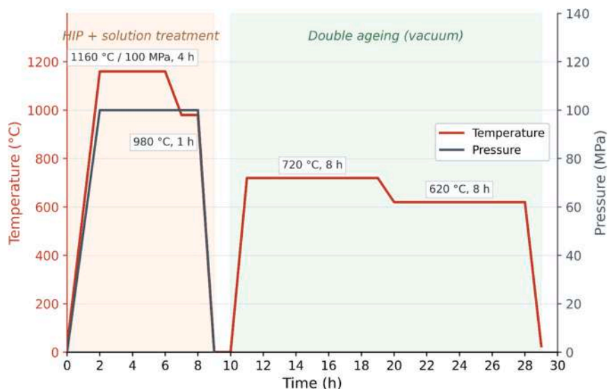
Fig. 1. Schematic representation of the HIP + heat-treatment applied to PBF-LB IN718.
