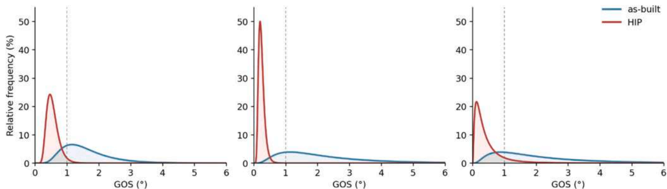
Fig. 11. Fitted GOS distributions of as-built and HIP conditions for samples 28, 29 and 30.
