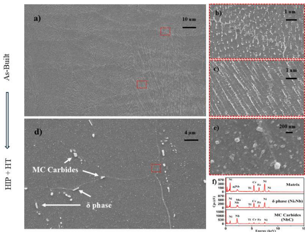
Fig. 9. SEM micrographs of PBF-LB IN718 (a–c) in the as-built condition, showing the cellular–dendritic substructure with Nb-rich interdendritic boundaries, and (d, e) after HIP and double ageing, showing MC carbides and \delta -phase at the grain boundaries and fine \gamma'/\gamma'' precipitates within the matrix; (f) EDS spectra of the matrix, \delta -phase and MC carbides.
