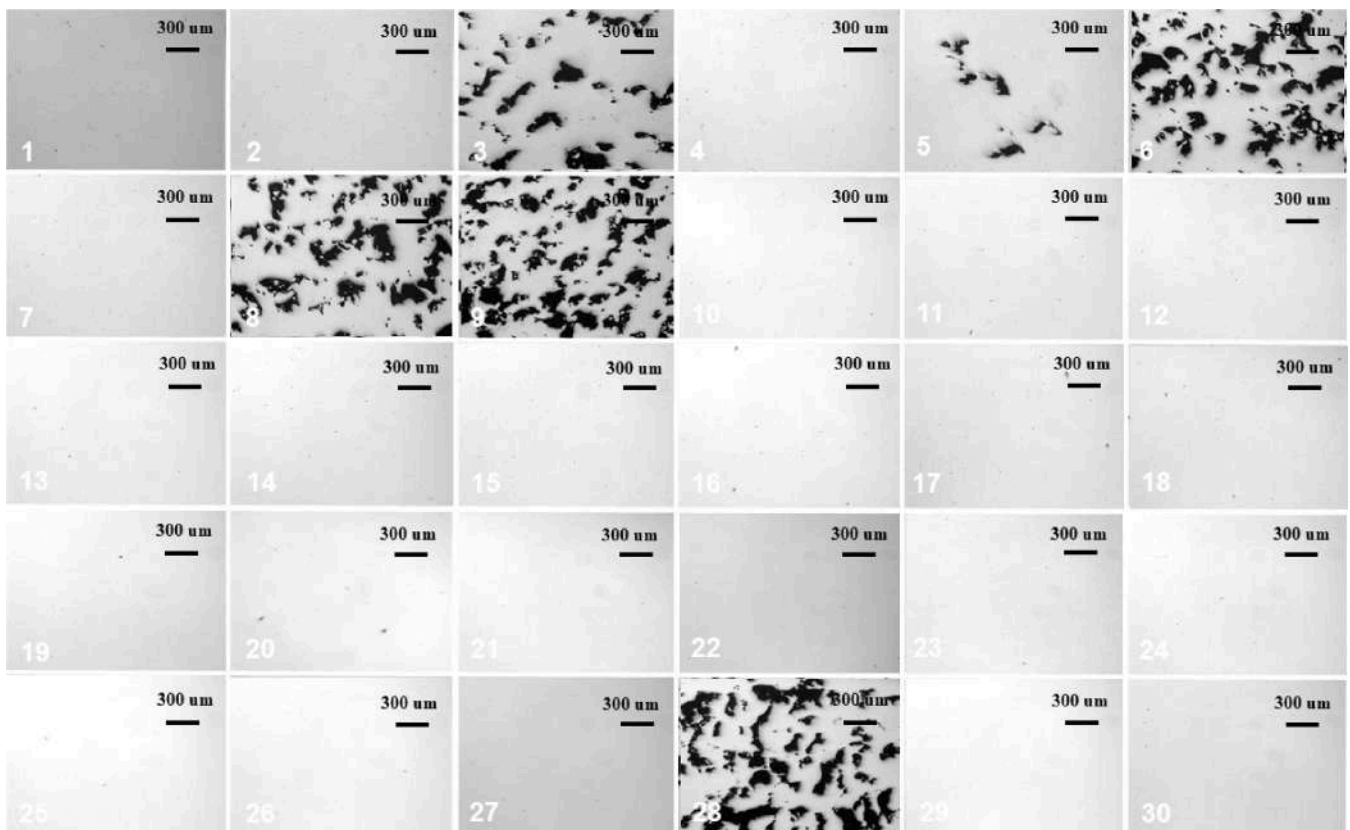
Fig. 4. Optical micrographs showing the pore distribution in as-built PBF-LB IN718 after HIPing.
