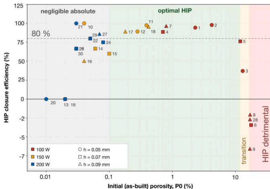
Fig. 15. Evolution of porosity before and after HIP vs efficiency across different samples.
