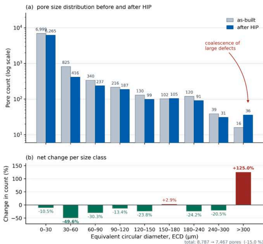
Fig. 6. Pore size distribution of PBF-LB IN718 in terms of pore count versus equivalent circular diameter (ECD), (a) as-built and post-HIP counts per size class on a logarithmic scale; (b) net change in count per class.
