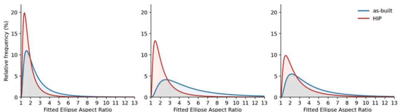
Fig. 12. Fitted AR distributions of as-built and HIP conditions for samples 28, 29 and 30.
