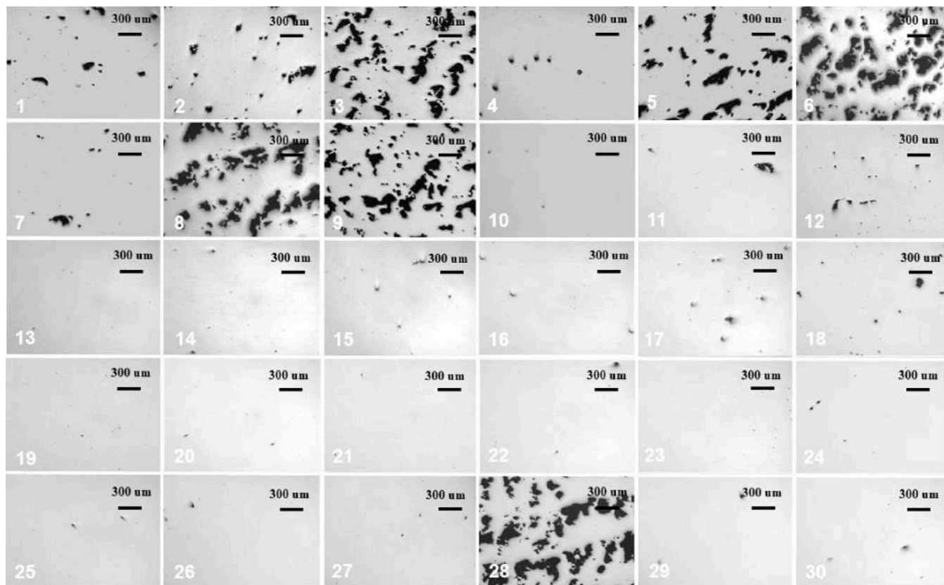
Fig. 2. Optical micrographs showing the pore distribution in as-built PBF-LB IN718 before HIP.
