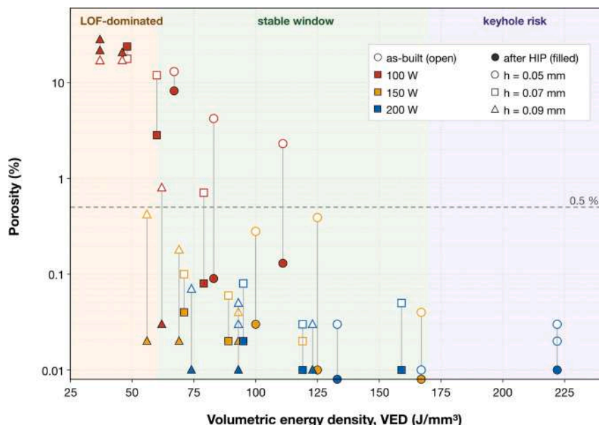
Fig. 5. Variation of Porosity Across PBF-LB IN718 Samples Before and After HIP Treatment.
