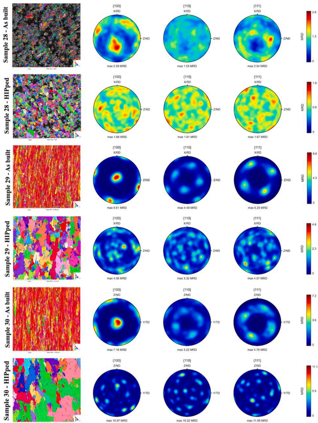
Fig. 10. IPF maps with the corresponding pole figures of as-built and HIP conditions for samples 28, 29 and 30.
