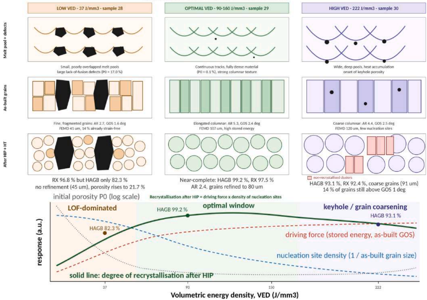
Fig. 13. Schematic representation of the effect of volumetric energy density on melt pool geometry, defect population and recrystallisation response after HIP in PBF-LB IN718. Low VED produces small, poorly overlapped melt pools, large lack-of-fusion defects and a weakly deformed as-built structure that only recovers during HIP; intermediate VED produces continuous, defect-free material with a highly deformed columnar structure that recrystallizes almost completely; high VED saturates the driving force while coarsening the grains and reintroducing keyhole porosity, leaving residual strained clusters after HIP. The bottom plot illustrates the resulting maximum in recrystallisation degree at intermediate VED as the product of a saturating driving force and a decreasing nucleation-site density (markers: measured post-HIP HAGB fractions for samples 28, 29 and 30). The curve is shown as a conceptual schematic linking these three measured conditions and does not represent a fitted or continuously validated relationship.
