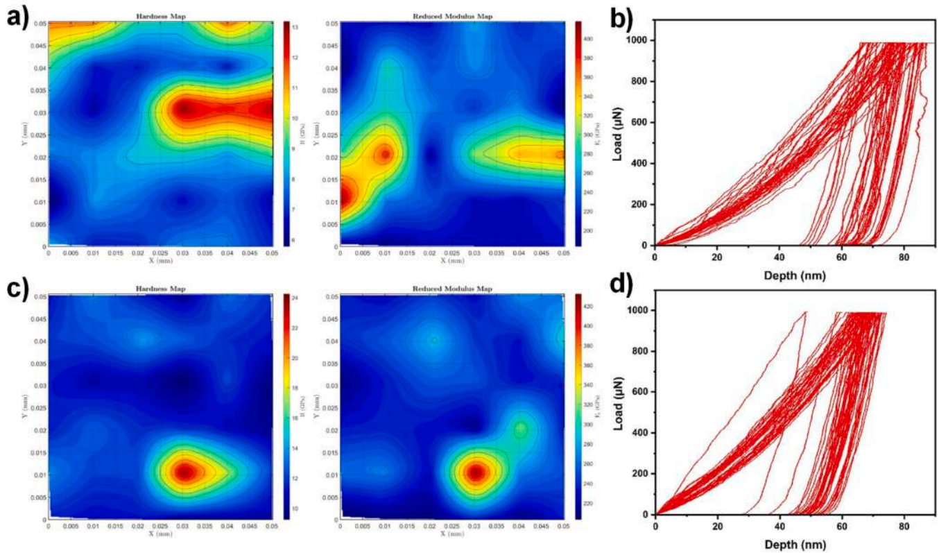
Fig. 14. Nanoindentation results from a 6 \times 6 grid array showing (a) pre-HIP hardness map and modulus map, (b) pre-HIP load-displacement, (c) post-HIP hardness map and modulus map, and (d) post-HIP load-displacement curves.
