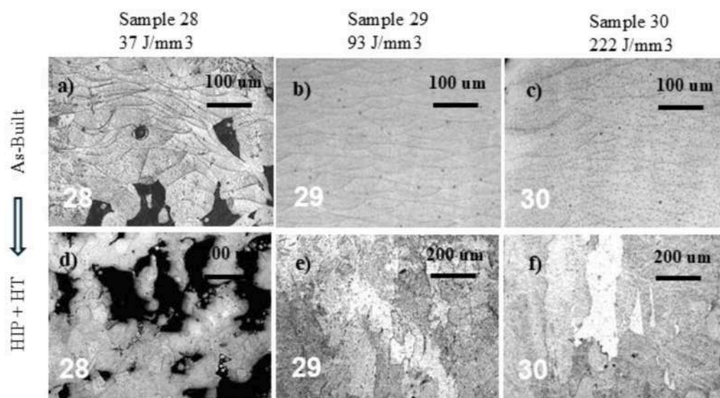
Fig. 7. Etched micrographs of PBF-LB IN718 samples in the as-built condition showing melt pool morphology.
