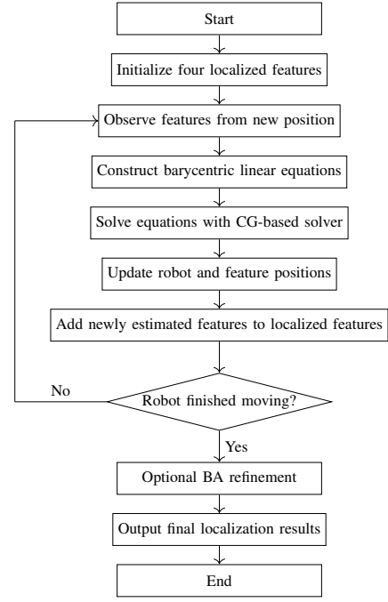
Fig. 2. Workflow of the proposed SRAFL approach. The lightweight BL-SRAFL provides online estimates, while an optional BA back-end refines the solution offline when higher accuracy is required.
