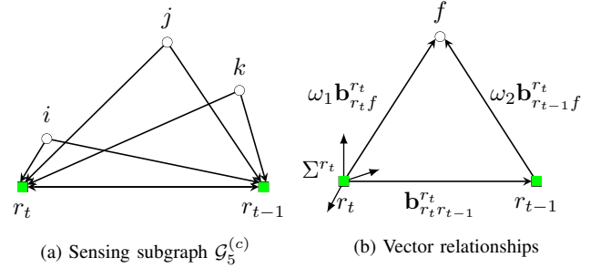
Fig. 3. Illustrations of the barycentric linear formulation.
