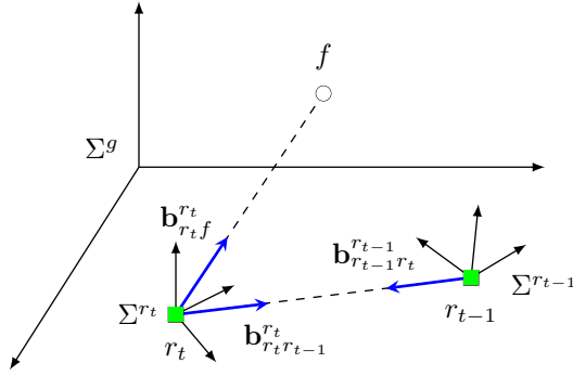
Fig. 1. An illustration of angle-based sensing. The green square represents the monocular camera, while the circle indicates features. Blue lines with arrows depict bearing angle measurements, black lines with arrow denote coordinate axes, and the dashed line serves as an auxiliary reference.
