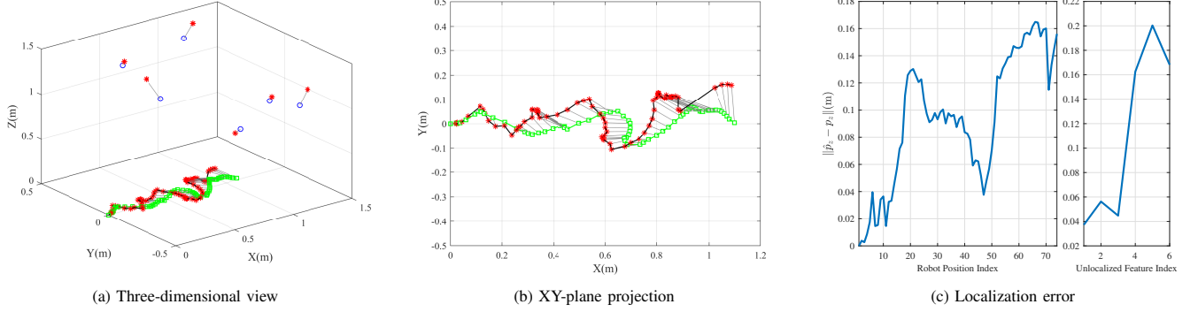
Fig. 8. Illustration of the experimental localization results of BL-SRAFL for the case study in Subsection V-B.
