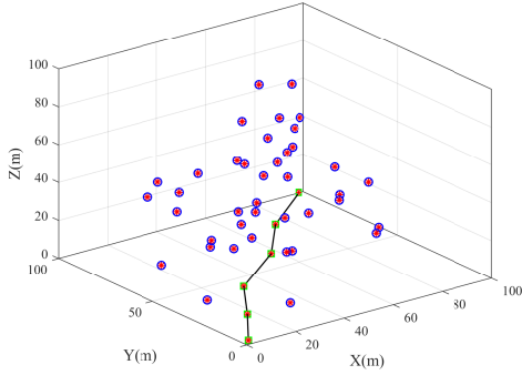
Fig. 6. Illustration of the final three-dimensional robot trajectory and feature positions generated by BL-SRAFL for the case study in Subsection V-A.
