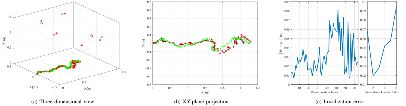
Fig. 9. Illustration of the experimental localization results of BL-SRAFL+BA for the case study in Subsection V-B.
