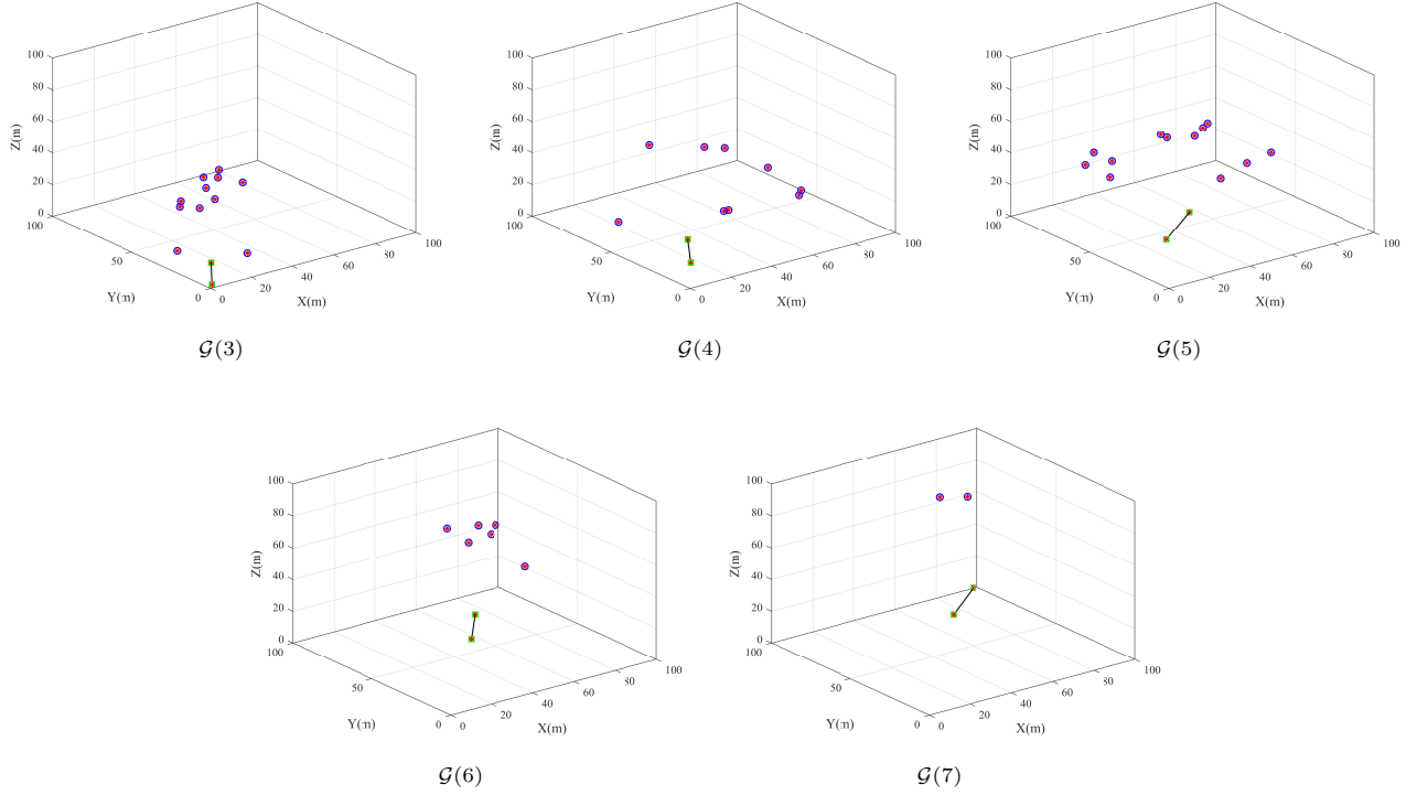
Fig. 5. Plots illustrating the convergence results of Algorithm 1 for the five moves of the robot. Blue circles and green squares are positions of features and robot, respectively, red asterisks are the final estimated positions of the robot and features, and black lines represent the estimated robot trajectory.
