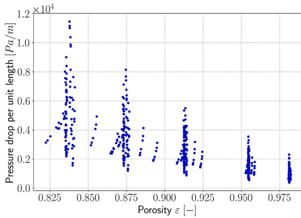
Fig. 6. Pressure drop per unit length as a function of the porosity \varepsilon (without the Hexagonal_GEO geometry).
