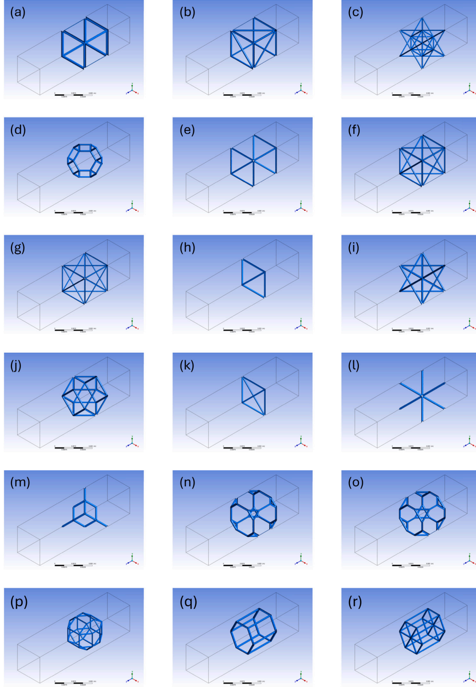
Fig. 1. Overview of the analyzed geometries: (a) Cube cell; (b) FD-Cube cell; (c) Octet cell; (d) Kelvin cell; (e) SC-BCC truss cell; (f) SC-FCC truss; (g) SC-Full truss; (h) Octa cell; (i) V-Octet cell; (j) T-Cube cell; (k) Octa cross cell; (l) Body center cell; (m) Diamond cell; (n) Truncated Cube4; (o) Truncated Cube3 cell; (p) Rhombicuboctahedron cell; (q) Hexagonal-empty cell; (r) Hexagonal cell. The porosity is \epsilon = 0.981 for all cells, except for the (o) Truncated Cube3 cell (which is \epsilon = 0.982 ).
