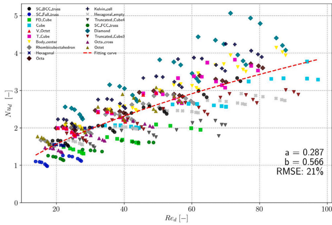
Fig. 8. Results of the 397 simulations in the final dataset, and best fitting curve according to Eq. (26). The obtained values of the fitting parameters are also reported, along with the RMSE error.
