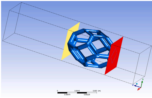
Fig. 2. Unit cell of a representative 3D printed lattice (Kelvin cell with porosity \varepsilon = 0.9 ) for solid–fluid heat exchange. The boundaries of the simulated domain are depicted with black lines, while the solid struts of the 3D printed cell are represented in blue. The cell inlet and outlet planes for the fluid flow are highlighted in red and yellow, respectively (note that, these latter planes do not coincide with the inlet and outlet boundaries of the domain).
