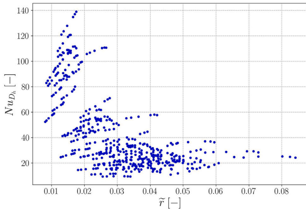
Fig. 11. Nu_{D_h} as a function of the dimensionless radius \tilde{r} .
