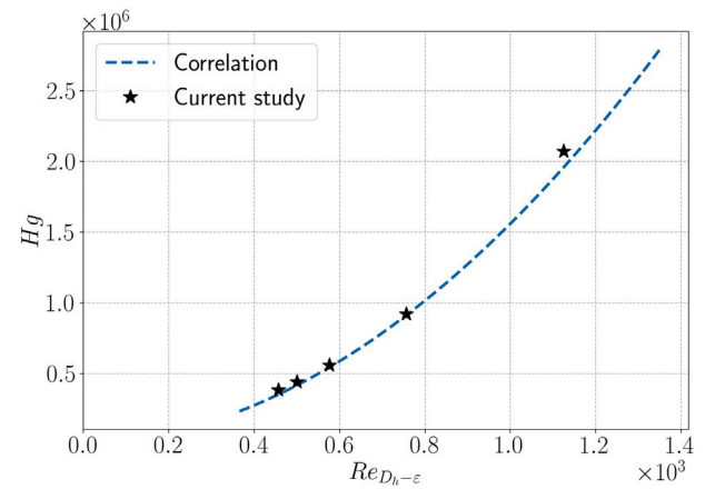
Fig. 5. Comparison of the Hagen numbers obtained in the current study for a Kelvin cell (with 1.0 elongation along the flow direction and porosity values in the range 0.83 to 0.981) and the correlation in Eq. (25), developed by [58].
