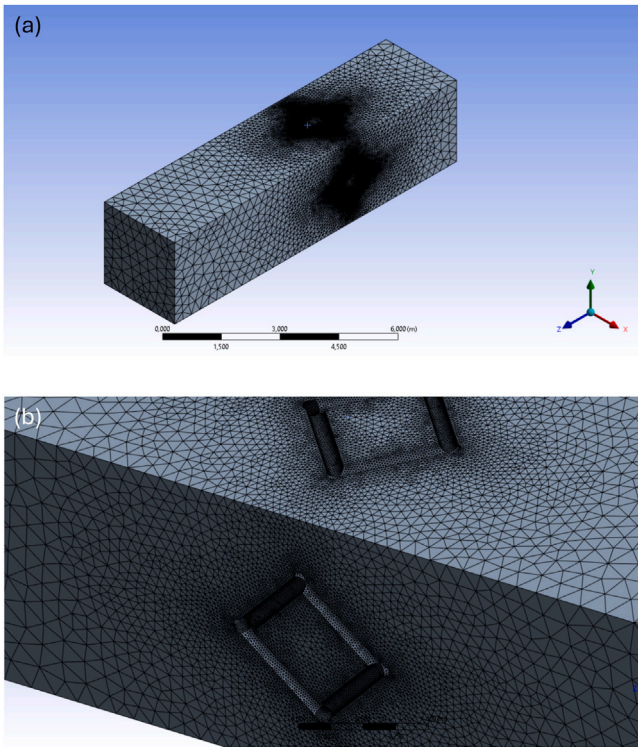
Fig. 3. Meshing of the computational domain: (a) overview of the mesh of the whole domain for a Kelvin cell; (b) detail of the mesh in the proximity of the Kelvin cell geometry.
