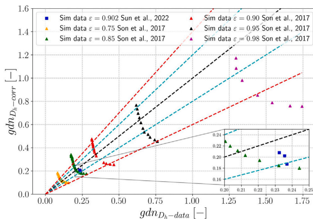
Fig. 10. Correlation (31) used with modified Kelvin cells (square markers, Sun et al. 2022) and with Tetrahedral cells (triangular markers, Son et al. 2017). The black dashed lines correspond to the correlation line, the light-blue dashed lines to \pm 20\% error, and the red dashed lines to \pm 40\% error.
