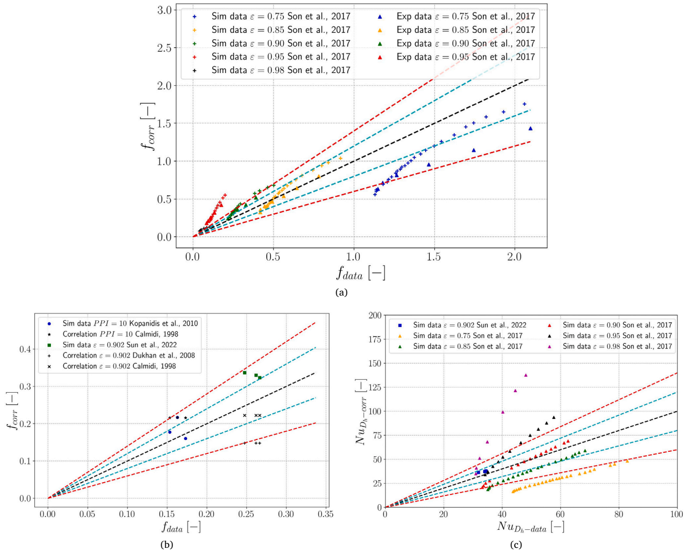
Fig. 9. (a) Correlation (28) compared with experimental and simulated data from [36]; (b) Correlation (28) compared with simulation of a modified Kelvin cell [34], a Weaire–Phelan structure [68] and correlations from Calmidi [69] and Dukhan [70]; (c) Correlation (27) compared with Tetrahedral (triangular markers) and modified Kelvin cells (square markers). The black dashed lines correspond to the correlation line, the light-blue dashed lines to \pm 20\% error, and the red dashed lines to \pm 40\% error.
