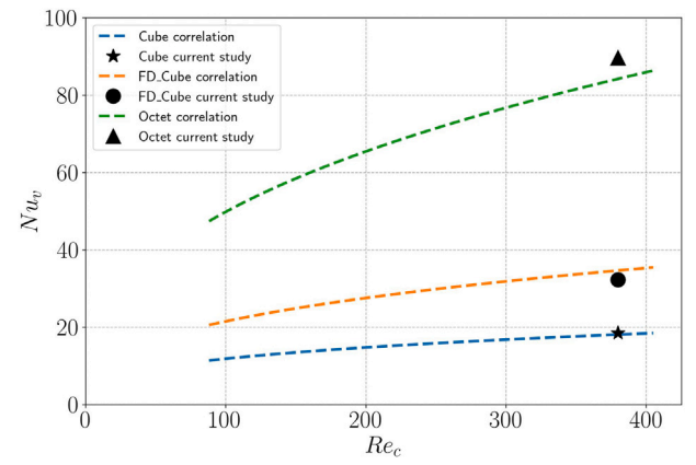
Fig. 4. Comparison of the volumetric Nusselt number obtained in the current study for different cells with the correlations reported in [25].
