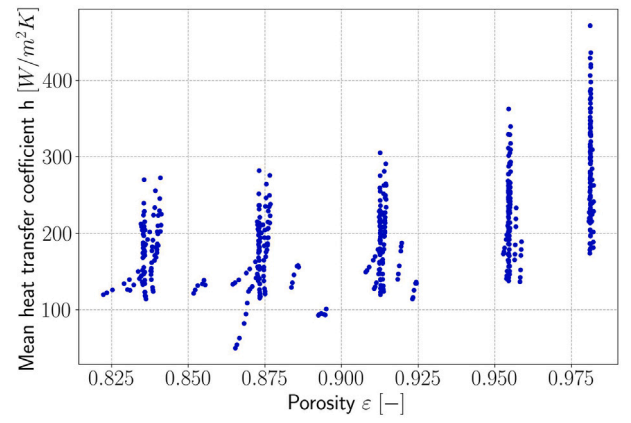
Fig. 7. Mean heat transfer coefficient as a function of the porosity \varepsilon .
