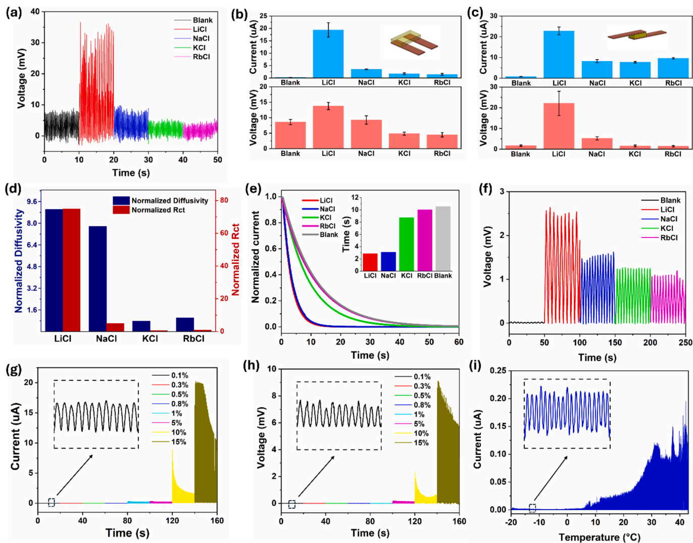
Fig. 3. Analysis of ionic conductivity in different PVA/AAC samples and electrical response under different parameters. a) Electrical voltage output of sandwich samples containing different salts to a constant local pressure of 10 N at 4 Hz. Comparison of the electrical outputs of current and voltage to a mechanical deformation for samples in b) parallel and c) sandwich configurations (frequency of 4 Hz and a constant force of 10 N). Error bars represent the standard deviation of peak values over 10 consecutive cycles. d) Diffusivity and charge transfer resistance values for each of the salts obtained during EIS test on a parallel sample. The values of the diffusivity and the charge transfer resistance were normalized with respect to the ones of RbCl sample. e) Current stabilization over time according to the salt content within a sandwich sample after a constant force deformation (80 N). Inset shows the bar chart with the time value for each of the salts. f) Voltage responses of dog-bone samples containing different salts, subjected to a cyclic tensile test at a speed of 200 \text{ mm min}^{-1} in the range 0–20% of strain. g) Electrical current and h) voltage output of a PVA/AAC/LiCl sample ( 1.5 \times 15 \times 10 \text{ mm}^3 ) to a dynamic compressive deformations (range from 0.1% to 15% strain). Insets illustrate a zoom of the cycles of some electrical cyclic responses. i) Current output to a dynamic mechanical thermal test at 1 Hz and 1% strain deformation in compression setup (temperature range from -20^\circ\text{C} to 43^\circ\text{C} ).
