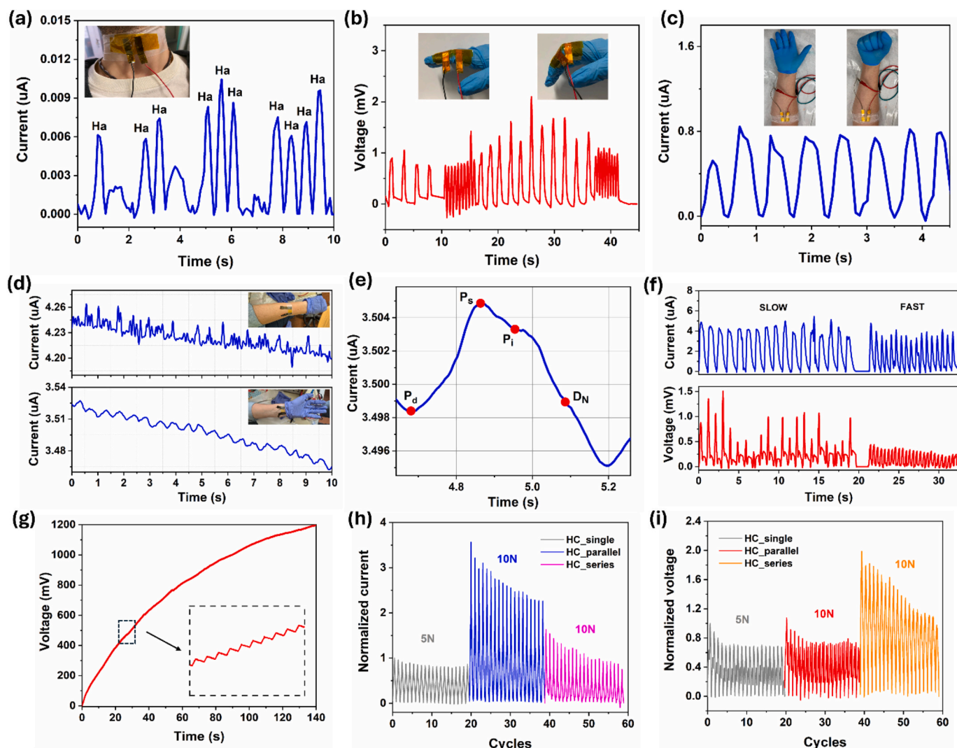
Fig. 5. Performances of flat and 3D piezoionic hydrogel samples. a) Recognition of vocal cord movement during laughter. b) Finger bending monitoring with different speeds movements. c) Current response to hand opening and closing. d) Heart rate sensed on the forearm (top) and on the wrist (bottom). e) Zoom of the pulse waveform with the corresponding diastolic pressure ( P_d ), systolic pressure ( P_s ), inflection point ( P_i ) and the dicrotic notch ( D_n ). f) Recording of the electric current (top) and voltage (bottom) output during a walk at different speeds. g) Charging of 1 \mu\text{F} capacitor for 140 s during a constant mechanical deformation of a honeycomb sample. Some charging steps are shown in the inset. h) The improvement of instantaneous current by connecting in series two piezoionic 3D printed devices. i) The improvement of instantaneous voltage by connecting in series two piezoionic 3D printed devices.
