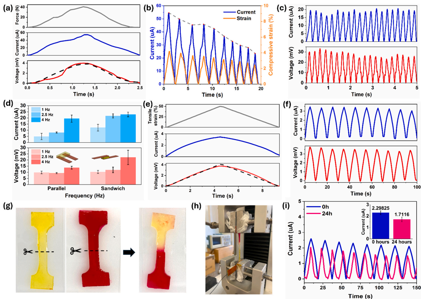
Fig. 2. Mechanical and electrical characterization of a PVA/AAc/LiCl piezoelectric sensor. a) Electrical current (middle) and voltage (bottom) responses of a sandwich-shaped sample to an external stimulus of 40 N (top). Simulated voltage response is superimposed with a dashed line to the experimental data. b) Current and strain behavior during a cyclic compression stimulus of 40 N at 25 mm min -1 in a sandwich-shaped sample. The dotted line follows the decay of the current for each cycle. c) Electrical current and voltage output of sandwich sample to a constant mechanical pressure of 10 N at 4 Hz. d) Comparison of the electrical outputs of current and voltage to mechanical pressure for both samples in sandwich and parallel configurations, at different frequencies and a constant force (10N). Error bars represent the standard deviation of peak values over 10 consecutive cycles. e) Electrical current (middle) and voltage (bottom) responses of a dog-bone sample to a tensile test with a strain from 0% to 50% (top). Simulated voltage response is superimposed with a dashed line to the experimental data. f) Electrical current and voltage output of a dog-bone sample subjected to a cyclic tensile test (at a speed of 200 mm min -1 in the range 0–50% of strain). g) Pristine tensile test specimens (left) and self-healed sample after 24 h (right). h) Self-healed sample subjected to a cyclic tensile test. i) Current output variation of pristine and self-healed samples subjected to a cyclic tensile test (strain range of 0–50% and speed of 200 mm min -1 ). The inset shows the bar graph with the average current value of 10 consecutive cycles.
