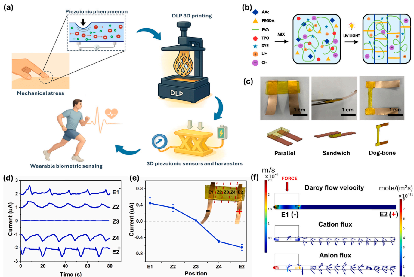
Fig. 1. Photocurable conductive hydrogel synthesis and piezoionic mechanisms. a) Schematic illustration of the exploitation of piezoionic phenomenon for fabricating 3D printed self-powered biometric sensors or energy harvesters. In the top of the image is represented the piezoionic effect in a polymeric material subjected to an external mechanical stimulus that produces an ionic displacement away from the deformation region and an ion flux measurable as an electrical response. b) Schematic of the preparation process of the ionic conductive hydrogel with a semi-interpenetrated network in an aqueous solution. c) Photopolymerized hydrogel flat samples with polyimide copper electrodes positioned in different configurations (parallel, sandwich and dog-bone) with their respective STL models. d) Current response of the hydrogel parallel sample to continuous deformations in 5 different zones of the device (curves were vertically shifted for clarity). e) Change in the polarity of the current output peaks according to the position of the stimulus. The inset shows the type of sample used during the test and the areas where the stimuli were applied. f) Simulated Darcy flow velocity (scale bar on the left) and related cation and anion fluxes (same scale bar on the right) in the hydrogel parallel sample shown in e) under the application of a force over the first electrode area (E1).
