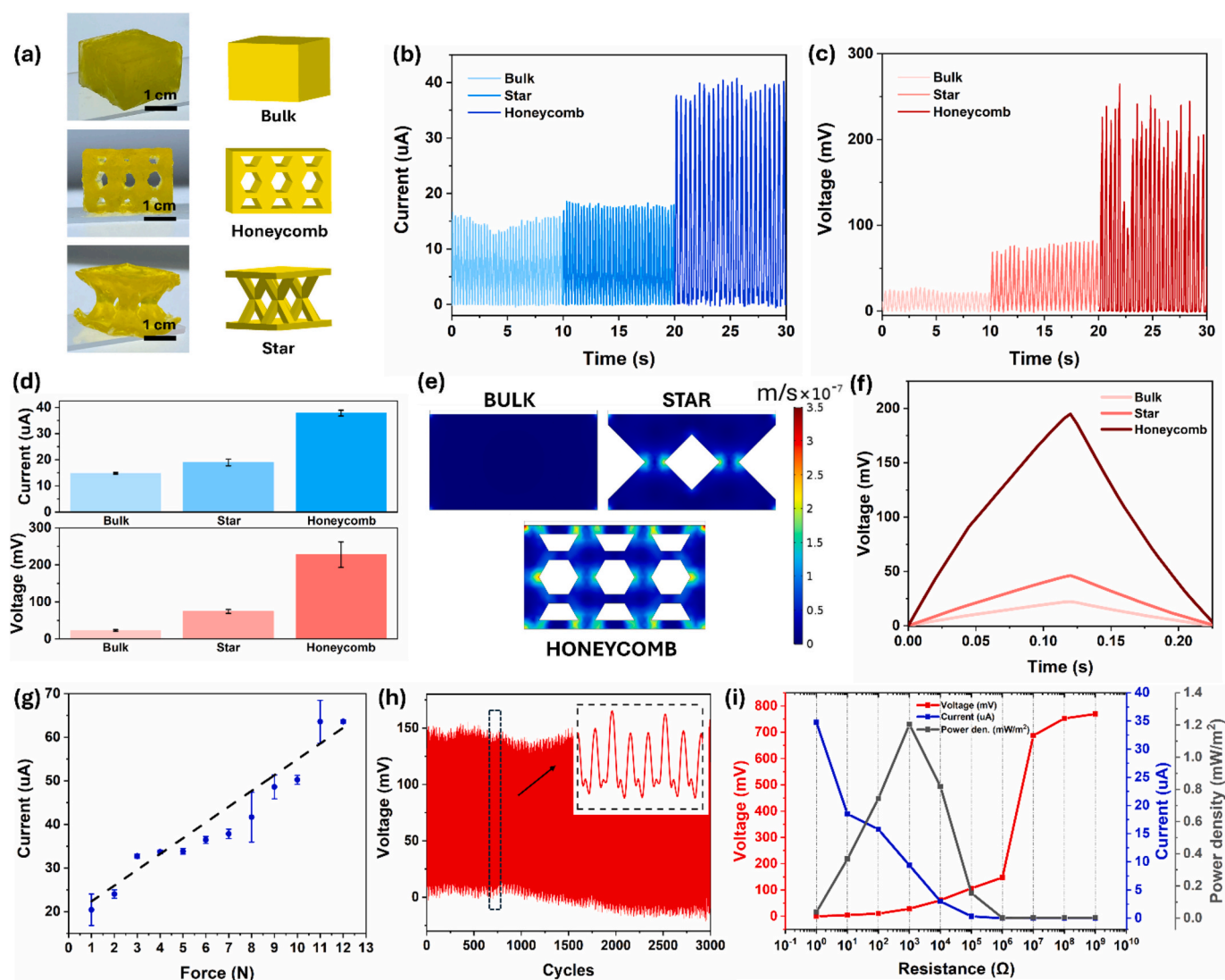
Fig. 4. 3D-printed piezoionic hydrogel pieces. a) Printed compression samples (bulk, honeycomb, stars) and their STL models. The samples have a thickness of 1 cm and an area of 1.5 cm 2 . b) Electrical current and c) voltage output of 3D specimens subjected to a cyclic compression test (frequency of 4 Hz and force of 10 N) and d) bar chart of the results. Error bars represent the standard deviation of peak values over 10 consecutive cycles. e) Simulated Darcy flow velocity in the 3D printed piezoionic samples under a force of 10 N. The color bar is the same for all the simulations. f) Simulated piezoionic voltage output under a compression with peak force of 10 N and frequency of 4 Hz. g) Evolution of the current output of a honeycomb 3D specimen as function of the force in a range from 1 N to 12 N. Error bars refer to the standard deviation of peak values over 10 consecutive cycles. h) Stability performance under mechanical loading of a honeycomb sample. The inset reports a zoom over some mechanical cycles. i) Impedance test results: output voltage, current, and electrical power density of a honeycomb piece under different load resistances in a range from 1 \Omega to 1 G \Omega .
