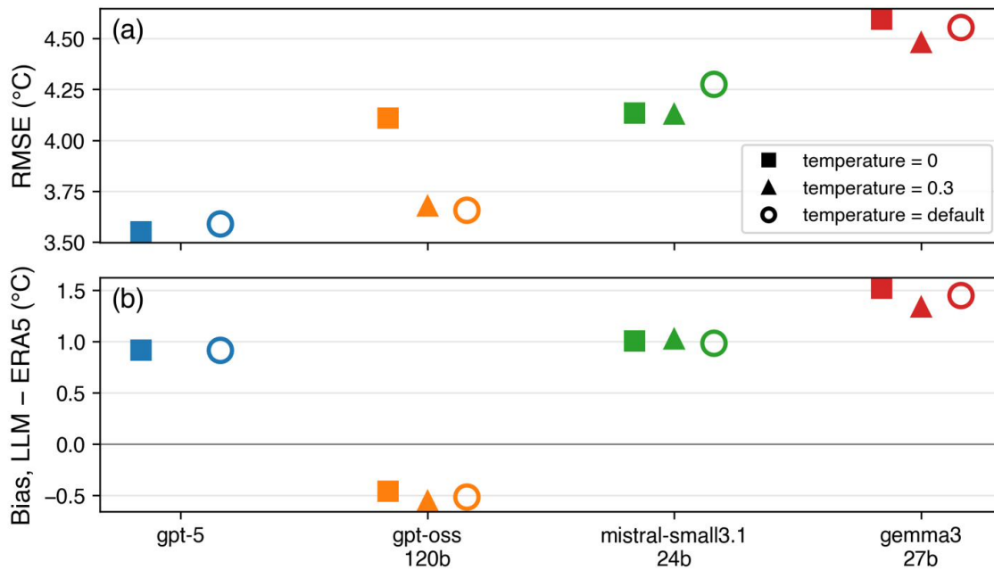
Fig. 6. Sensitivity of July temperature skill to the sampling-temperature setting at the 1,540-point subset. (a) RMSE and (b) mean bias (LLM minus ERA5) for July mean 2-m air temperature (1991-2020). Markers denote the sampling setting, where available: filled square, temperature = 0; filled triangle, temperature = 0.3; open circle, API default (sampling-temperature parameter left unset). Squares and triangles are the full-grid July runs restricted to the subset, and open circles are independent single-month July runs at the API default.
