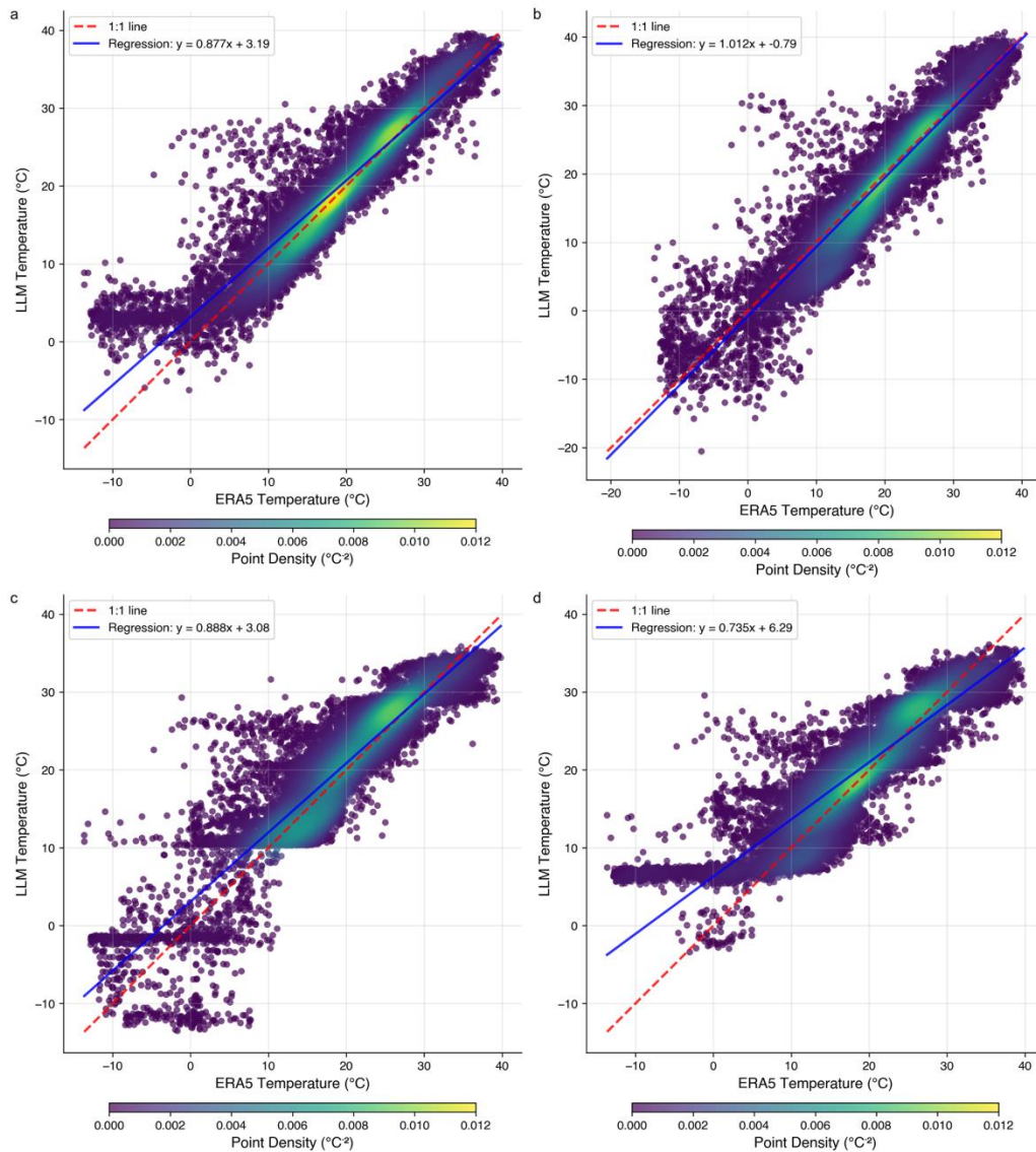
Fig. 4. Scatter plots of LLM-predicted versus ERA5 2-m air temperature (1991-2020). (a) GPT-5, (b) GPT-OSS 120B, (c) Mistral-small-3.1 24B, and (d) Gemma 27B. Point density was estimated using a Gaussian kernel density estimator with the default Scott bandwidth (Scott 2015).
