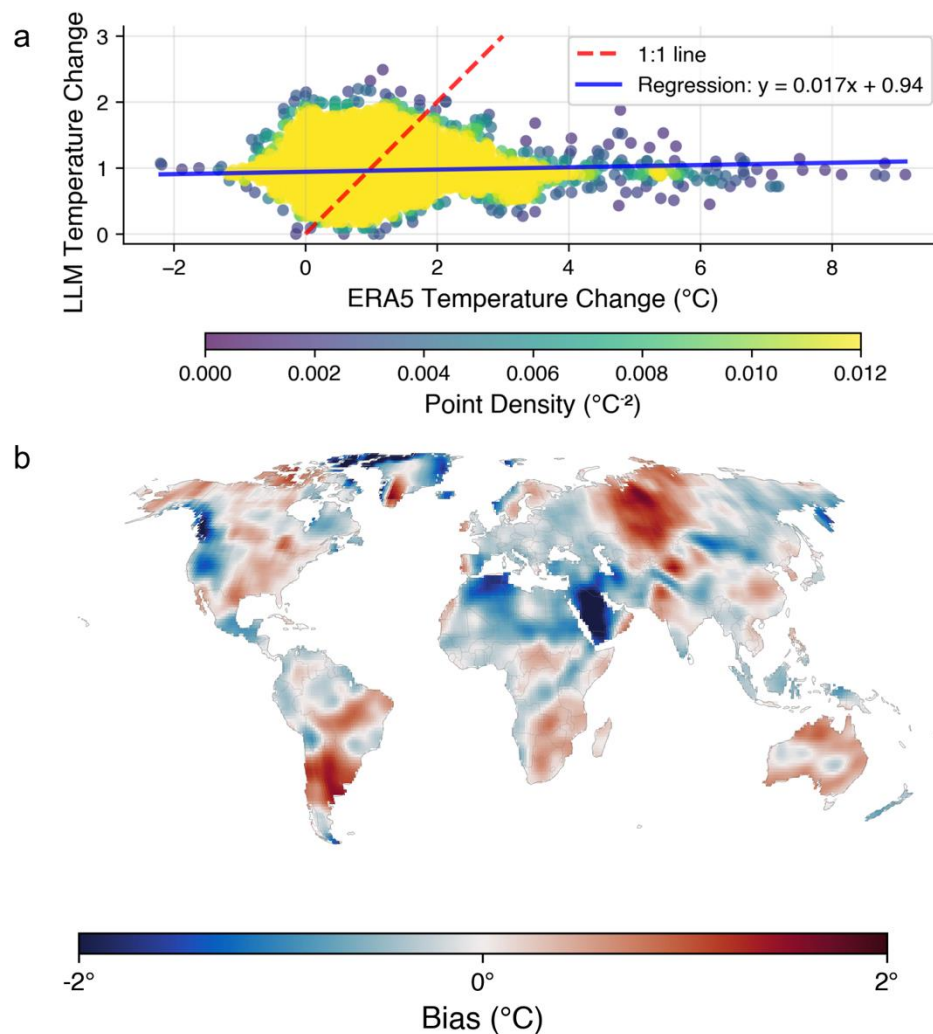
Fig. 7. GPT-5 predictions of temperature change between 1950-1974 and 2000-2024. (a) Scatter plot of LLM-predicted versus ERA5-derived change in mean July 2-m air temperature. (b) Spatial bias map (LLM minus ERA5). Simulation was run with sampling temperature 0.3. Bias calculated using a neighborhood (radius = 2) scheme (see Methods).
