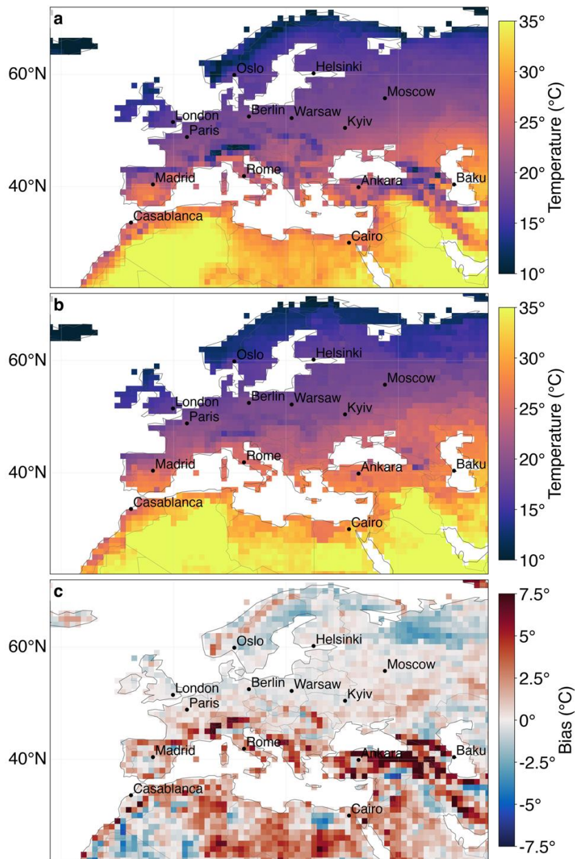
Fig. 2. Mean July 2-m air temperature (1991–2020). (a) ERA5 reanalysis. (b) LLM GPT-5 predictions. (c) Bias (GPT-5 minus ERA5). All panels are shown on a 1° grid.
