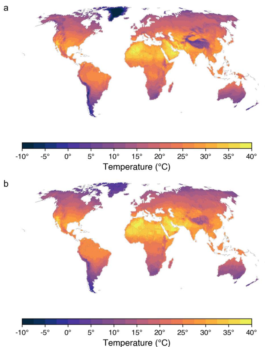
Fig. 1. Mean July 2-m air temperature (1991-2020). (a) ERA5 reanalysis. (b) LLM GPT-5 predictions. Both panels are shown on a 1° grid.
