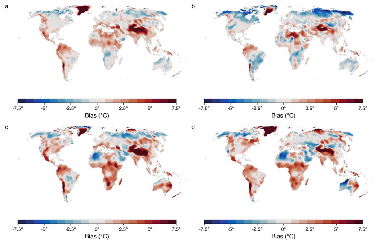
Fig. 3. Bias in mean July 2-m air temperature (1991-2020), defined as LLM predictions minus ERA5 reanalysis. (a) GPT-5, (b) GPT-OSS 120B, (c) Mistral-small-3.1 24B, and (d) Gemma 27B. All simulations were run with sampling temperature set to 0.3. Bias was calculated using a neighborhood (radius = 2) scheme (see Methods).
