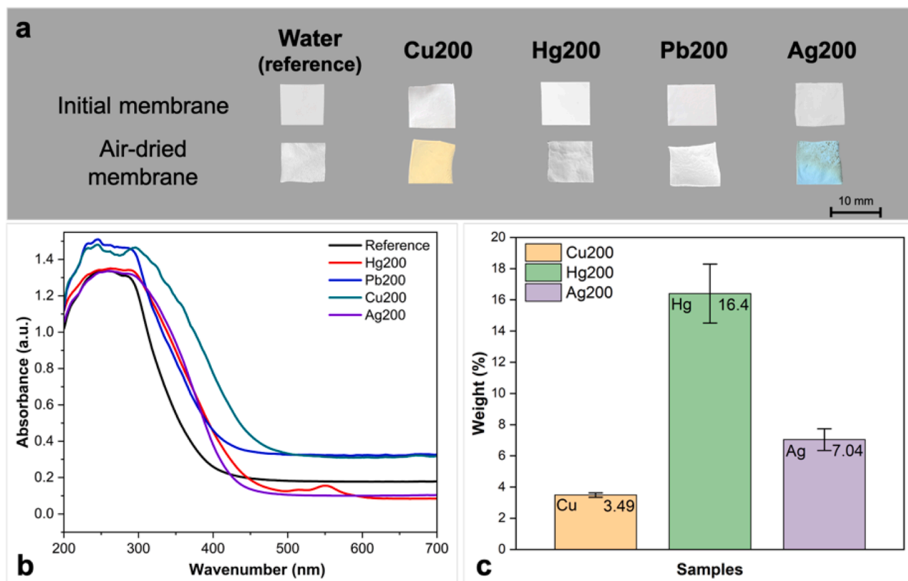
Fig. 6. Thiol-metal coordination of the thiol-functionalized ENMs. (a) Visual appearance of membranes after immersion in aqueous solutions of Cu(II), Hg(II), Pb(II) (concentration of 200 mg/L, pH 1) and subsequent air-drying for 1 day (except for the membrane exposed to Ag(I) solution, which was air-drying for 30 days). (b) Corresponding UV-Vis spectra of membranes after 1 day of air-drying, highlighting ion-dependent spectroscopic responses. (c) Quantitative elemental analysis of heavy metal uptake by the membranes determined by EDX after immersion in the respective metal ion solutions. Error bars represent the standard deviation of three independent experiments.
