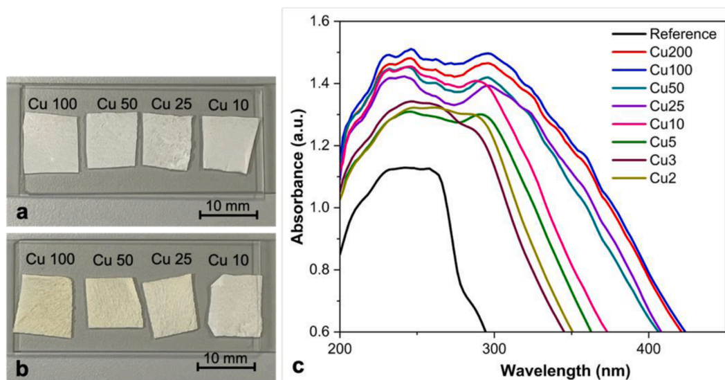
Fig. 7. Concentration-dependent response of thiol-functionalized ENMs toward Cu(II). Appearance of the membranes before (a) and after (b) exposure to the copper solution; (c) corresponding UV-Vis spectra of membranes immersed in Cu(II) solution at different concentrations under ambient conditions, compared to the membrane reference immersed in distilled water.
