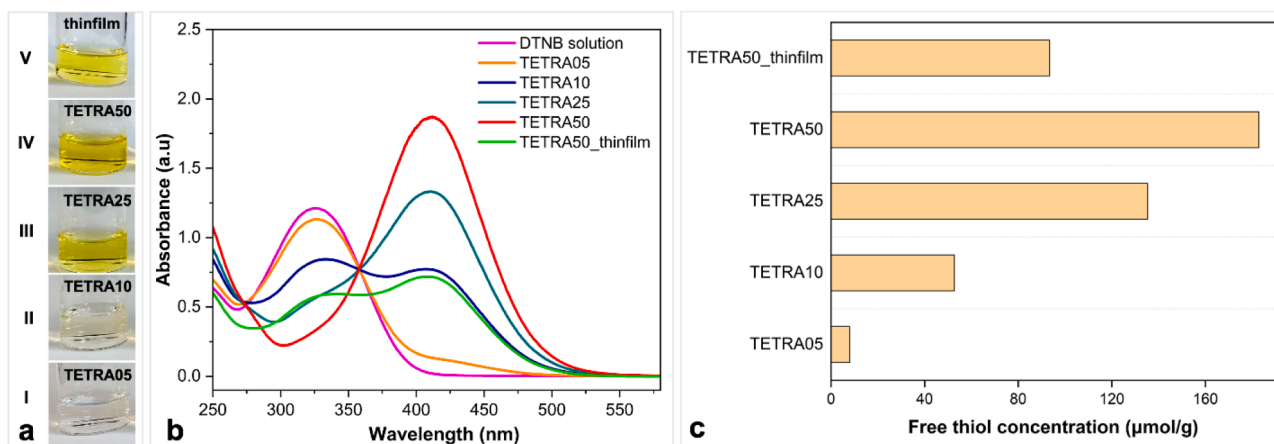
Fig. 5. Quantification of thiol functional group concentrations on the ENMs: (a) photographs of DTNB solution after immersing the functionalized membranes and thin-film (I: TETRA05; II: TETRA10; III: TETRA25; IV: TETRA 50; V: TETRA50_thinfil); (b) UV-Vis spectra of the DTNB solution prior and after membrane/thin-film immersion, showing the progressive increase of the 412 nm absorption peak, associated with TNB^{2-} , with the amount of the TETRA crosslinker in the electrospinning formulation; (c) free thiol concentration of the functionalized membranes and thin-film normalised by dried sample weight.
