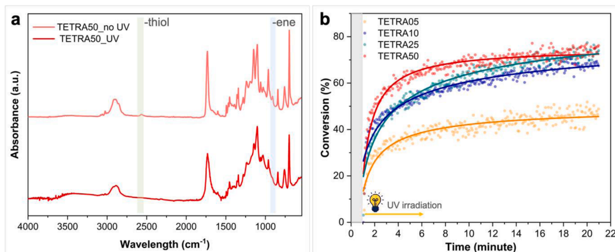
Fig. 2. (a) ATR-FTIR spectra of the membrane containing the highest amount of crosslinker (TETRA50) before (TETRA50_no UV) and after (TETRA50_UV) 20 min of irradiation. (b) Vinyl conversion percentage as a function of irradiation time for all formulations, as determined by real-time FTIR measurements.
