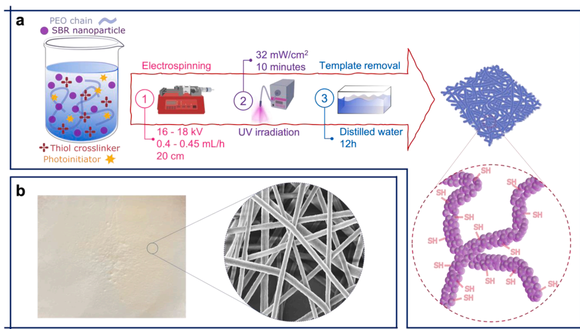
Fig. 1. (a) Schematic illustration of the fabrication procedure of the thiol-functionalized ENMs: (1) suspension electrospinning, (2) UV irradiation, and (3) template removal. (b) Optical photograph of the resulting membrane together with a representative FE-SEM image showing the nanofibrous structure.
