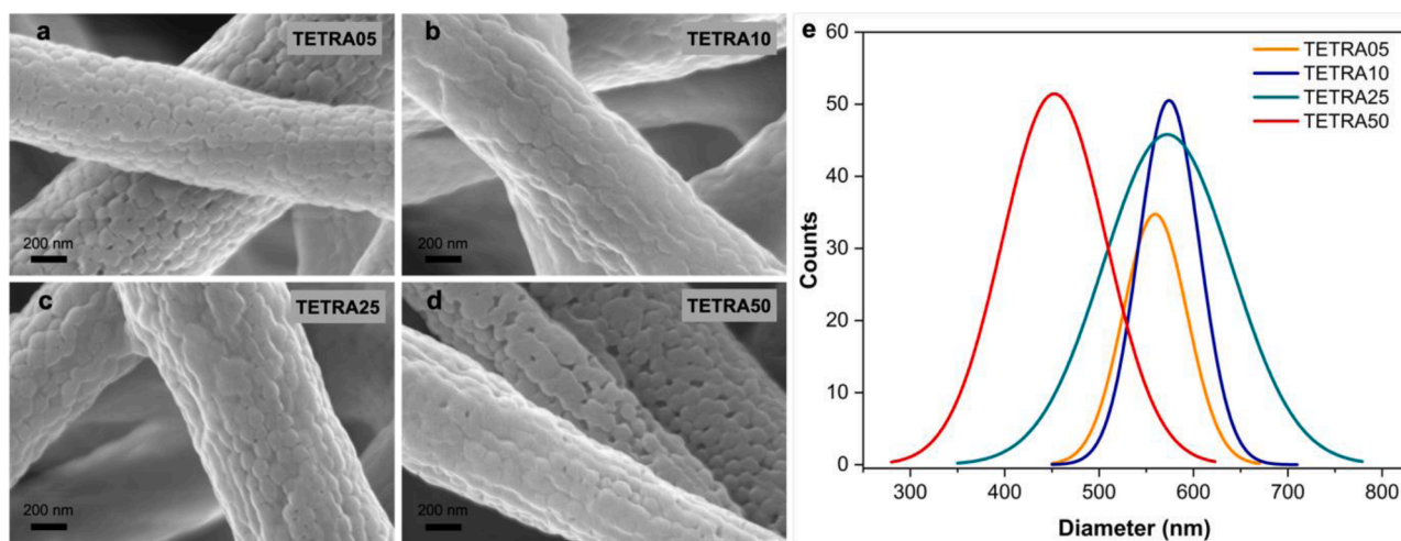
Fig. 3. Morphological analysis of the ENMs with different amounts of thiol crosslinker from 5 to 50 phr: FESEM images of (a) TETRA05, (b) TETRA10, (c) TETRA25, and (d) TETRA50; and (e) corresponding normalized average fiber diameter distributions.
