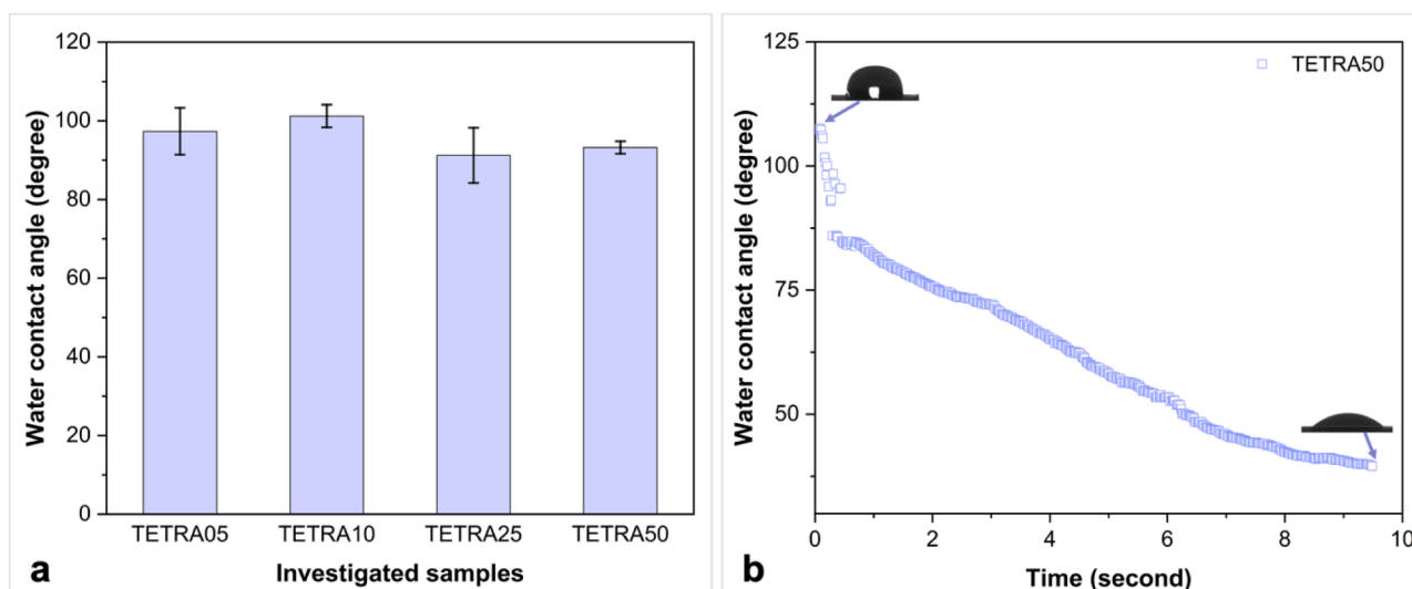
Fig. 4. Wettability of the thiol-functionalized ENMs: (a) water contact angle values of all investigated samples immediately after drop deposition, and (b) the evolution of water contact angle with time of the TETRA50 sample.
