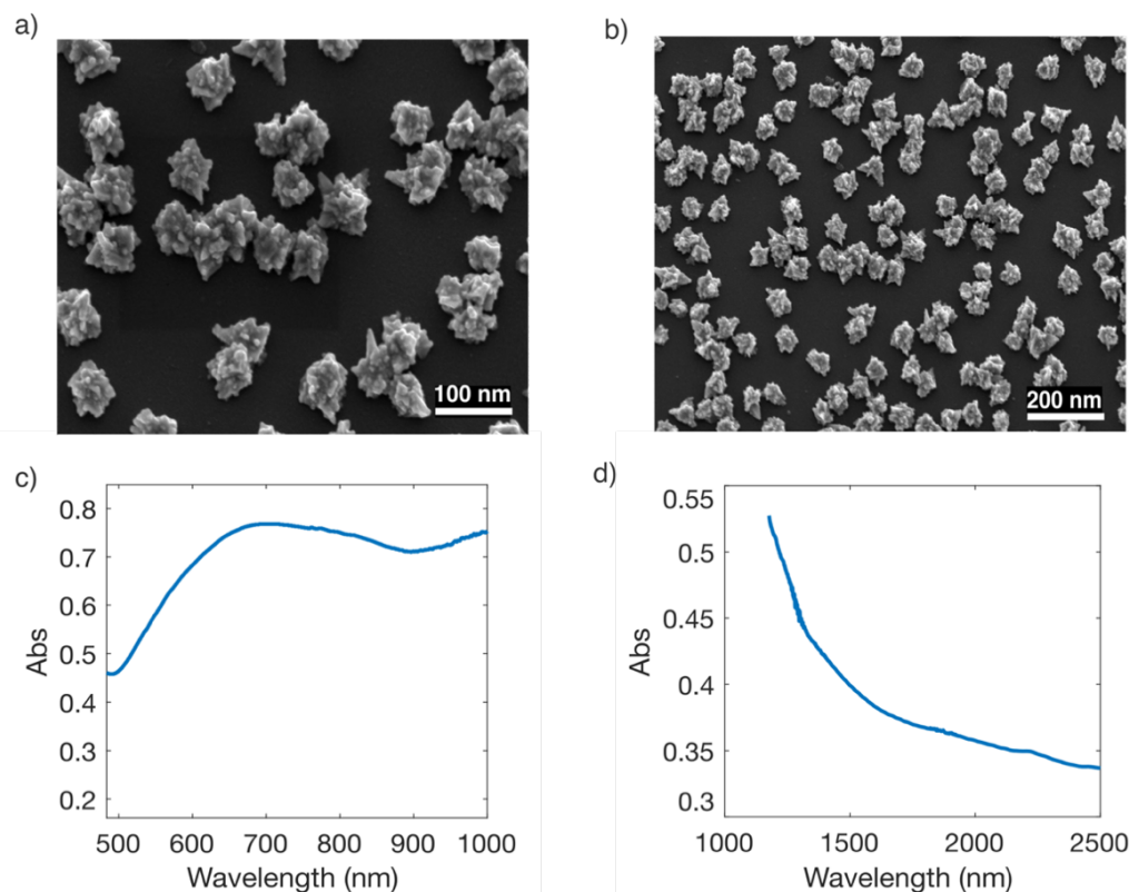
Fig. 2. (a) 50K, (b) 25K magnification SEM images of AuNSs deposited on the D-shaped fiber after 30 minutes of growth with different magnification. (c) UV-Vis-NIR (d) FTIR spectra of AuNSs grown on a flat glass
