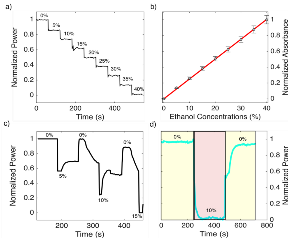
Fig. 3. (a) Sensorgram showing the D-shaped fiber transmitted power reduction for each ethanol concentration in time. (b) Calibration curve of the D-shaped fiber sensor for ethanol concentration ranging from 0% to 40 %. Recovery of the sensor after exposure to ethanol solution at a flow rate of c) 500 \mu\text{L}/\text{min} and of d) 1 \text{mL}/\text{min} .
