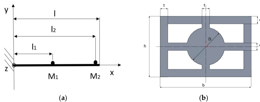
Figure 5. Cantilever beam: (a) System schematic representation; (b) Cross-section details.
