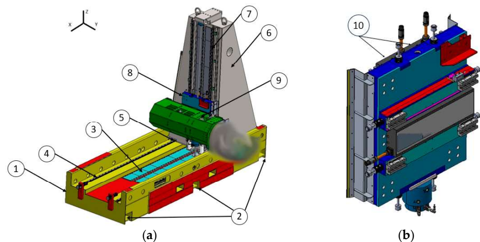
Figure 1. Cartesian robot prototype: (a) Overall machine; (b) Detail view of Z Carriage sub-assembly.
