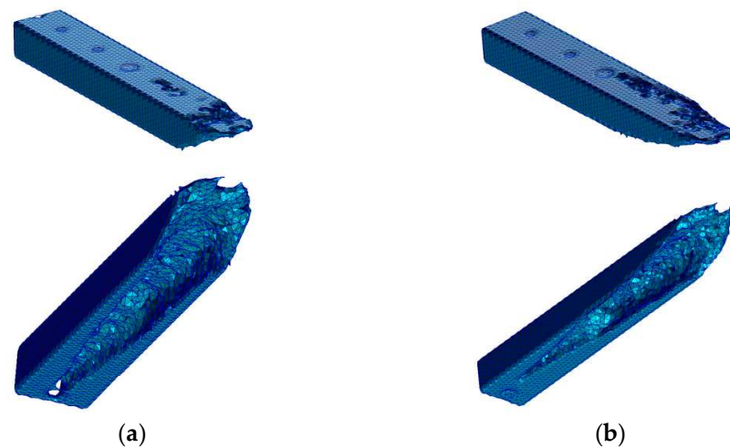
Figure 9. Topology optimization output: (a) ESL method; (b) QSL method.
