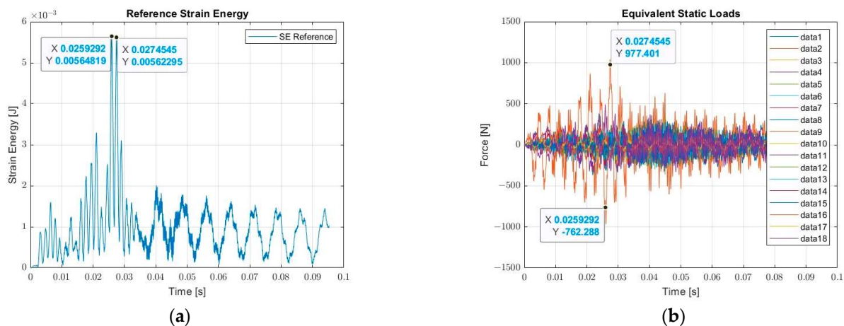
Figure 8. Transient analysis output: (a) Strain energy; (b) Equivalent Static Loads.
