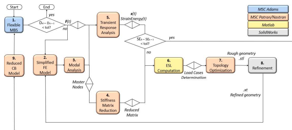
Figure 3. ESL method employed in the work.
