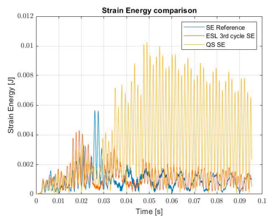
Figure 10. Strain energy comparison.
