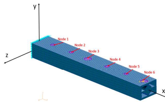
Figure 6. Beam finite element model.
