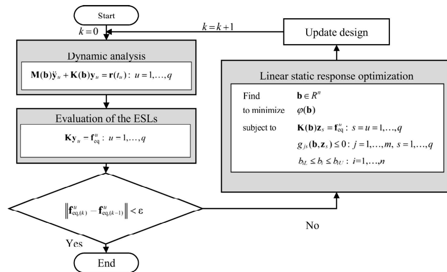
Figure 2. ESL method employed in the literature [15].
