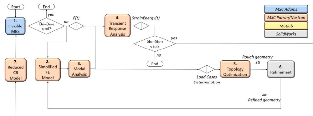
Figure 4. QSL method employed in the work.
