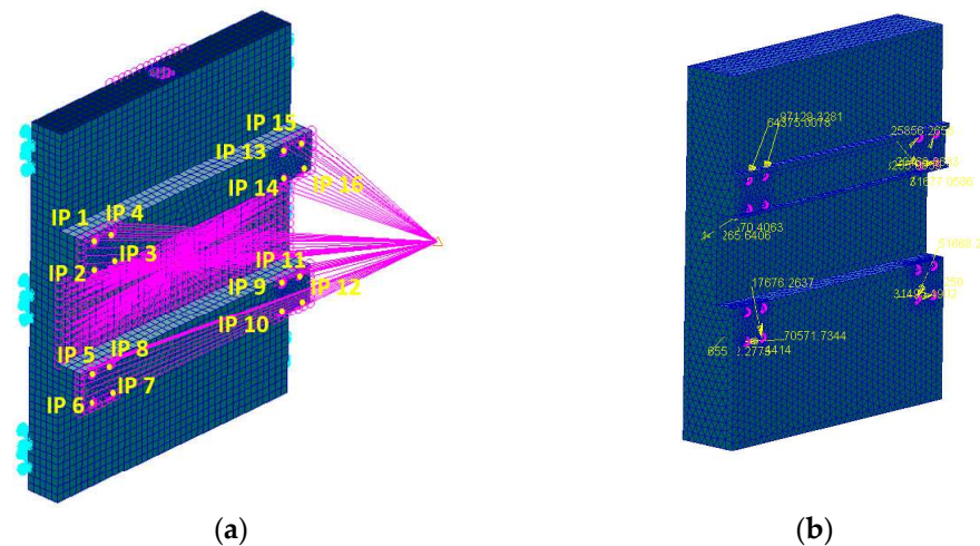
Figure 11. Z Carriage: (a) Finite Element model; (b) Design Volume.
