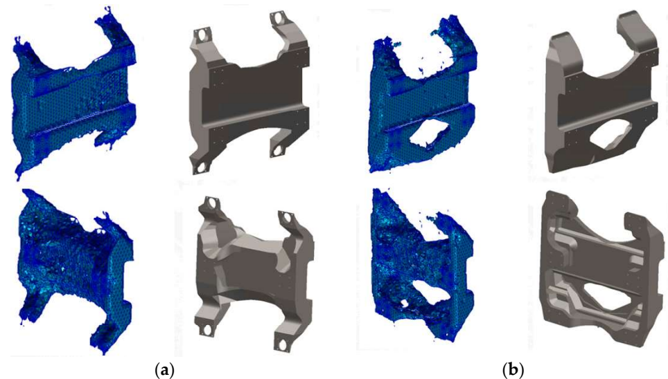
Figure 12. Z Carriage topology optimization output: (a) ESL method; (b) QSL method.
