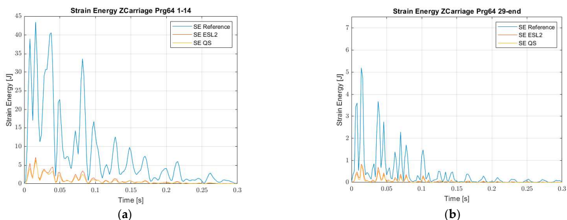
Figure 13. Z Carriage strain energies: (a) Trajectory Prg64 1–14; (b) Trajectory Prg64 29–end.
