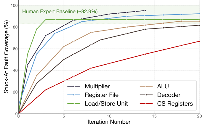
Fig. 3. Coverage across generation iterations. Regular datapaths improve rapidly, whereas control/state-dependent modules require sustained search.
