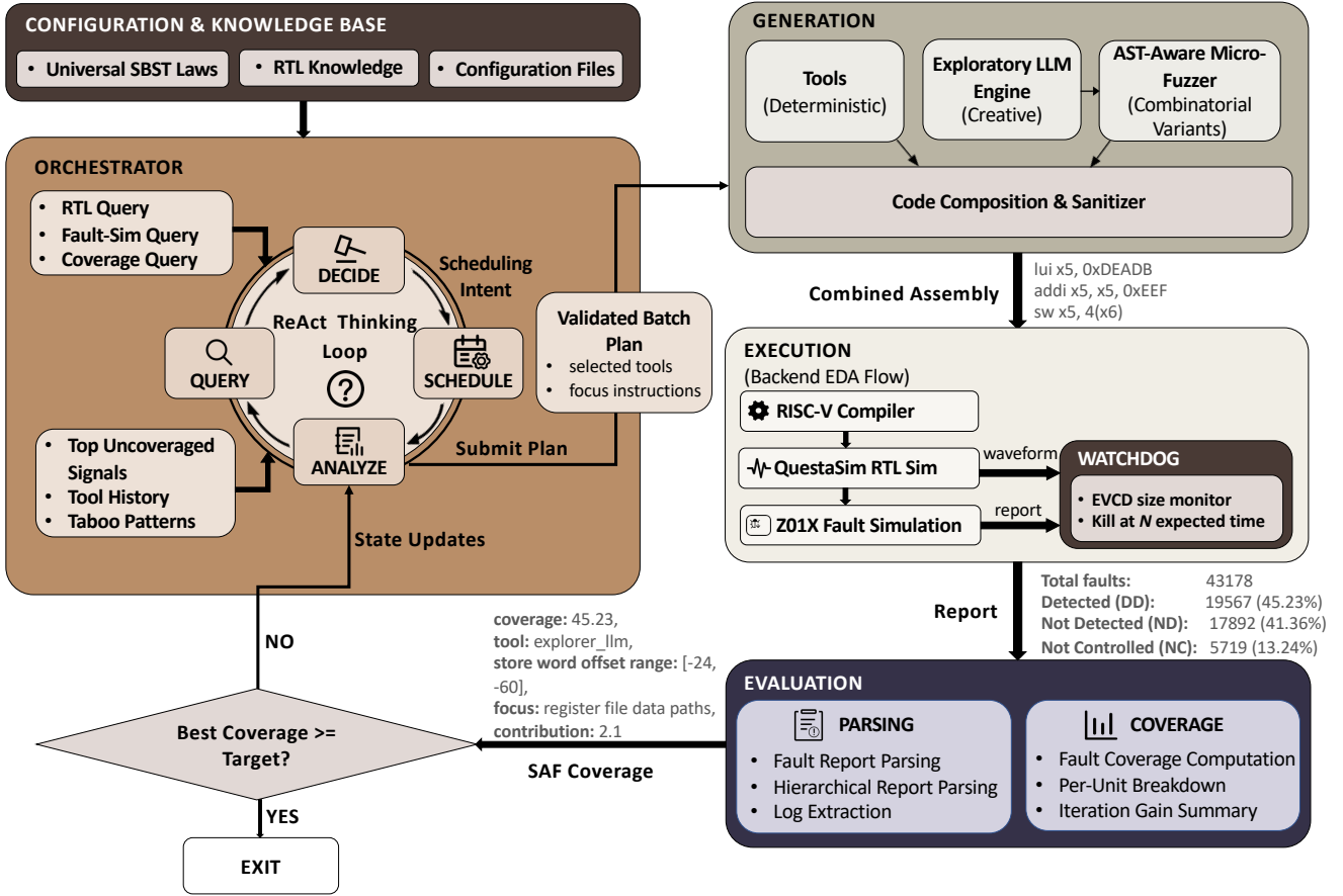
Fig. 1. Si-ATLAS closed loop. The Orchestrator turns compressed fault feedback into a validated batch plan. Deterministic templates, an exploratory LLM, and an AST-aware micro-fuzzer generate candidates; the Sanitizer and Watchdog bound their use in the backend toolchain.
