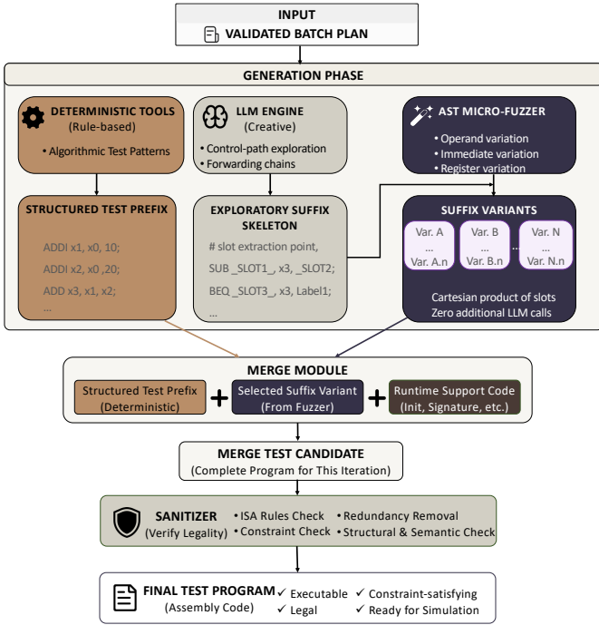
Fig. 2. Multi-engine synthesis: a deterministic prefix establishes legal state, the LLM proposes a structural skeleton, and the micro-fuzzer expands typed operand slots before sanitization.
