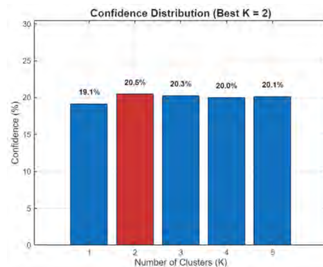
Figure 9. Distribution of confidence percentages associated with different values of the number of clusters k , calculated from the Gap Statistic via softmax normalization, on the entire dataset including male and female subjects. The column in red represents the selected k = 2 value, which produced a subdivision strongly consistent with the biological sex of the subjects.
