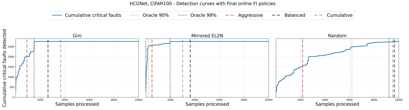
Fig. 2: Detection curves for HCGNet/CIFAR-100 under Gini, Mirrored EL2N, and random workload ordering. Informative rankings concentrate critical-fault discovery early, making dynamic stopping substantially more effective than under random ordering.
