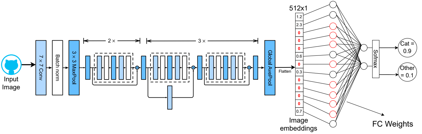
Fig. 2: Sparse ResNet18. Activation sparsity is computed in the penultimate layer, representing the feature embeddings extracted by the network, and not in the network weights. Inactive neurons (red circles) correspond to zero-valued activations that do not contribute to the output.
