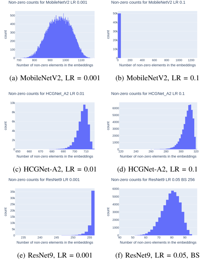
Fig. 3: Panels (a)–(f) show distributions of non-zero activations for increasing learning rates. Higher learning rates yield progressively sparser feature embeddings, suppressing non-relevant feature channels. This confirms that training dynamics can implicitly drive activation sparsity, yielding sparse activation patterns correlated with higher fault masking.
