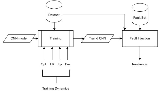
Fig. 1: Overview of the proposed implicit sparsity framework.
