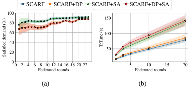
Fig. 4: Evaluation of the benchmarks in terms of (a) satisfied demand and (b) training time. Despite additional training time, SCARF+DP+SA maintains a strong 88% satisfied demand, securely building a robust and generalizable model.
