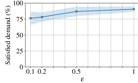
Fig. 3: Satisfied demand achieved by when varying \epsilon values. \epsilon = 1 offers a reasonable privacy-performance trade-off.
