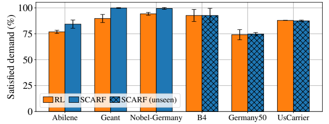
Fig. 2: Percentage of satisfied demand. SCARF outperforms RL in topologies seen during training, and achieves comparable performance when employed in unseen topologies.
