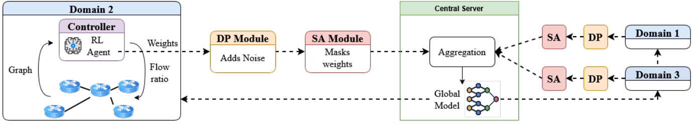
Fig. 1: Overall SCARF learning process. ISPs can collaborate for network management while keeping their data private.
